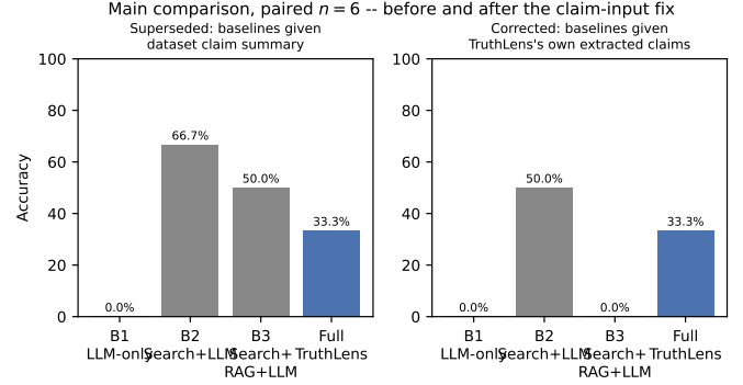
Fig. 3. Table V plotted, superseded vs. corrected. The reversal is concentrated in items where baselines had been implicitly handed a claim to reason about that TruthLens itself never produced.
