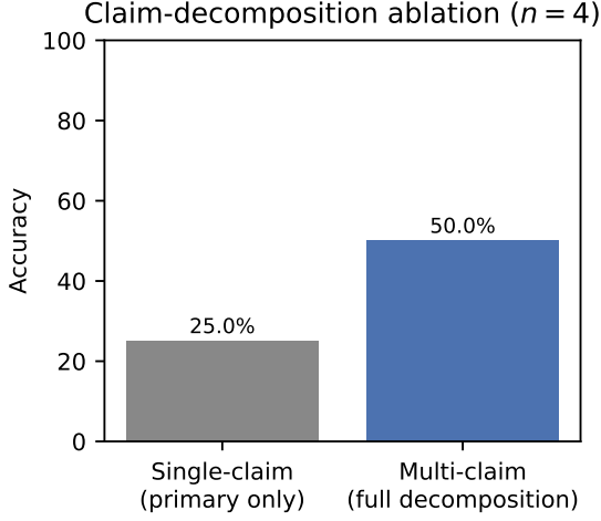
Fig. 4. Table VI plotted. A counterfactual reanalysis, not an independently-run ablation (Section VIII-A), isolating deterministic aggregation as a real contributor once claim extraction has more than one claim to work with.
