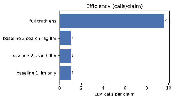
Fig. 8. LLM calls per claim by configuration (research/system_efficiency.csv). Full TruthLens’s call count is derived from real average sources/claim, not directly measured end-to-end; latency is not shown, a disclosed gap (text).
