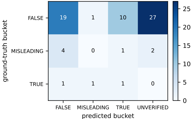
Confusion matrix (resolved items)
