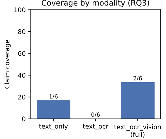
Fig. 7. Table XI plotted. text_ocr scoring below text_only is reported as a real result, not suppressed (Section X explains the likely cause).
