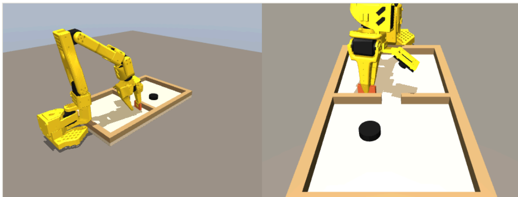
MuJoCo scene: SO-101 holding the paddle at the gate (side and gate cameras).
