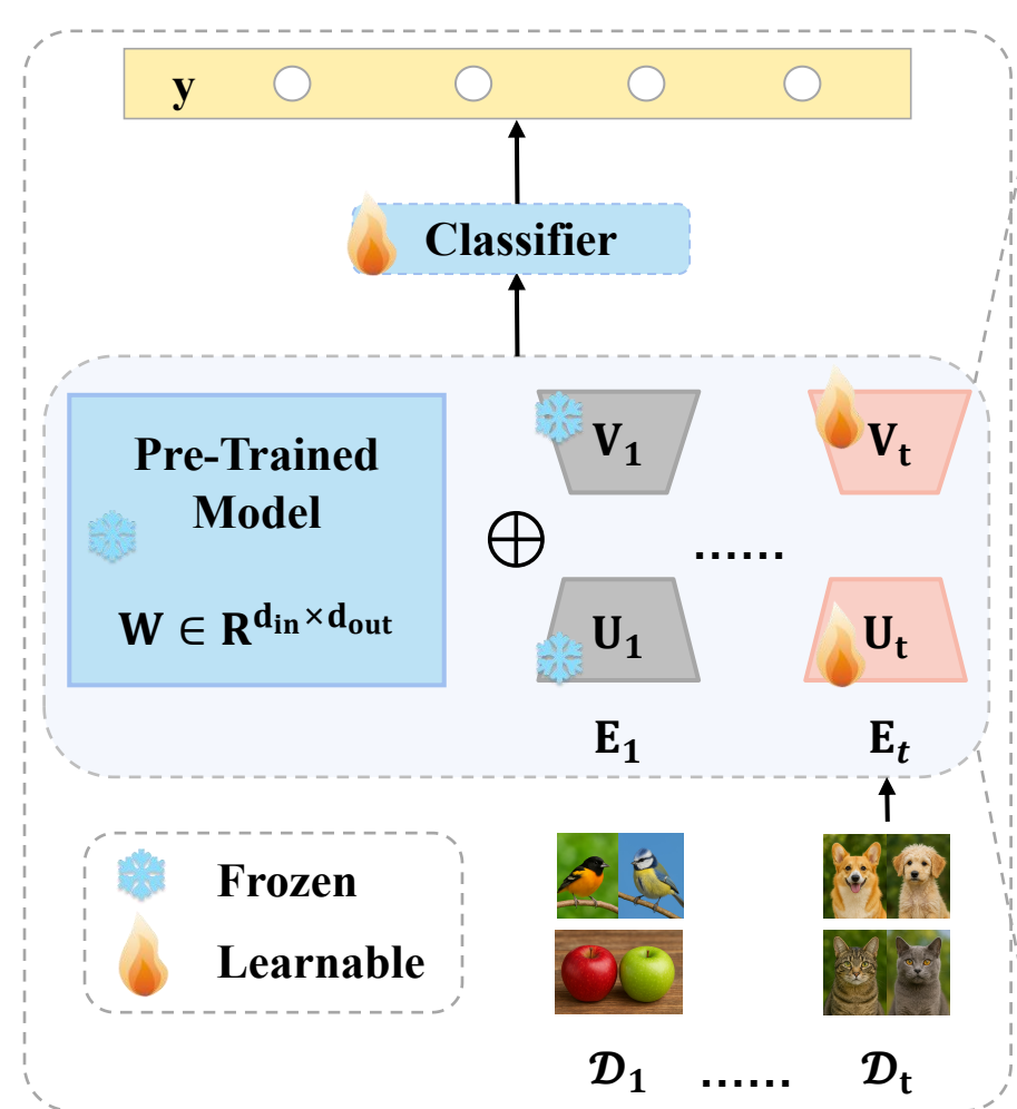
(a) LoRA-Expert Training
