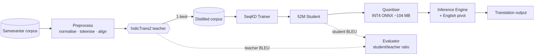
Figure 3.5: Level-1 data flow diagram: corpus to deployed translation
