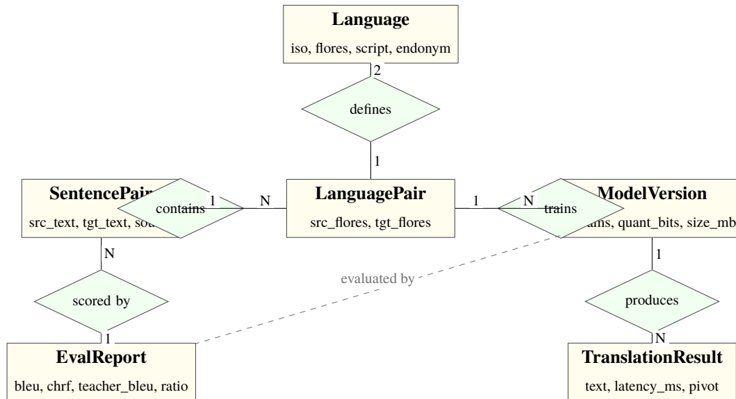
Figure 3.6: Entity-relationship model of SETU’s persistent artifacts
