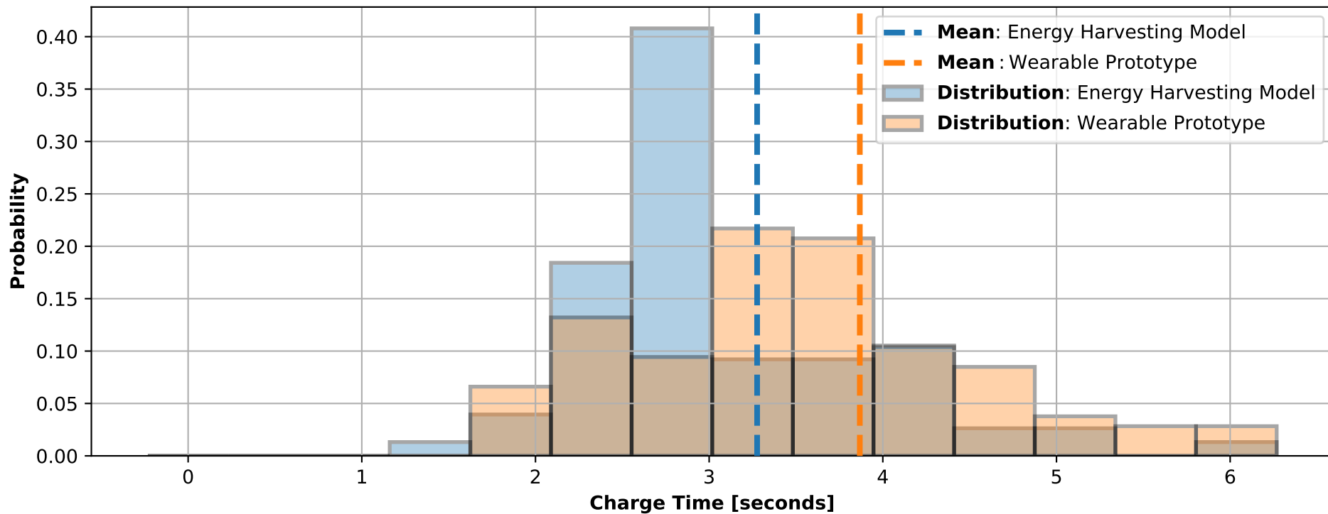
Distribution of Charge Times for Walking (Sensor on Arm )
