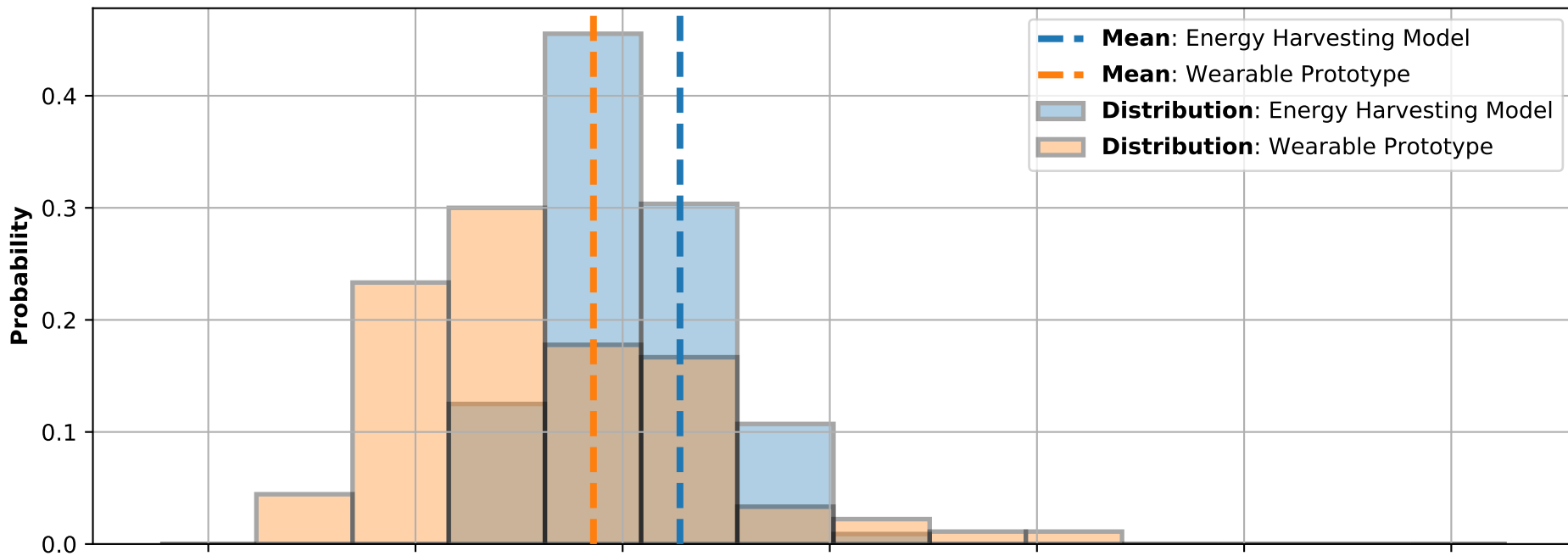
Distribution of Charge Times for Walking (Sensor on Arm )
