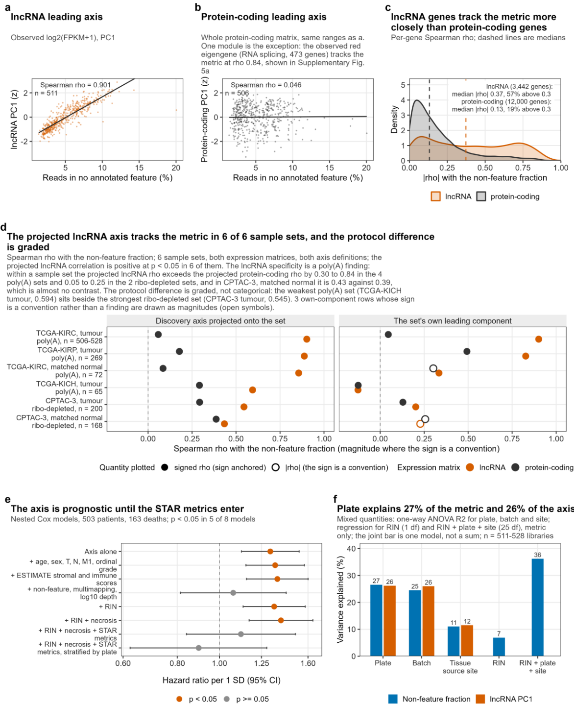
Fig. 2 | The leading IncRNA expression axis tracks non-exonic read content. a First principal component of the observed IncRNA matrix, log2(FPKM + 1), against the non-feature read fraction per library, with a least-squares fit (Spearman rho 0.90, n = 511). b As a for the protein-
