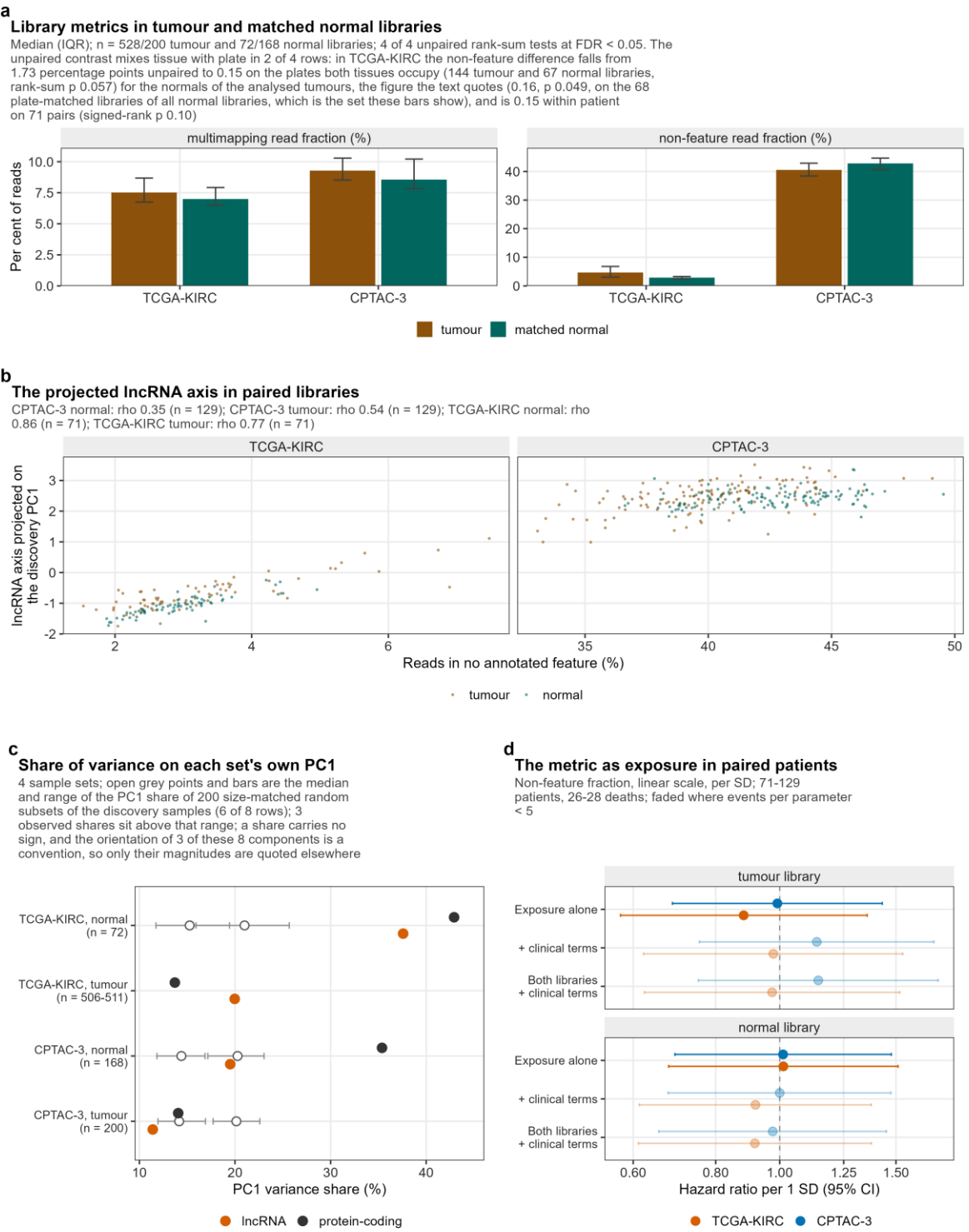
50 a Median and interquartile range of the multimapping and non-feature fractions in tumour and 51 matched normal libraries of TCGA-KIRC and CPTAC-3. b Projected lncRNA axis (the
