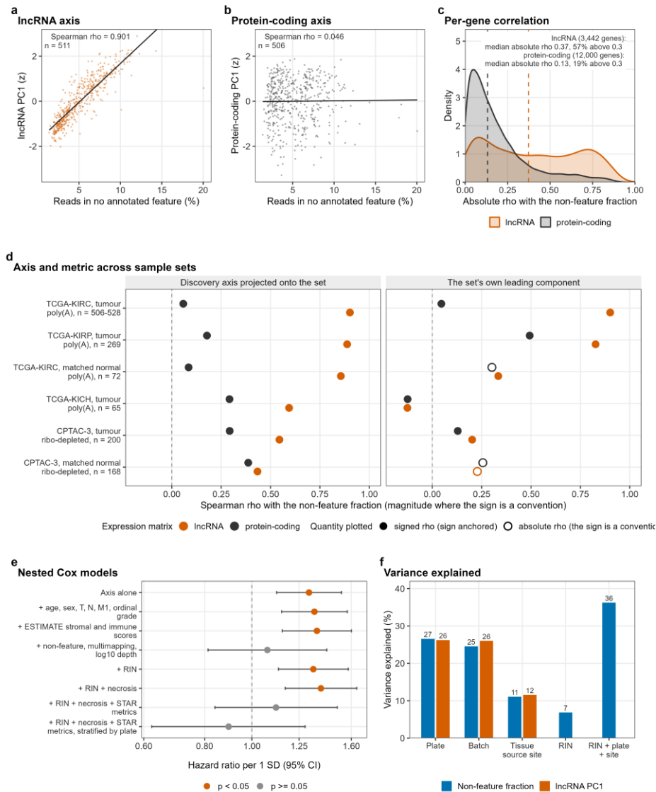
Fig. 2. The leading lncRNA expression axis tracks non-exonic read content. a First principal component of the observed lncRNA matrix, \log_2(\text{FPKM} + 1) , against the non-feature read fraction per library, with a least-squares fit (Spearman rho 0.90, n = 511 ). b As a for the protein-coding matrix, on identical axes (rho 0.05, n = 506 ). The observed protein-coding red eigengene (473 genes, RNA splicing) does track the metric (rho 0.84, Supplementary Fig. 5a). c Densities of per-gene absolute Spearman correlation with the metric. Dashed medians are 0.37 for 3,442 lncRNAs (56.8% above 0.3) and 0.13 for 12,000 protein-coding genes (18.8%). d Spearman correlation of the axis with the metric in six sample sets, faceted by the projected discovery axis and each set's own leading component. Open symbols, plotted as magnitudes, mark the 3 of 12 own-component rows whose sign cannot be fixed because its correlations with mean expression and the projected axis are weak or disagree. The projected lncRNA axis gives rho 0.90, 0.89, 0.86, 0.59, 0.55 and 0.43 in TCGA-KIRC tumours ( n = 528 ), TCGA-KIRP (269), TCGA-KIRC normal kidney (72), TCGA-KICH (65), CPTAC-3 tumours (200) and CPTAC-3 normal tissue (168). Within each set the projected lncRNA correlation exceeds the projected protein-coding correlation by 0.30 to 0.84 in the four poly(A) sets and by 0.05 to 0.25 in the two ribo-depleted sets. e Hazard ratio per standard deviation of the lncRNA axis under eight nested Cox models (503 patients, 163 events), with 95% confidence intervals on a logarithmic axis. Red marks p < 0.05 . The hazard ratio is 1.31 to 1.39 before the three STAR metrics enter and 1.08 after. It is 1.12 with RNA integrity and slide necrosis added to the STAR metrics, and 0.90 with plate stratification. f Variance in the metric and the axis explained by plate (26.6% and 26.2%), batch (24.6% and 26.0%) and tissue source site (11.1% and 11.6%), as one-way analysis of variance R-squared on 511 to 528 libraries. Two further bars, for the metric only, give regression R-squared on the 527 patients with an integrity number, for RNA integrity alone (6.9%, 1 degree of freedom) and for RNA integrity with plate and site (36.2%, 25 degrees of freedom). The joint bar comes from a single model, so it need not equal the sum of the other bars.
