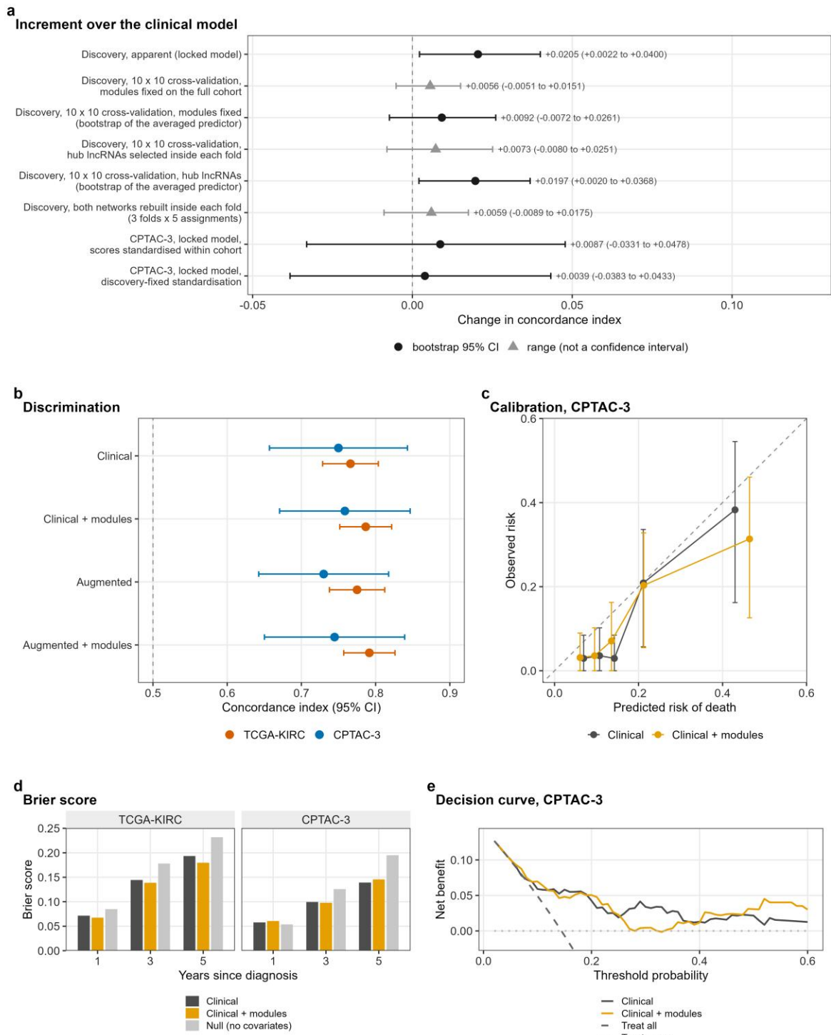
Fig. 7. Module eigengenes add no demonstrable discrimination over the clinical model. All panels are for overall survival. The clinical model is age, sex, T category, nodal status, M1 and ordinal grade. The augmented model adds the ESTIMATE stromal and immune scores and the
