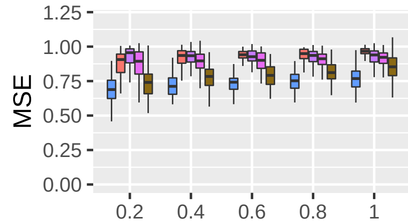
Threshold within Genes
