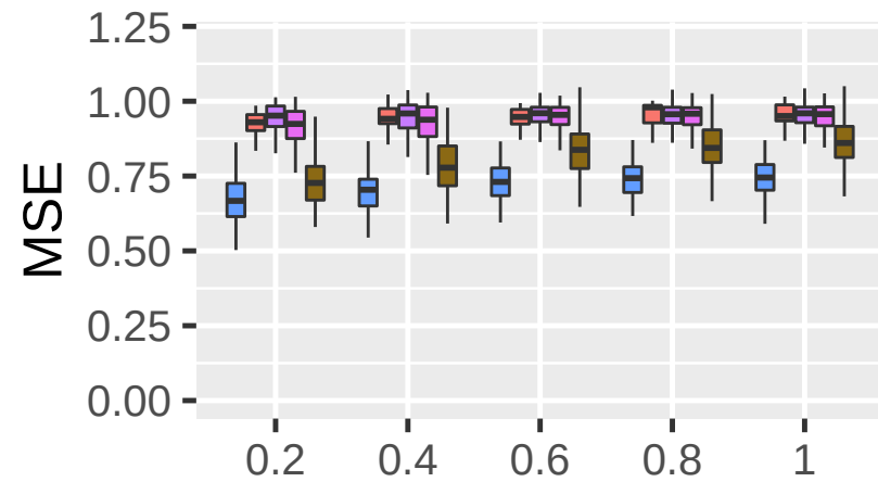
Multiplicative within Genes
