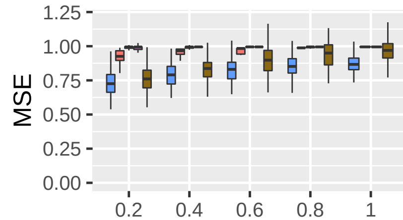
Multiplicative between Genes
