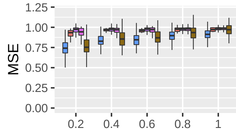
Threshold between Genes
