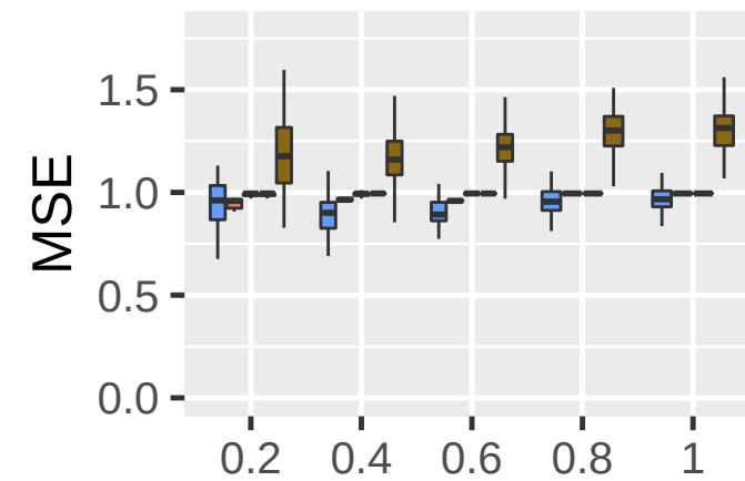
Rickercurve
