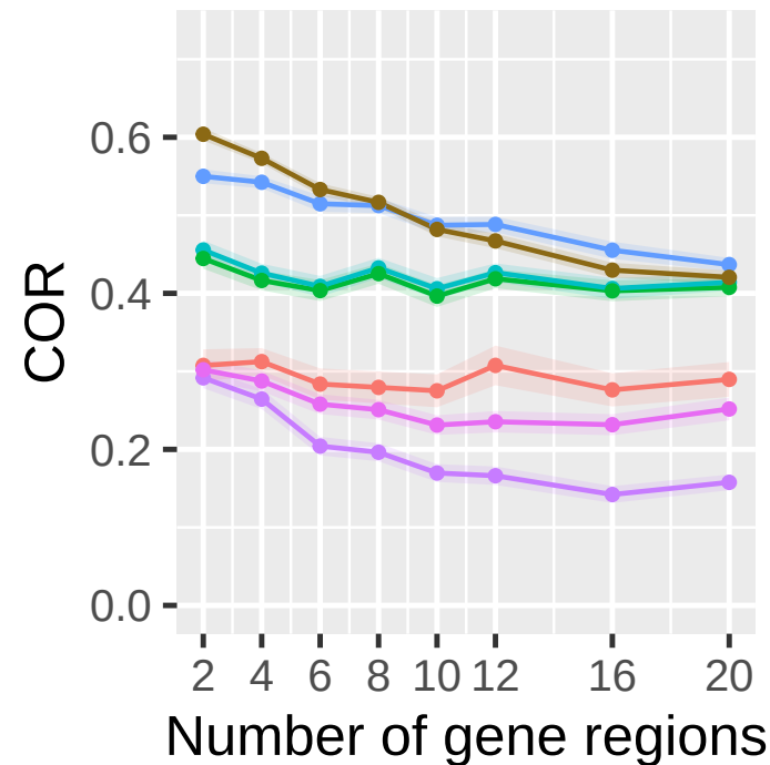
Threshold between Genes
