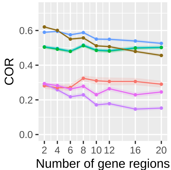
Multiplicative within Genes
