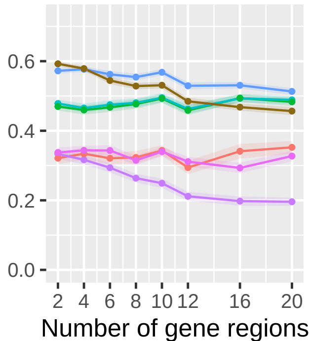
Threshold within Genes
