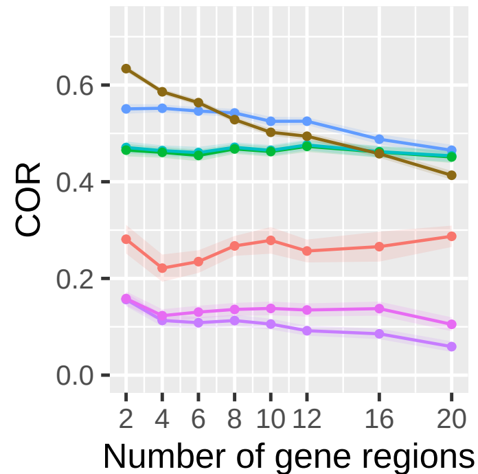
Multiplicative between Genes
