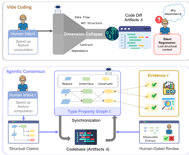
Figure 1: Vibe coding (top) treats natural-language prompts as the primary interface and produces code directly, with no persistent structure linking intent to artifacts. Agentic Consensus (bottom) introduces an explicit consensus layer C that mediates between human intent and executable artifacts, maintaining structural traceability and evidence-linked validation throughout the workflow.
