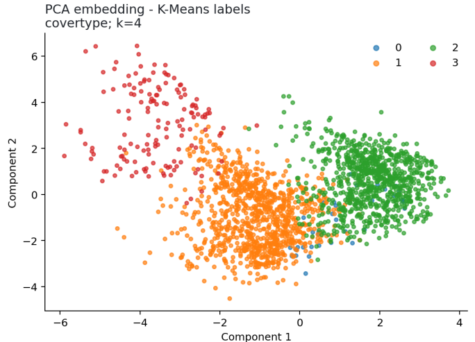
Fig. 4. Covertypes PCA view colored by k = 4 K-Means assignments; geometry is descriptive and does not claim recovery of seven classes.
