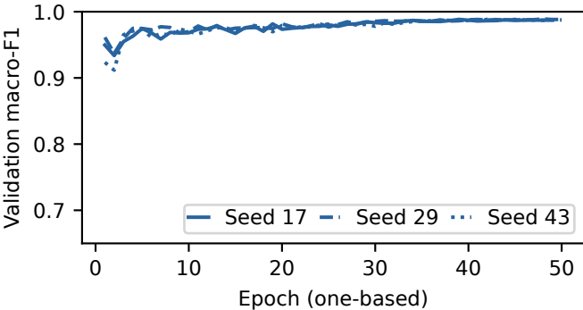
ResNet-50
