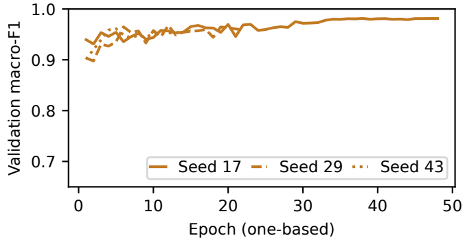
ViT-Small/16
