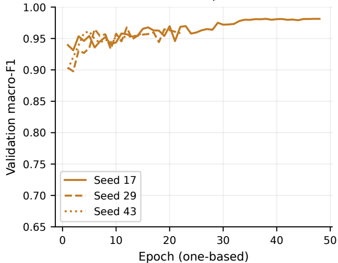
ViT-Small/16
