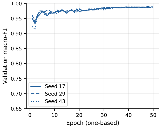
ResNet-50
