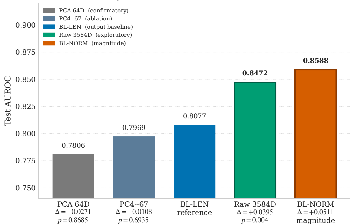
Paired Layer-16 comparison on the 98-prompt test set
