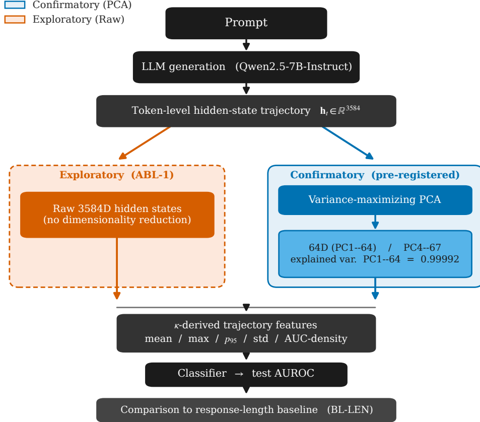
Experimental pipeline: confirmatory PCA vs. exploratory raw trajectories
