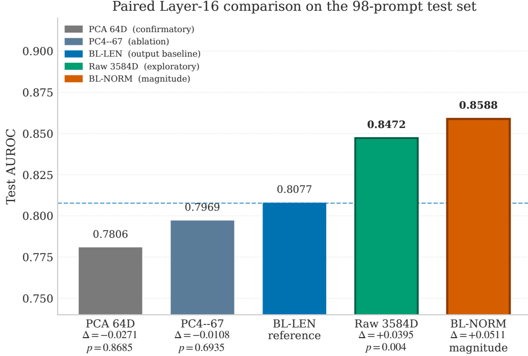
Figure 3: Paired Layer 16 test AUROC on the 98-prompt set: PCA 64D (0.7806), PC4-67 (0.7969), BL-LEN (0.8077), raw 3584D (0.8472), and BL-NORM (0.8588). BL-NORM and PC4-67 are reported in full. Raw vs. BL-LEN is exploratory ( p = 0.004 ).
