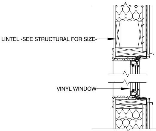
A04-02. 5- VINYL WINDOW DETAILS
