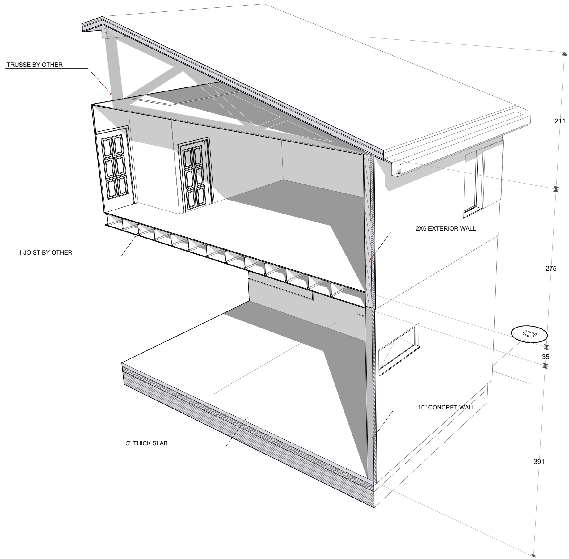
A04-01. 1- 3D SECTION
