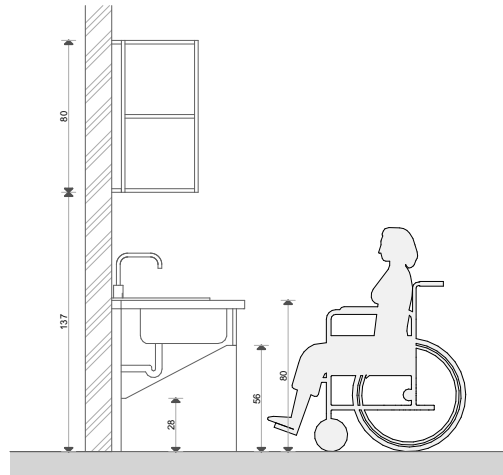
A04-03. 1- B.F SINK DETAILS
