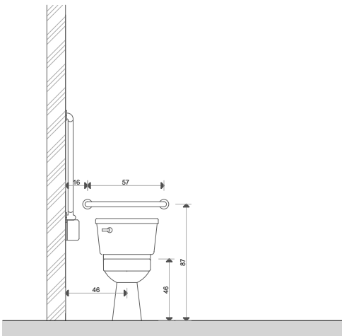
A04-03. 3- B.F WASHROOM FIXTURE
