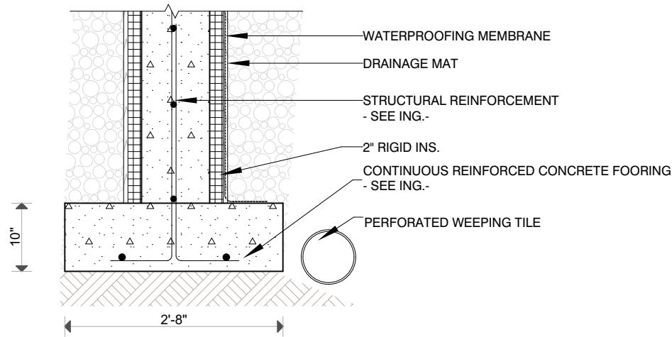
A04-02. 1- FOUNDATION FOOTING SECTION
