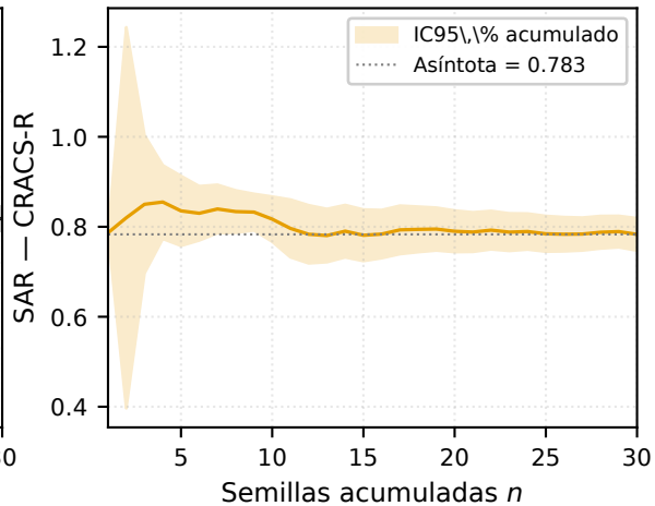
(b) E6\_burst, K = 300
