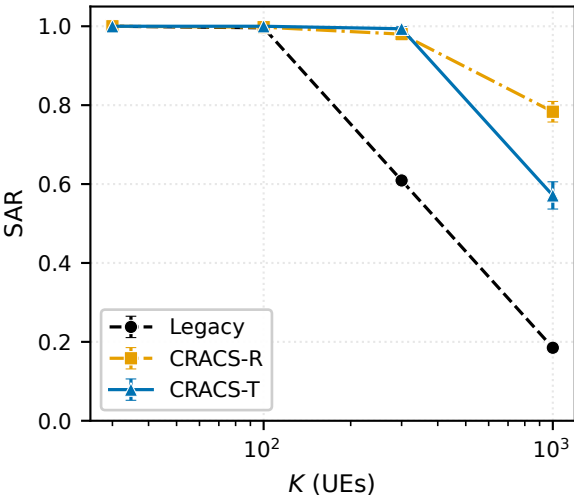
(a) Poisson (TM1), T = 60 s
