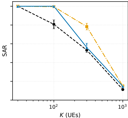
(b) Beta(3,4) (TM2), T = 10 s
