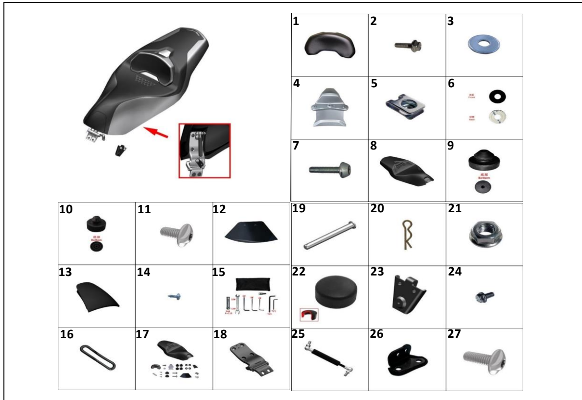
F-13 SEAT CHUSION ASSEMBLY
