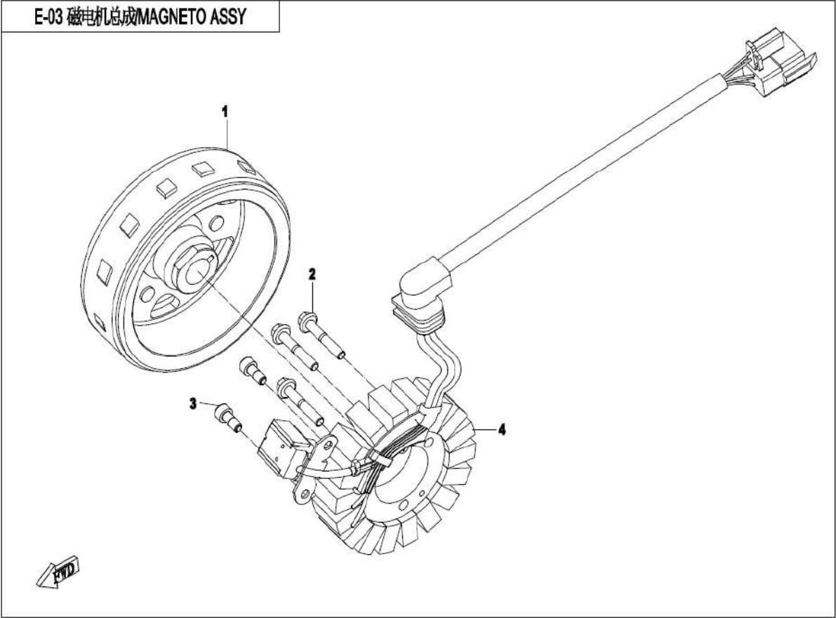
E03 MAGNETO ASSY.
