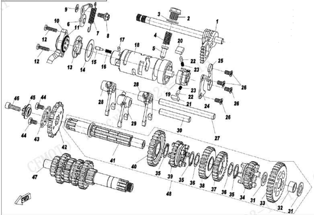
E06 TRANSMISSION ASSY.
