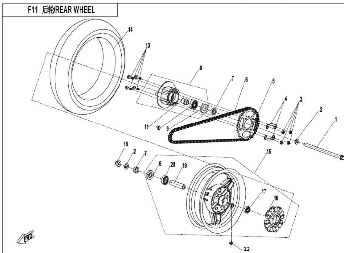
F11 REAR WHEEL
