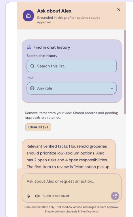
Current app · grounded answer, evidence, and voice controls
