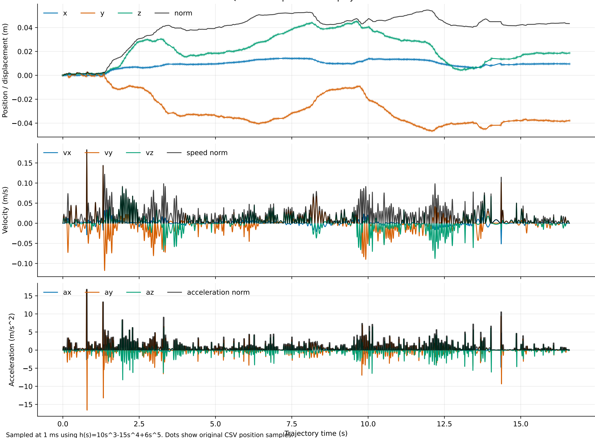
Quintic interpolation of replay translation
