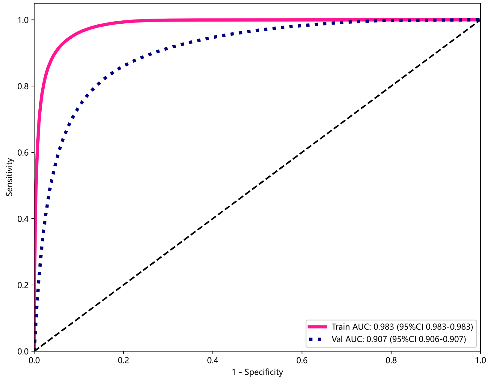
Model: resnet50
