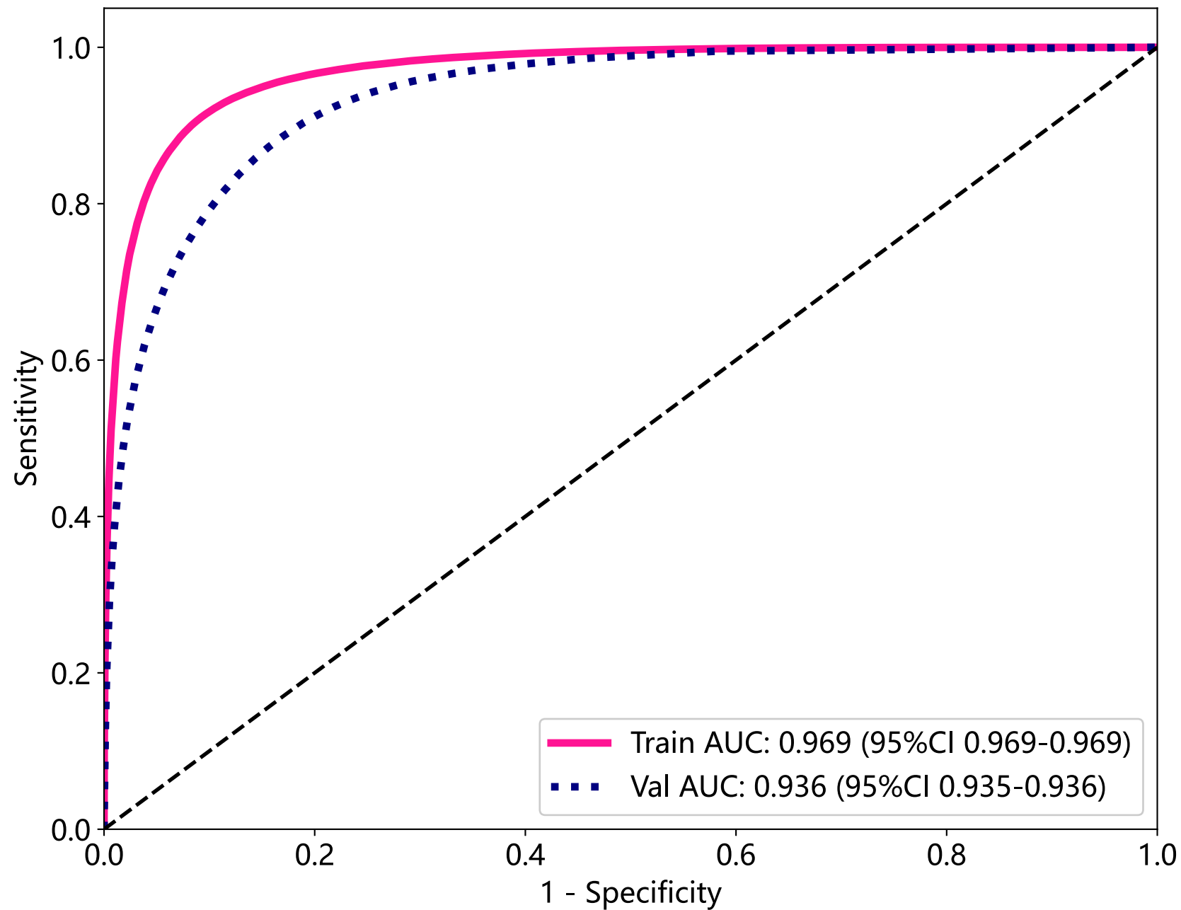
Model: resnet50
