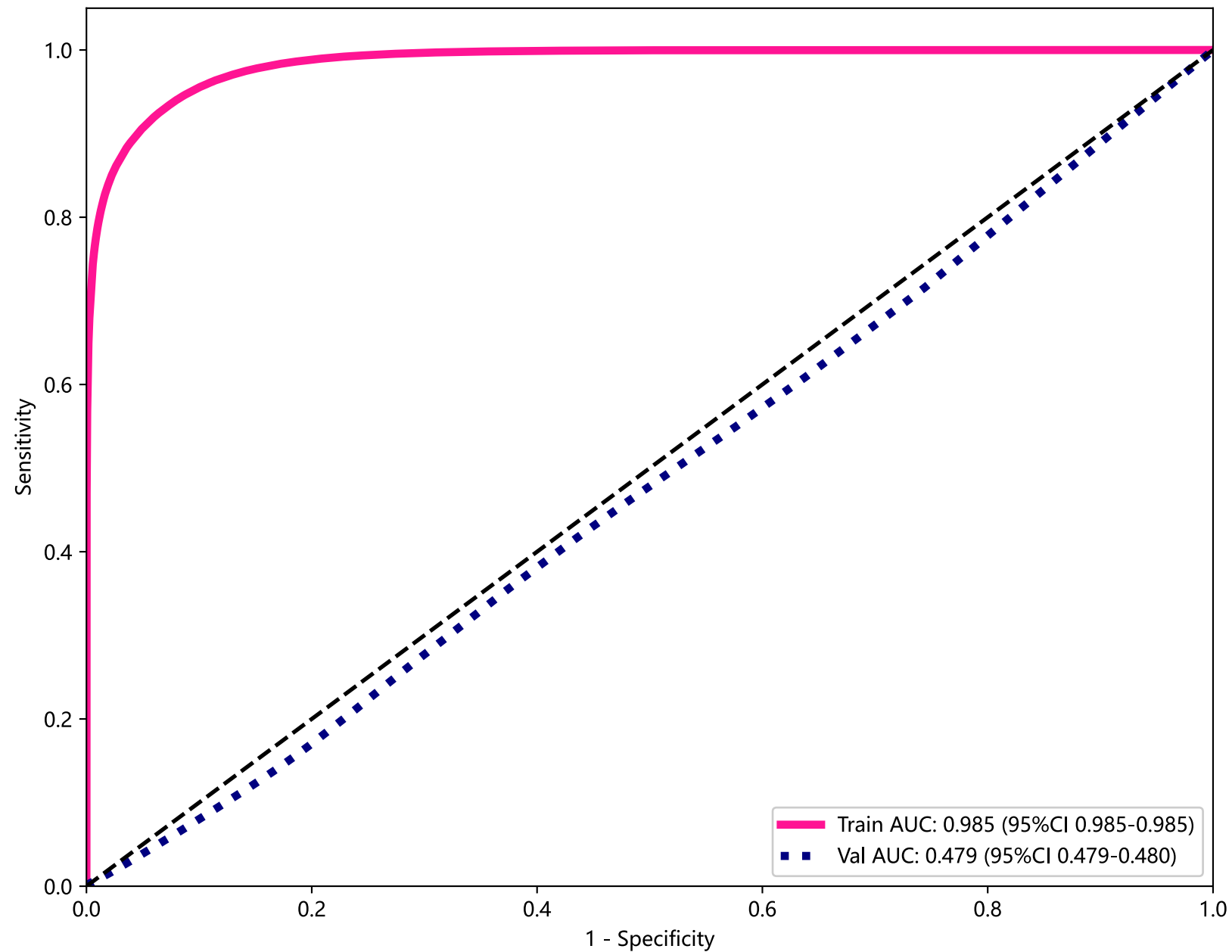
Model: resnet50
