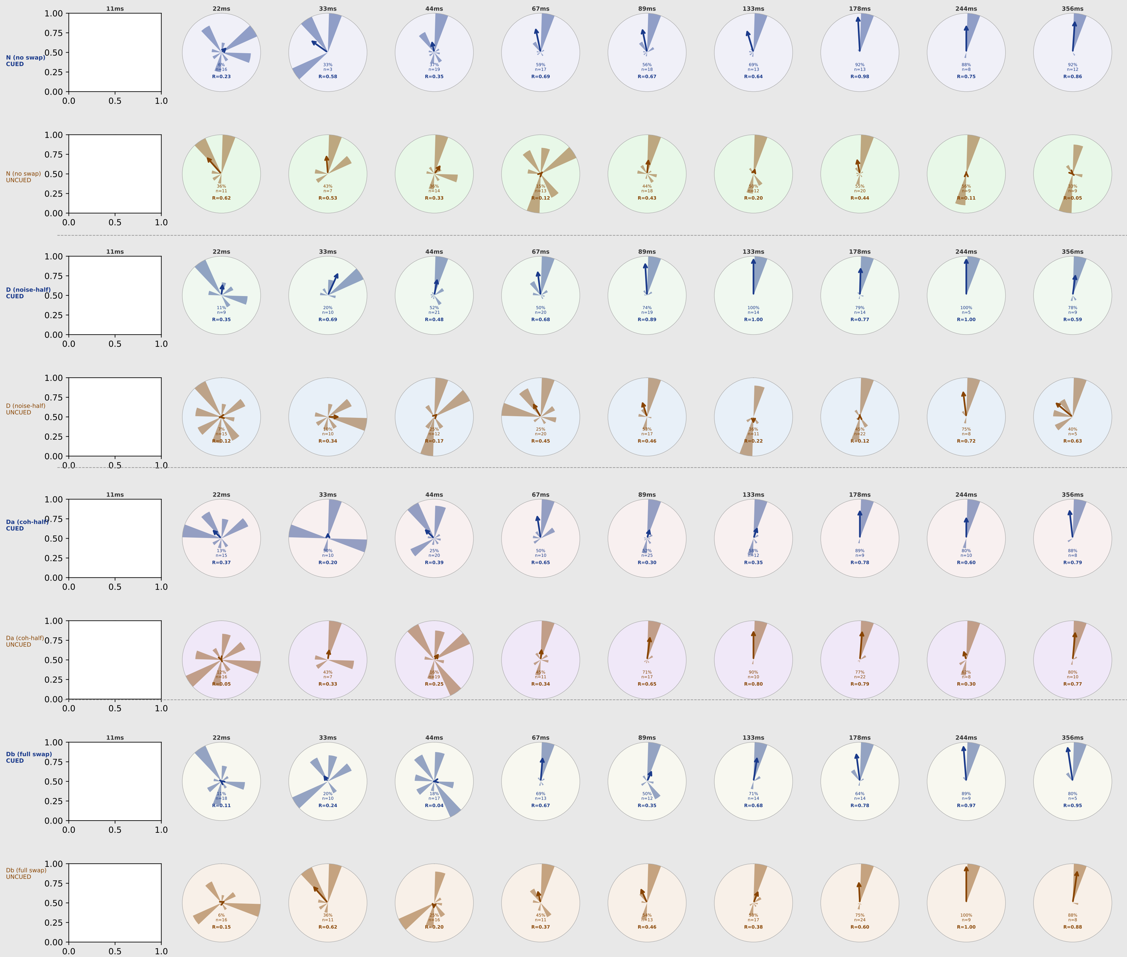
SubfieldSwap Ap35 — Response direction relative to correct heading (0° = correct) n=1026 (2 sessions). Duration increases left→right. Arrow = mean resultant.
