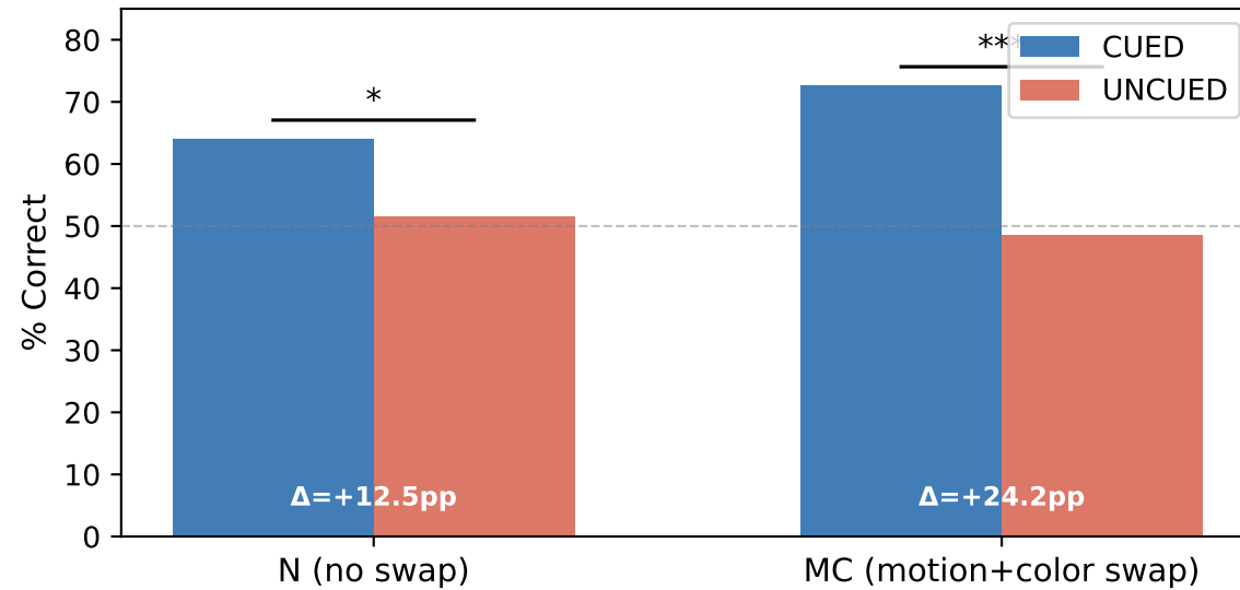
S&B Replication — Cueing Effect (44ms, Ap2.0°, 5 dots/deg²)
