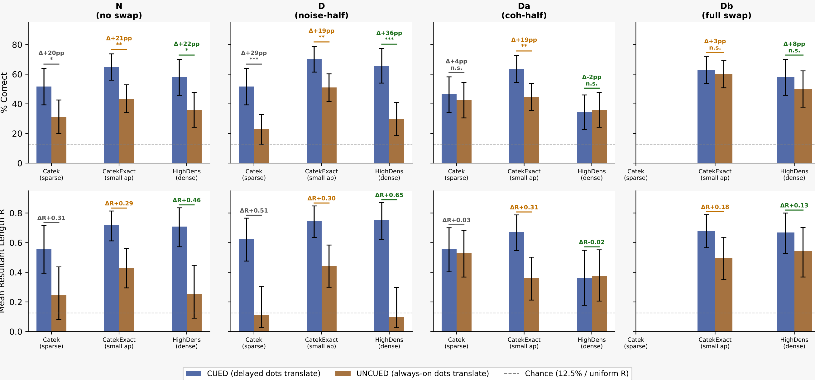
SubfieldSwap: comparison across experiments Error bars: \pm 1.96 SE (accuracy) | 95% bootstrap CI (R). \Delta brackets: CUED–UNCUED difference.
