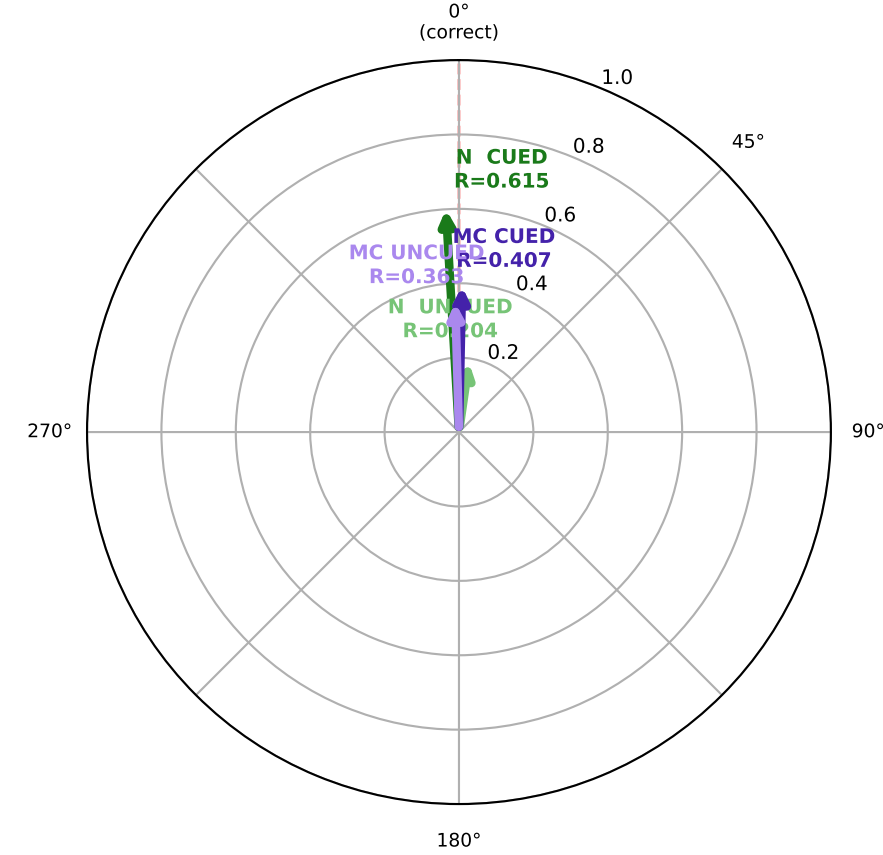
Vector Averages (R = arrow length)
