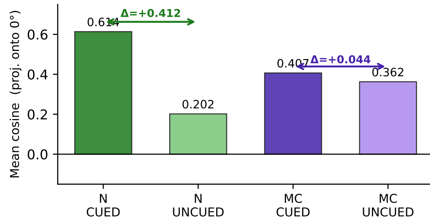
Projection onto Correct Direction
