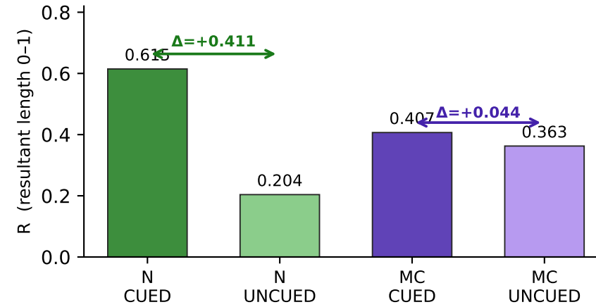
Vector Resultant Magnitude (R)
