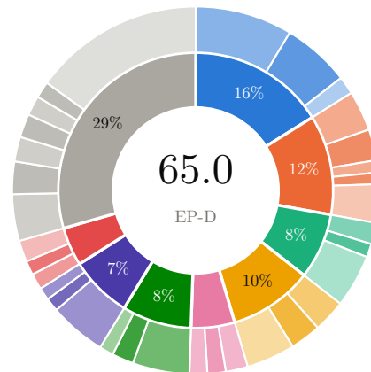
AssayFormer
