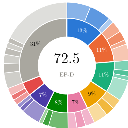
BPMF
