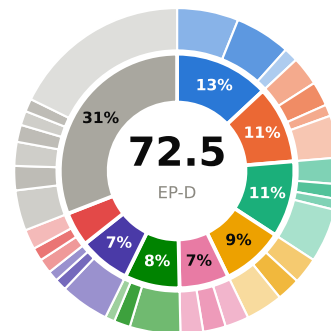
BPMF
