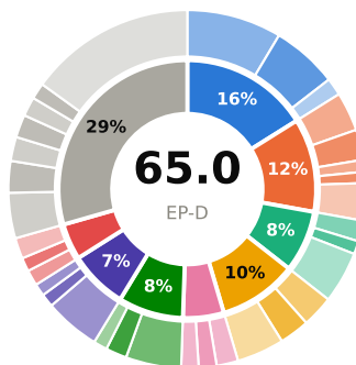
AssayFormer
