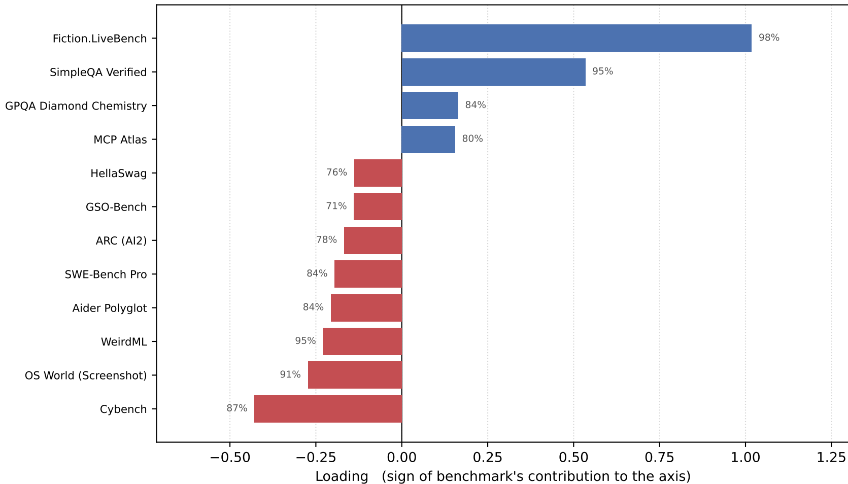
Axis 3 — 4% of total variance top 12 benchmarks by |loading| (% = sign agreement across posterior draws)
