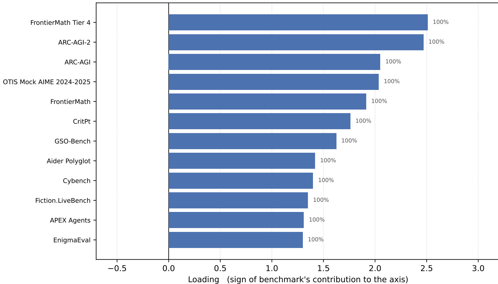
Axis 1 — 63% of total variance top 12 benchmarks by |loading| (% = sign agreement across posterior draws)
