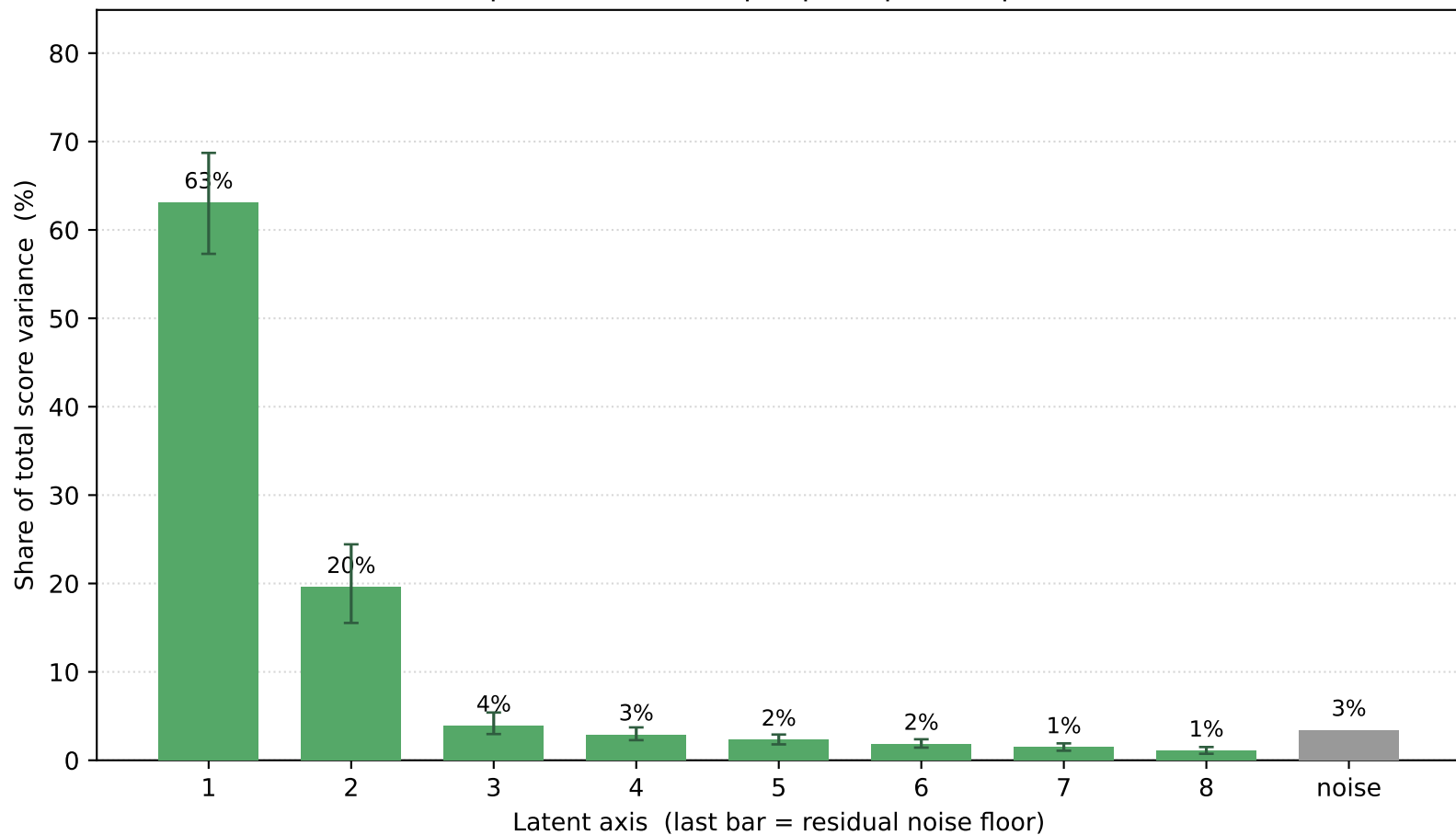
Explained variance per principal component
