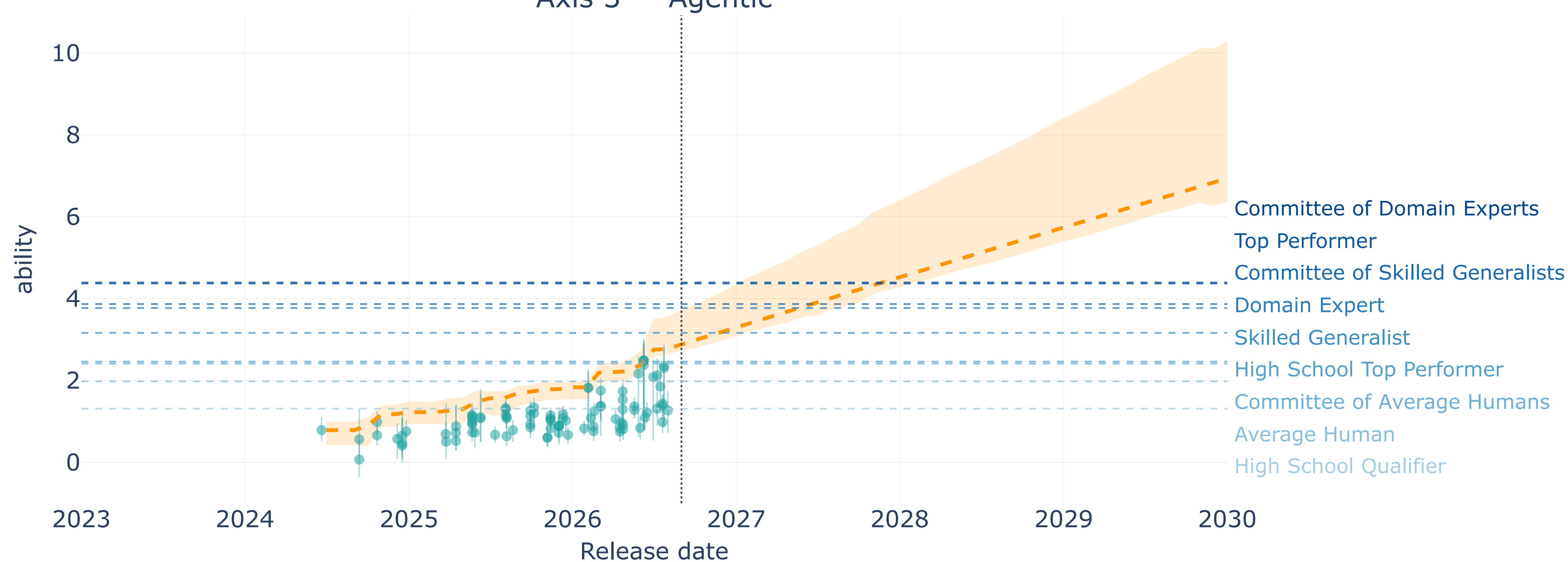
Axis 3 — Agentic
