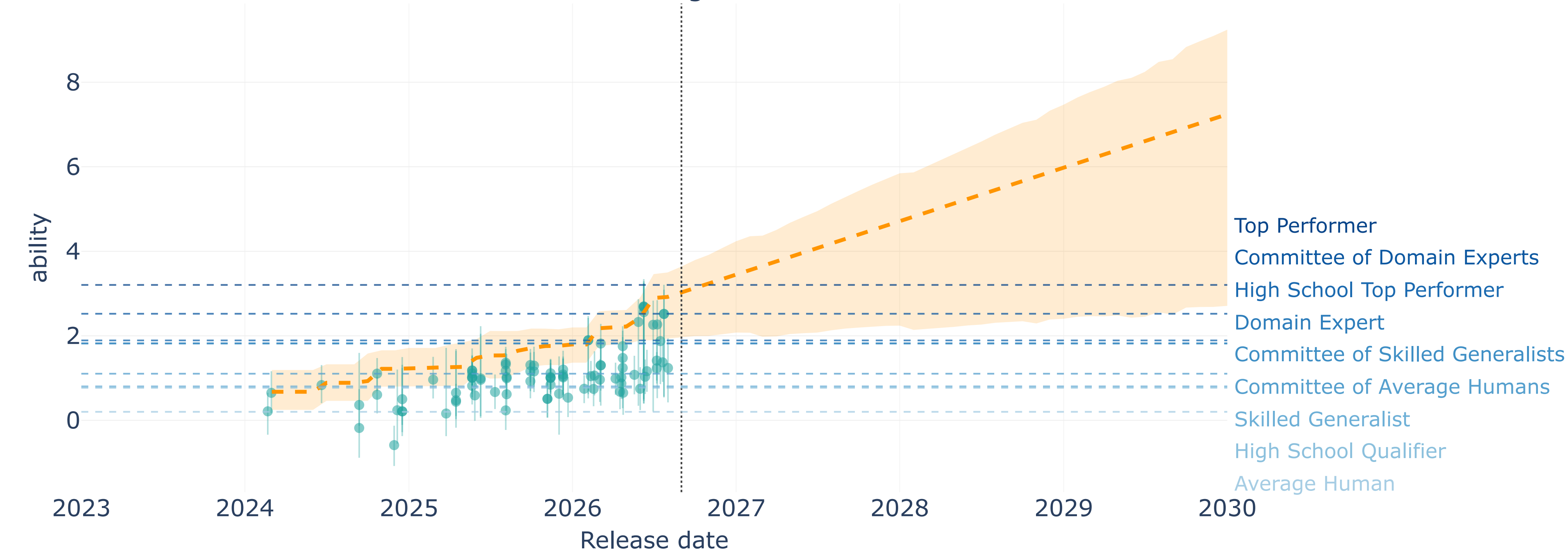
Axis 3 — Agentic
