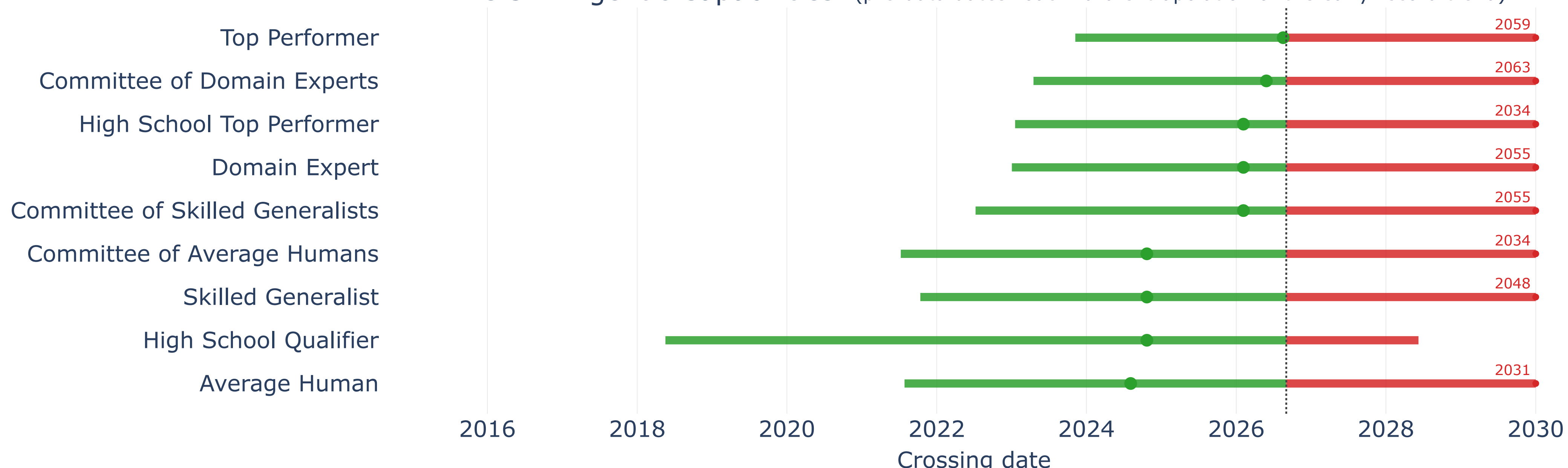
Axis 3 — Agentic Capabilities (pre-data dates: backward extrapolation of the early record trend)
