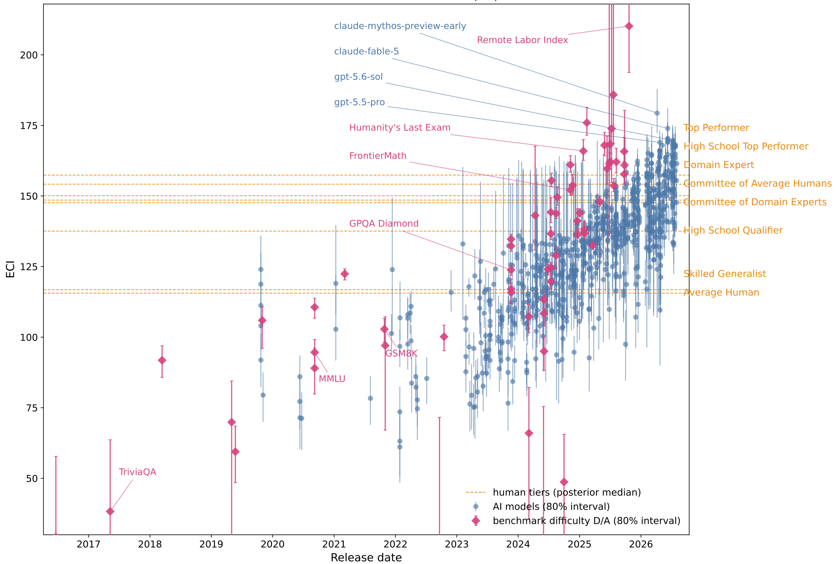
ECI timeline with benchmark difficulties (1D)
