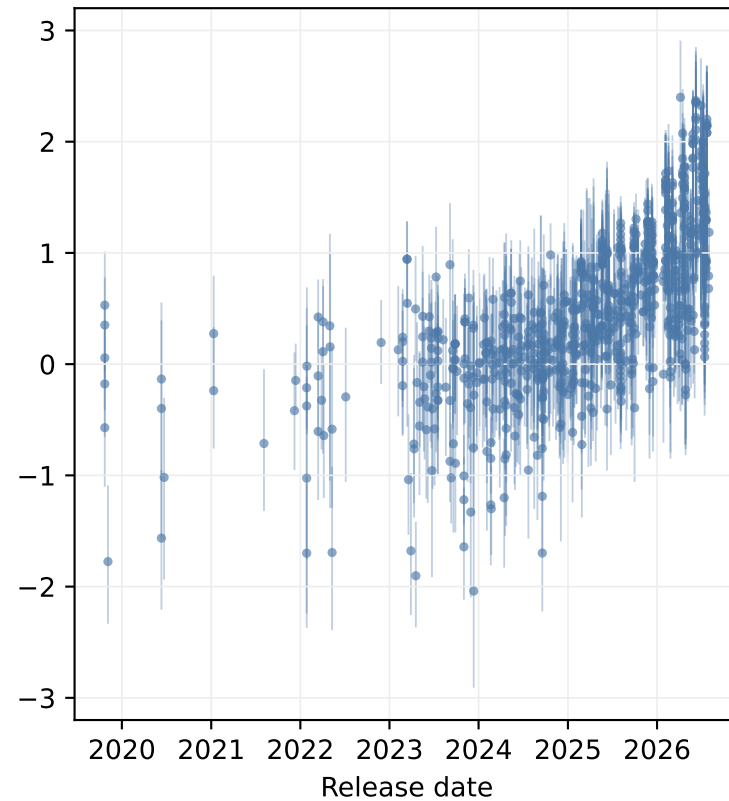
Axis 3 — Agentic
