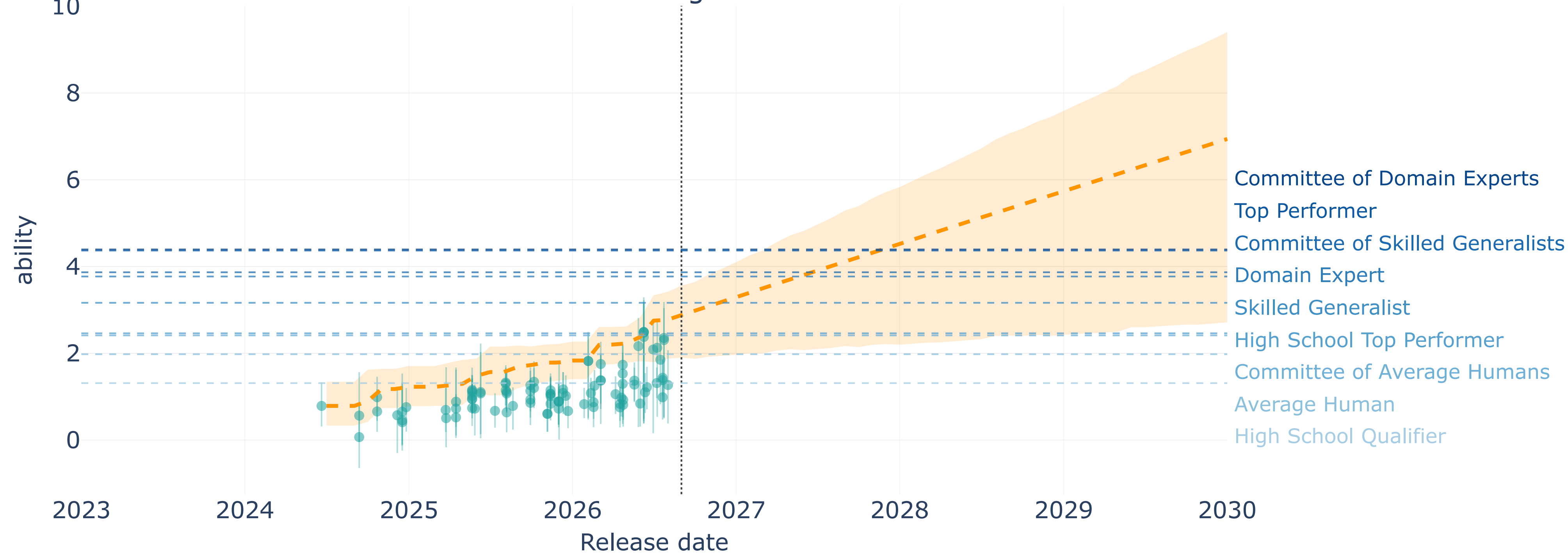
Axis 3 — Agentic
