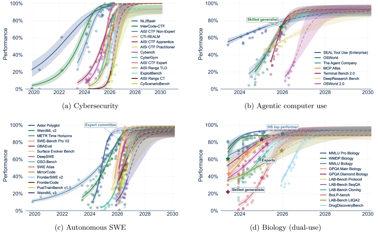
Figure 4: Security-critical capability trajectories. Benchmarks with direct safety implications show rapid progress, with most projected to saturate by 2027–2028; chemistry, which saturated earliest, is shown in Supp. Figure 6. Starred markers indicate human baselines where available. On OSWorld, users unfamiliar with the software achieve 72% (Xie et al., 2024); on biology benchmarks, domain experts range from 38% (BioLP-bench, laboratory practitioners) to 83% (GPQA Diamond Biology, in-domain PhDs) (Dev et al., 2025; Rein et al., 2023). Graphical conventions are similar to Figure 1.
