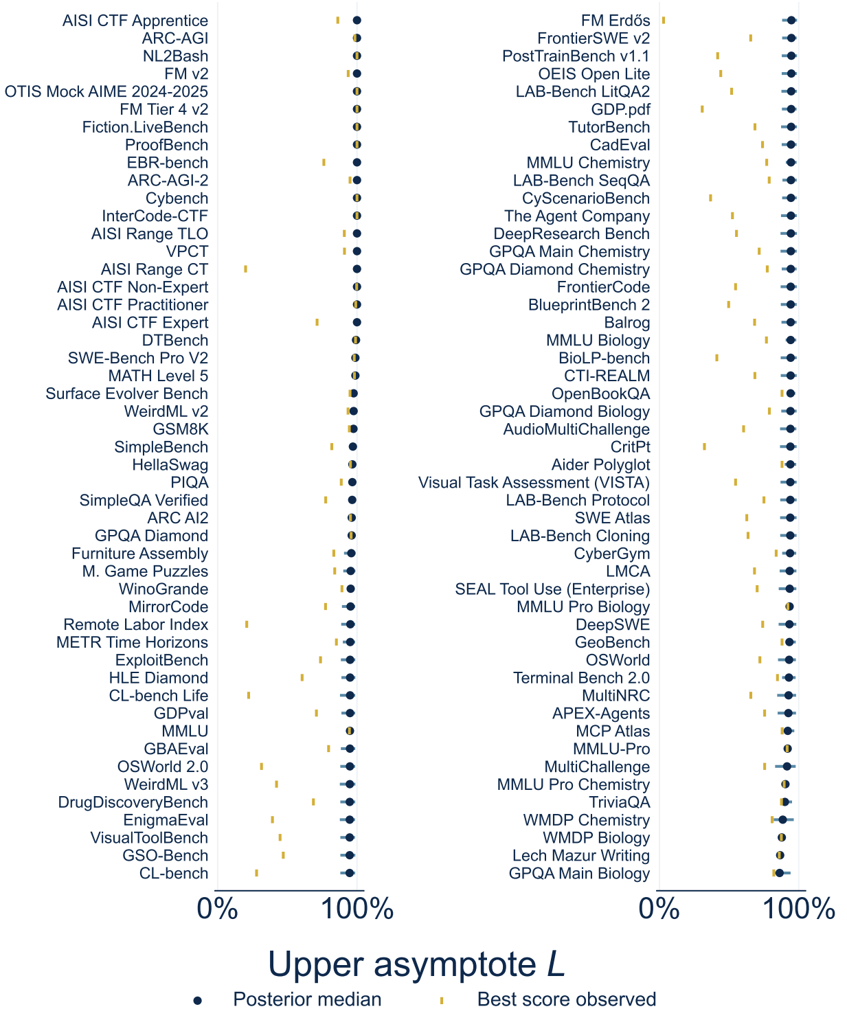
Figure 8: Upper asymptote estimates by benchmark. Posterior median and 80% credible interval of the upper asymptote L_i for each benchmark, ordered by median from the top of the left panel to the bottom of the right one, with the best score observed up to October 2026 marked by a vertical tick. The hierarchical structure allows partial pooling, so benchmarks with little data are shrunk toward the population distribution.
