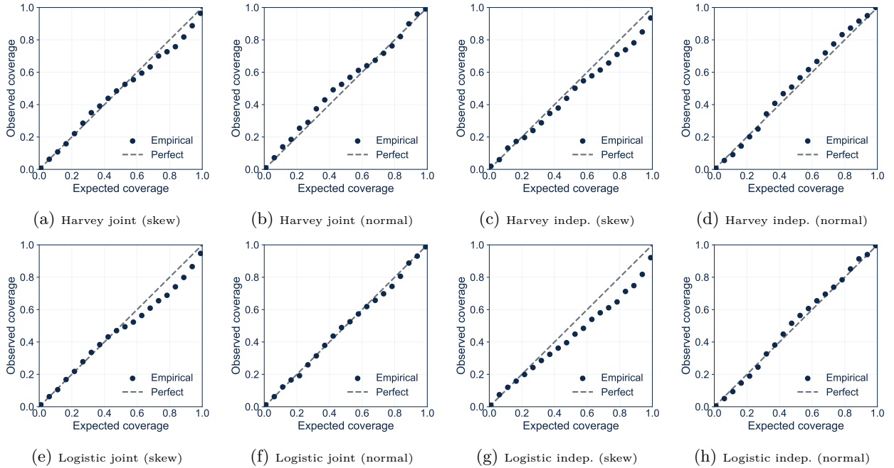
Figure 5: Calibration curves for all 8 model variants. Well-calibrated models produce points close to the diagonal. Normal-likelihood variants come closest to nominal coverage on this holdout; skew-normal variants have intervals that are somewhat too narrow.
