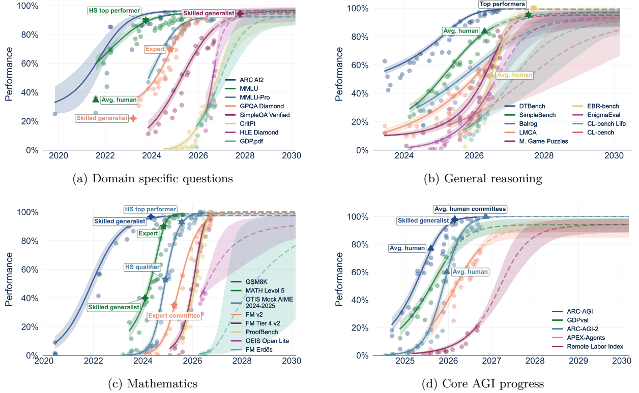
Figure 1: Benchmark trajectories across capability categories. Points show frontier model scores at release; solid lines show posterior mean trajectories; shaded regions indicate 80% credible intervals. Dashed lines extrapolate to 2030. Human reference points are star-like symbols whose number of branches denotes the expertise level: 3 for average human, 4 for skilled generalist, 5 for domain expert, and 6 for top performer. See more details in Appendix F. All categories show rapid progress towards saturation, with several benchmarks already exceeding human expert baselines.
