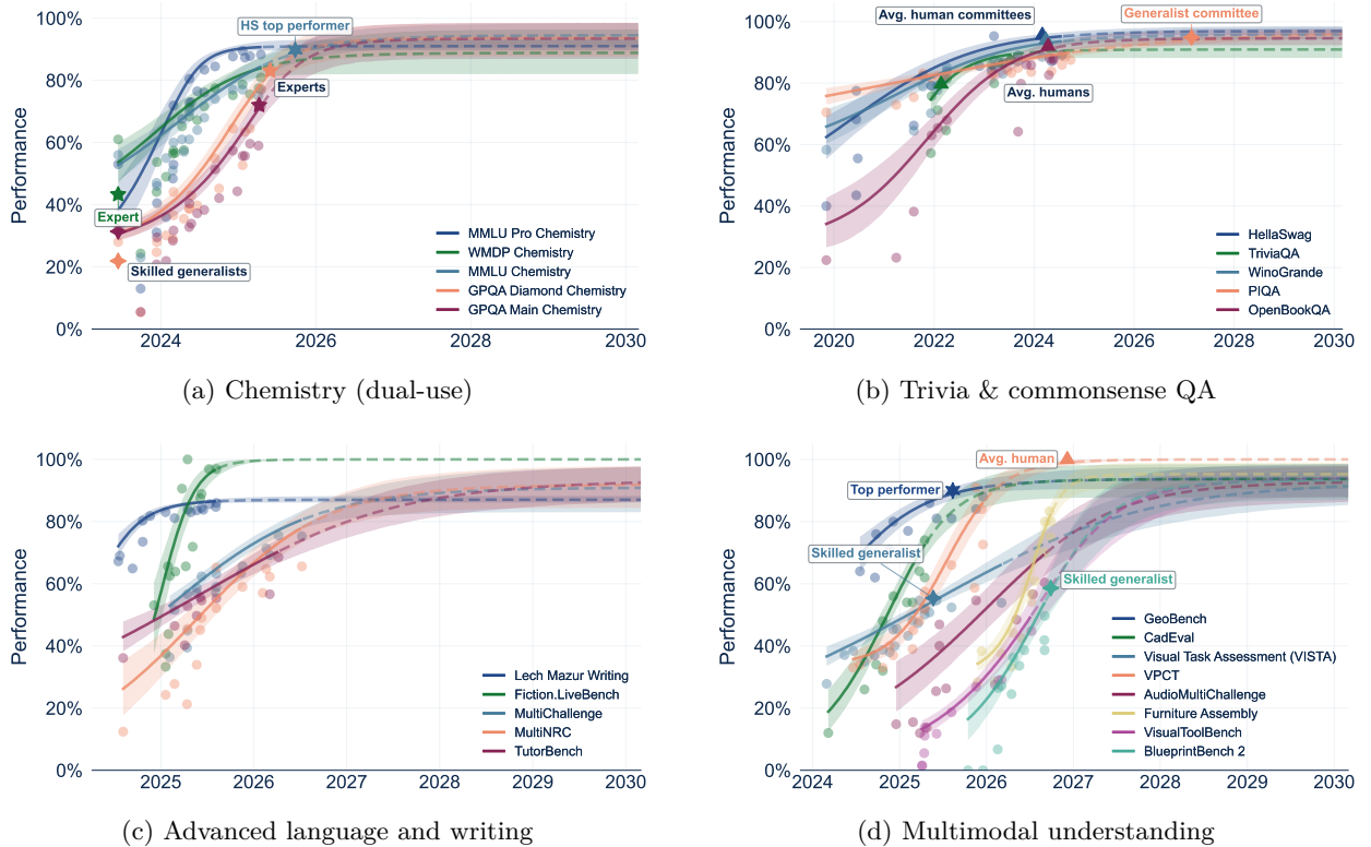
Figure 6: Additional benchmark trajectories. Chemistry benchmarks are already saturated; trivia and commonsense benchmarks are at or near saturation; language and multimodal understanding show trajectories consistent with other categories. Graphical conventions are similar to Figure 1.
