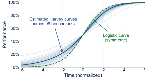
Figure 2: Harvey curves capture asymmetric progress. Fitted Harvey curves (blue) show more gradual acceleration compared to the logistic (green dashed). Curves are standardized to 50% at time 0 with growth rate 1. The thick blue curve is the median Harvey trajectory.
