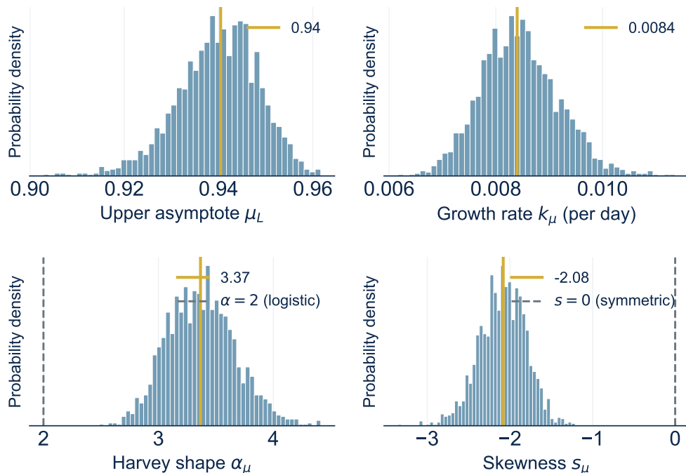
Figure 7: Hierarchical model hyperparameters. Posterior distributions for the joint Harvey model hyperparameters, controlling the population-level distribution of upper asymptotes ( L_{\min} + (1 - L_{\min})\mu_L ), growth rates ( k_\mu ), Harvey shapes ( \alpha_\mu = 1 + \alpha_\mu^{\text{raw}} ), and skewness ( s_\mu ) across benchmarks. Solid lines mark the posterior medians; dashed lines mark \alpha_\mu = 2 , at which the Harvey curve reduces to a logistic, and s_\mu = 0 .
