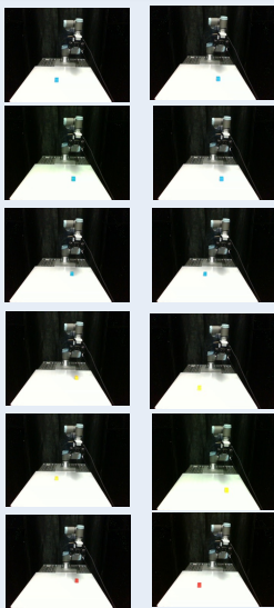
Color, Position
