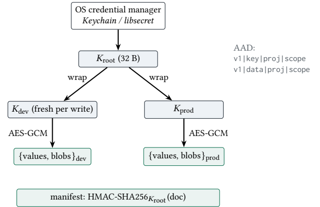
Figure 3: Vault key hierarchy. Rewriting a scope rotates its data key; AAD binds every ciphertext to its project and scope.
