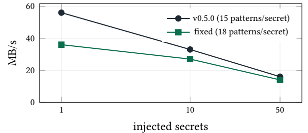
Figure 5: Redactor throughput. Terminal-scale output is far below either curve.
