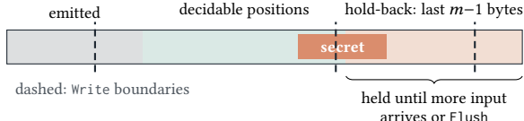
Figure 4: The scanner only decides positions that have at least m-1 bytes of lookahead, so a secret that straddles one or more Write boundaries is still seen whole.
