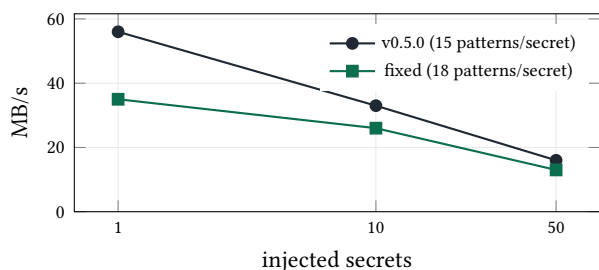
Figure 5: Redactor throughput. Terminal-scale output is far below either curve.
