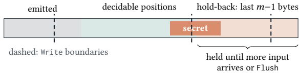
Figure 4: The scanner only decides positions that have at least m - 1 bytes of lookahead, so a secret that straddles one or more Write boundaries is still seen whole.
