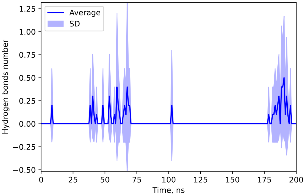
Hydrogen bonds number between 15557444 and TIAM
