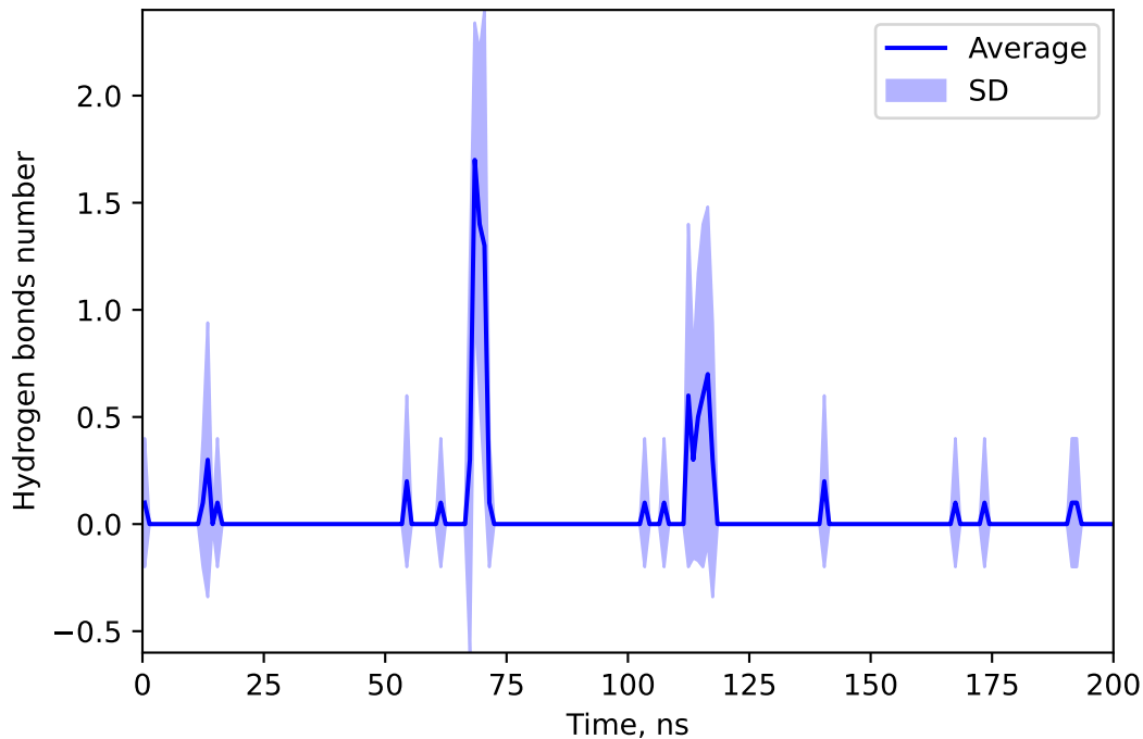
Hydrogen bonds number between 73293549 and RONI
