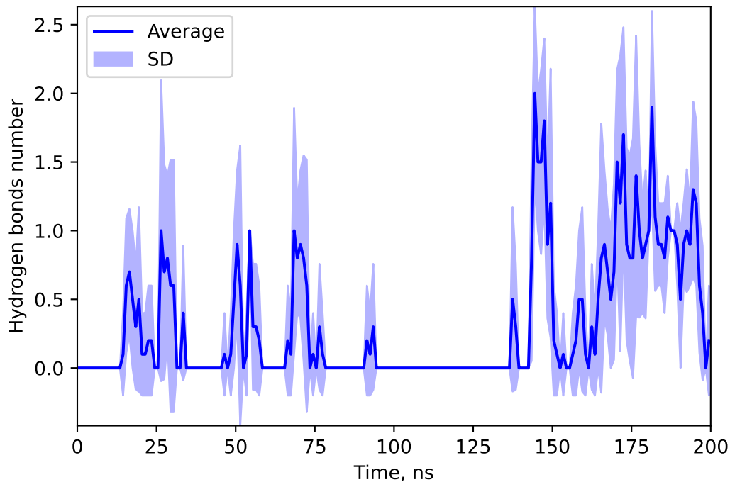
Hydrogen bonds number between 166625339 and DEME
