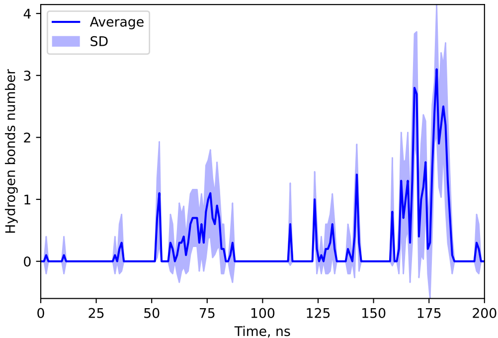
Hydrogen bonds number between 145975502 and SPIR
