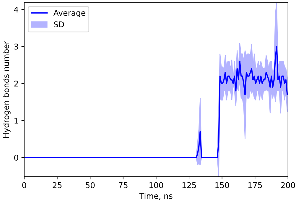
Hydrogen bonds number between 137644274 and STRE
