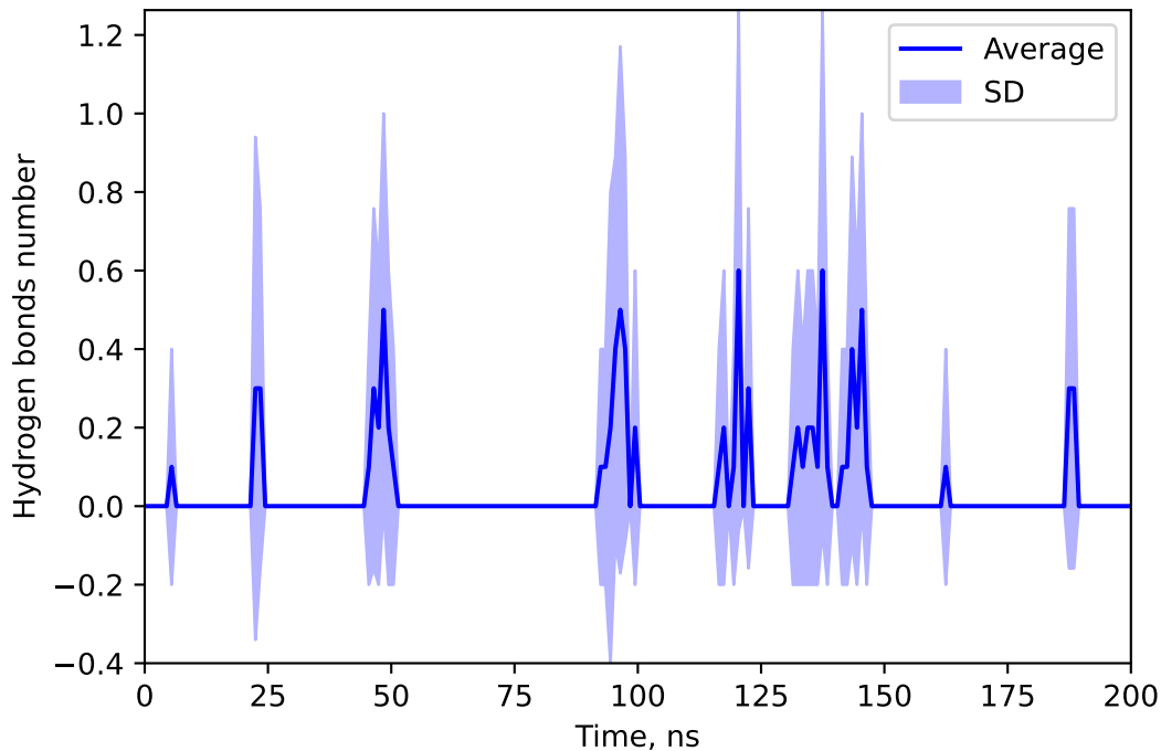
Hydrogen bonds number between 155521967 and SULF
