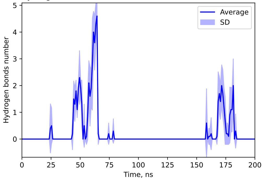
Hydrogen bonds number between 155557444 and CEFA
