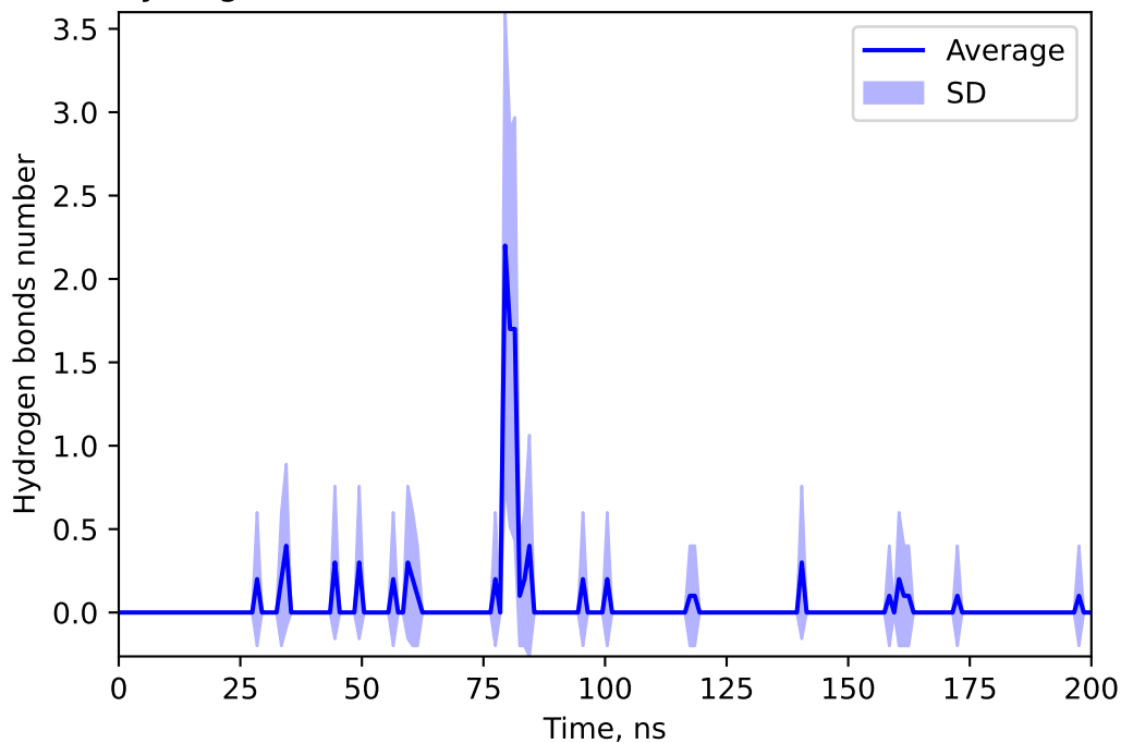
Hydrogen bonds number between 155521967 and RONI
