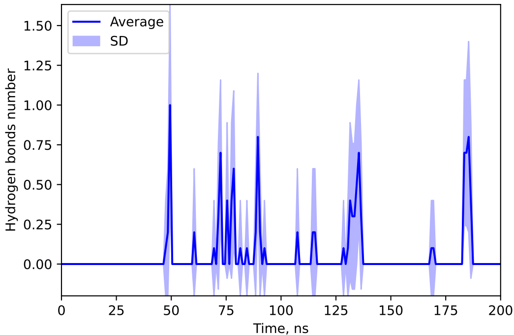
Hydrogen bonds number between 44569229 and TIAM
