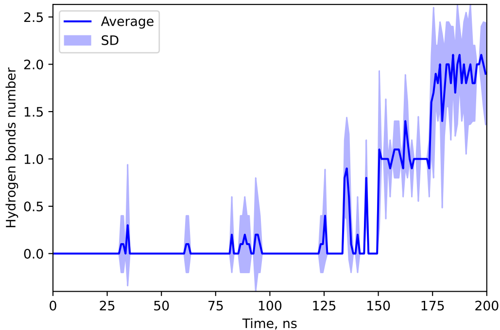
Hydrogen bonds number between 127034107 and DOXY
