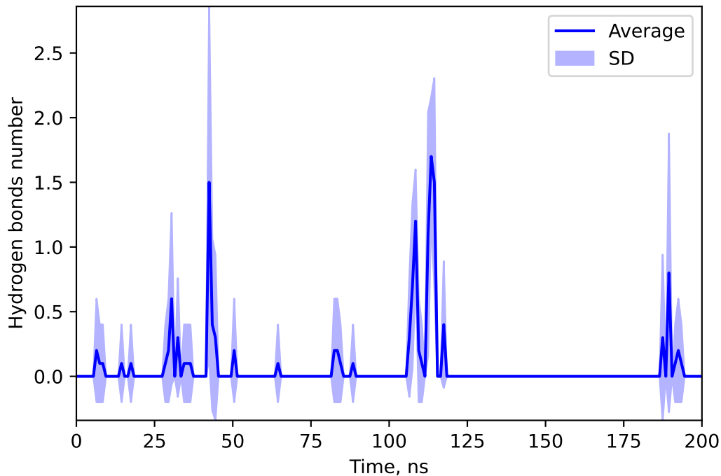
Hydrogen bonds number between 195797 and DOXY
