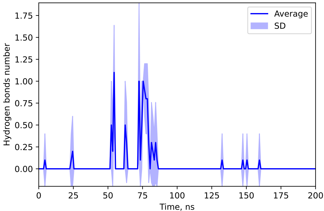
Hydrogen bonds number between 155514020 and LYNC
