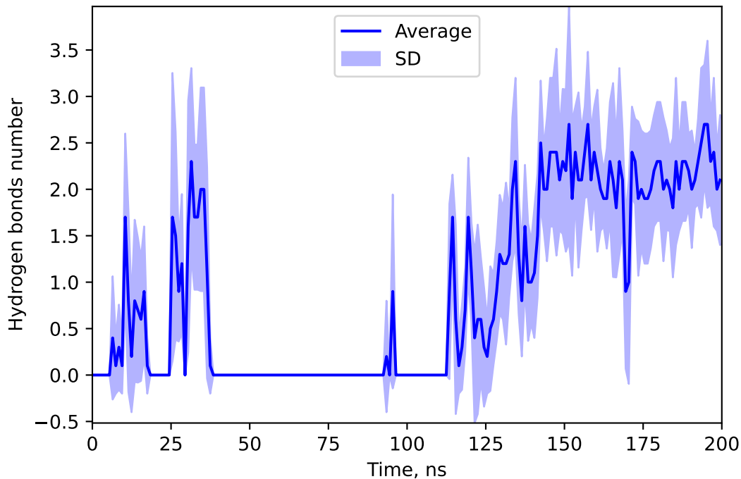
Hydrogen bonds number between 137644274 and DEME
