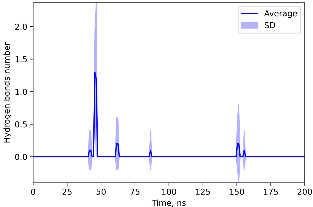
Hydrogen bonds number between 127034107 and STRE
