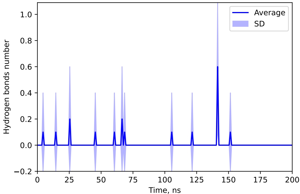
Hydrogen bonds number between 155521967 and TIAM
