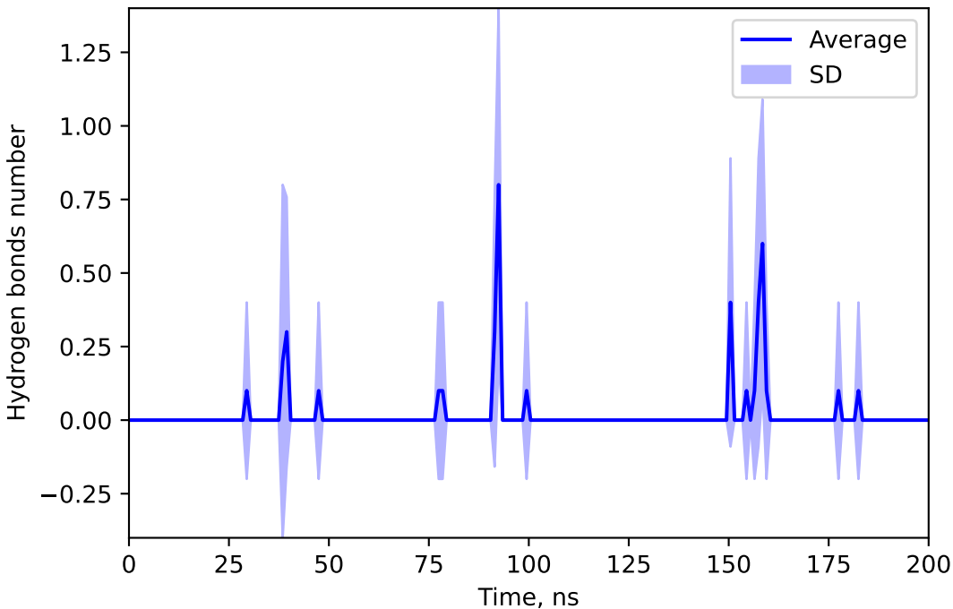
Hydrogen bonds number between 44569229 and METR
