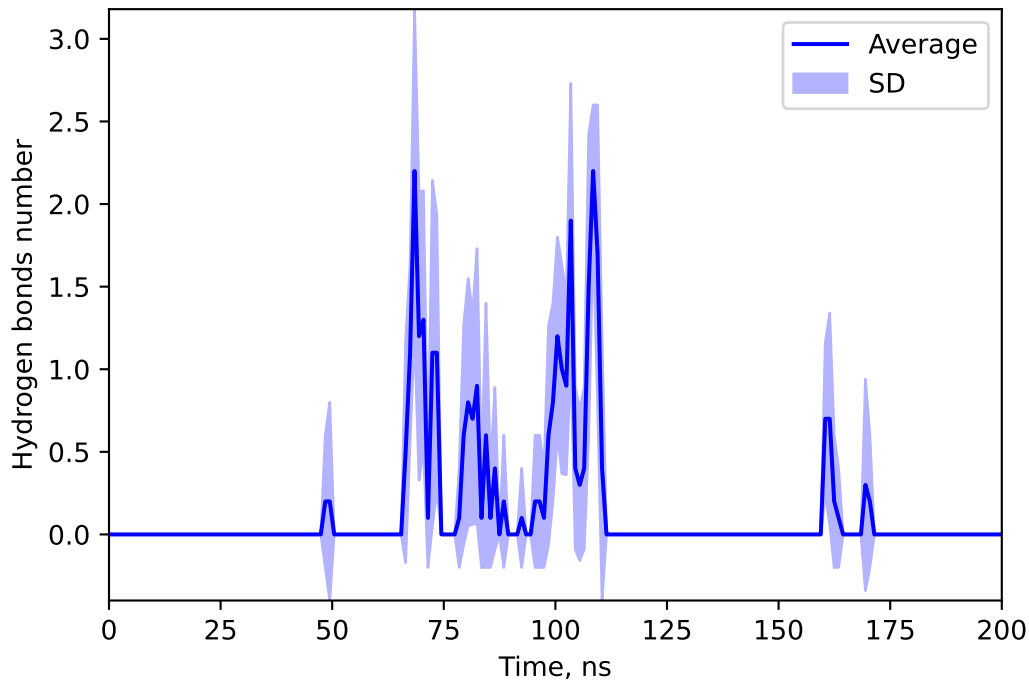
Hydrogen bonds number between 155518747 and DOXY
