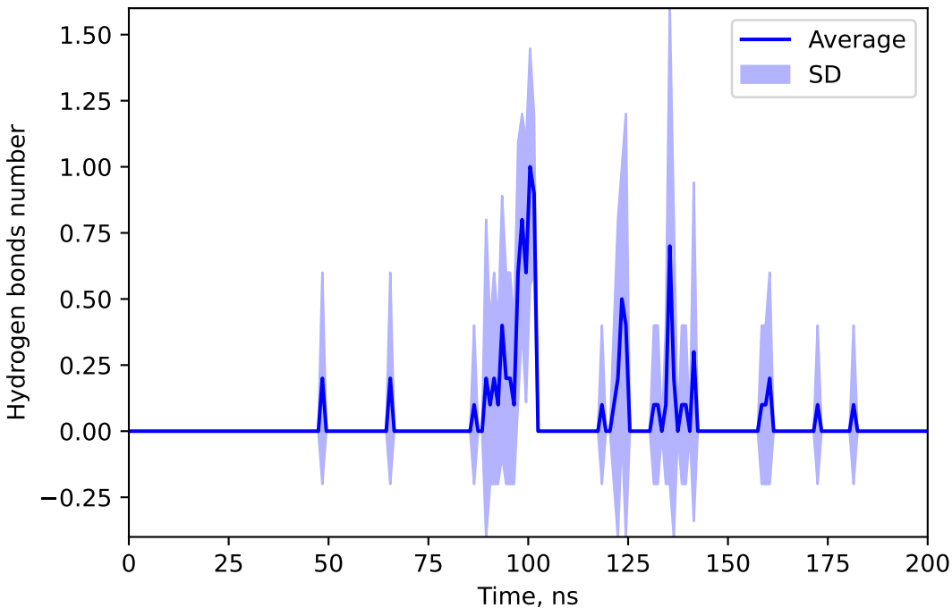
Hydrogen bonds number between 44575206 and DEME
