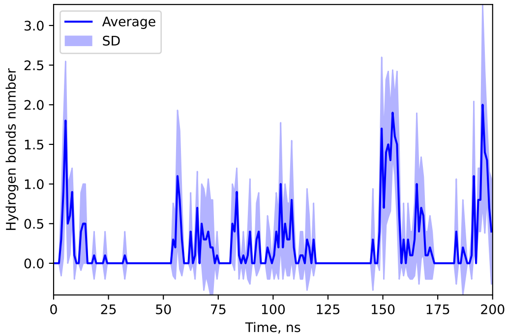
Hydrogen bonds number between 137644274 and DANO
