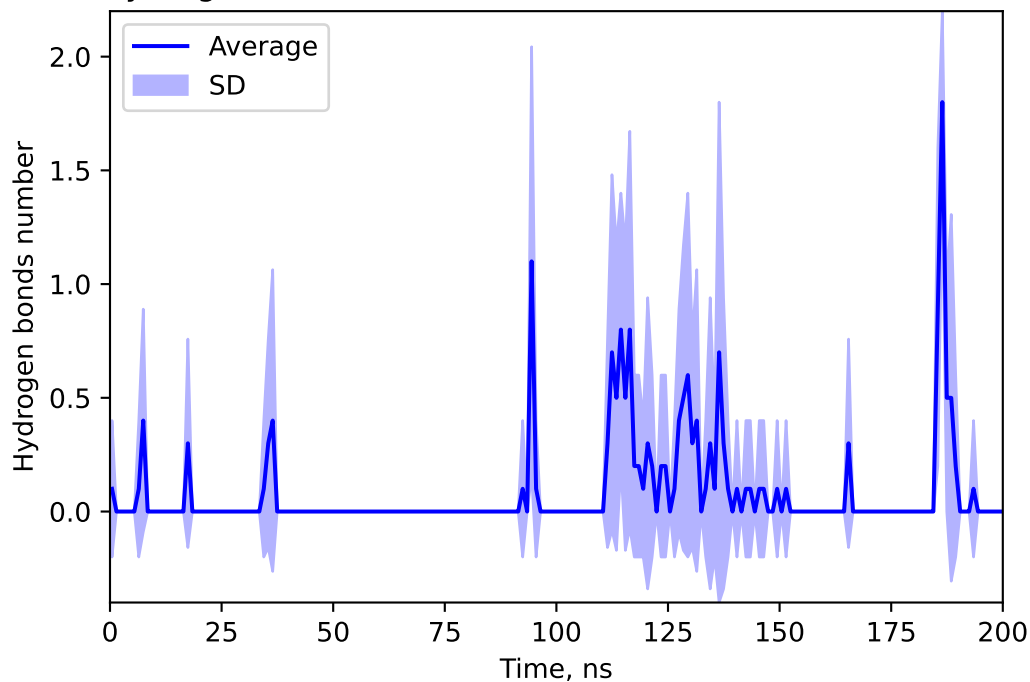
Hydrogen bonds number between 155521967 and DOXY
