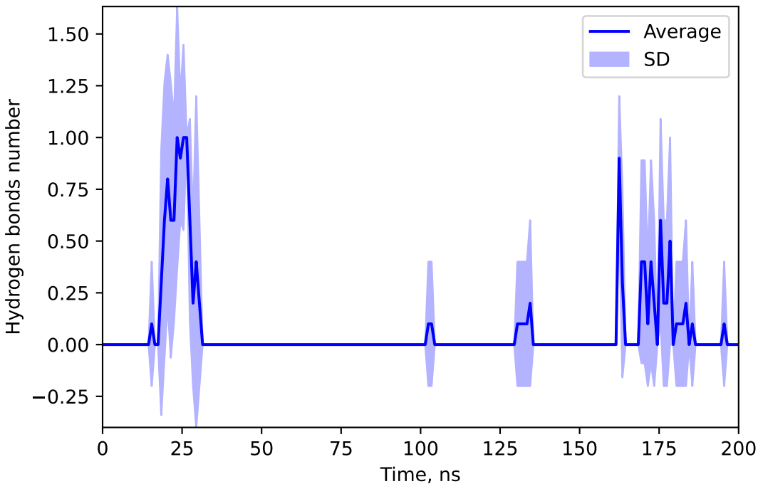
Hydrogen bonds number between 155559627 and TIAM
