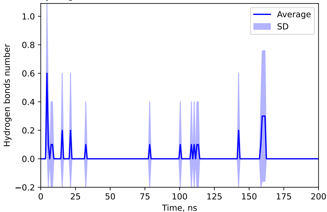
Hydrogen bonds number between 155521967 and METR
