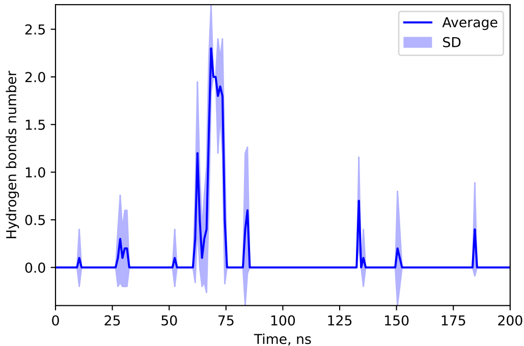
Hydrogen bonds number between 155518747 and LYNC
