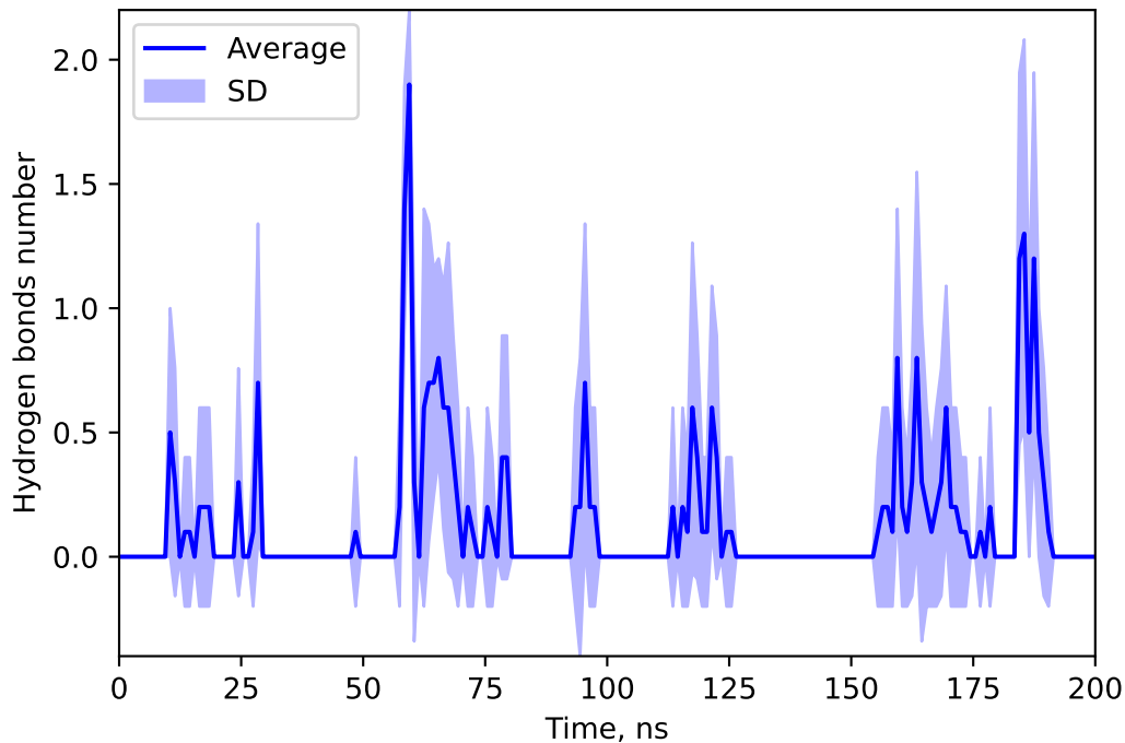
Hydrogen bonds number between 44575206 and SULF
