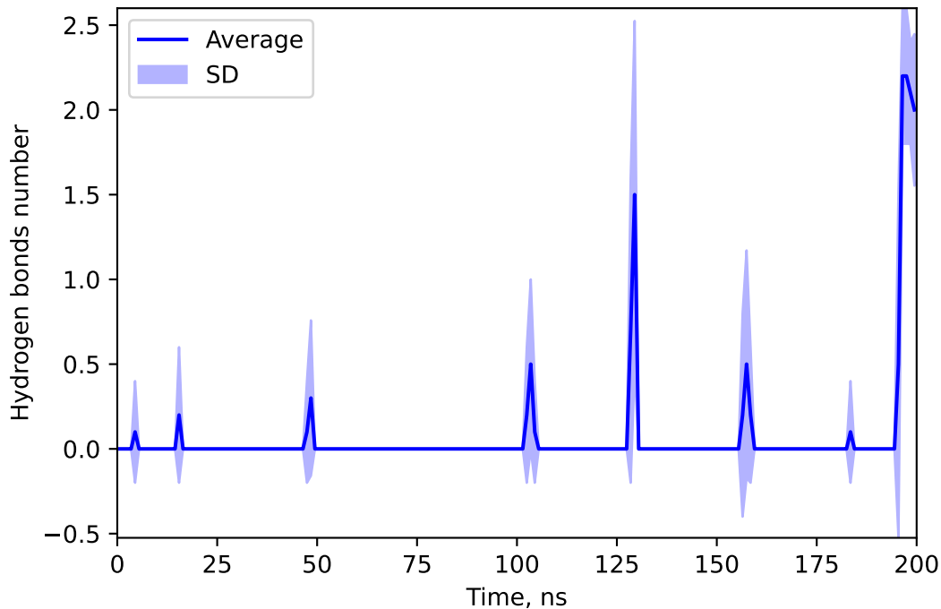
Hydrogen bonds number between 137646969 and STRE
