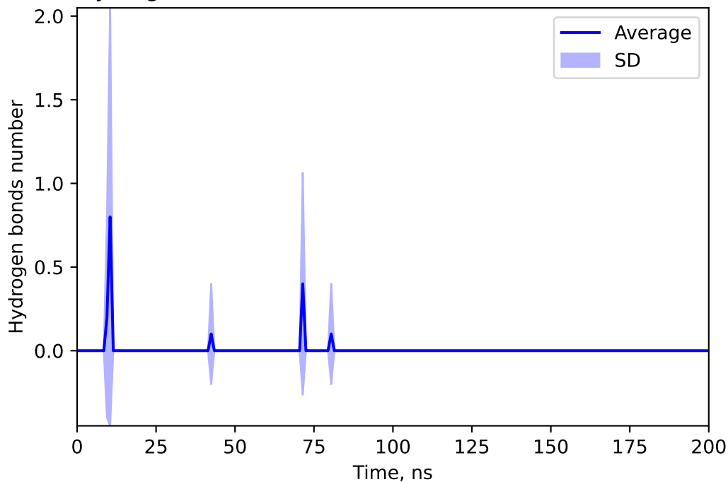
Hydrogen bonds number between 73293549 and METR
