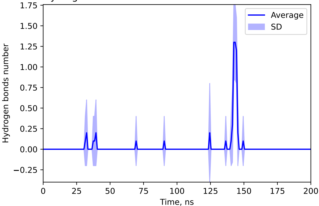
Hydrogen bonds number between 15559627 and SPIR
