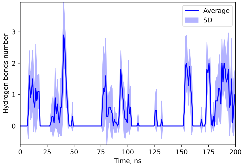
Hydrogen bonds number between 137644274 and CEFA
