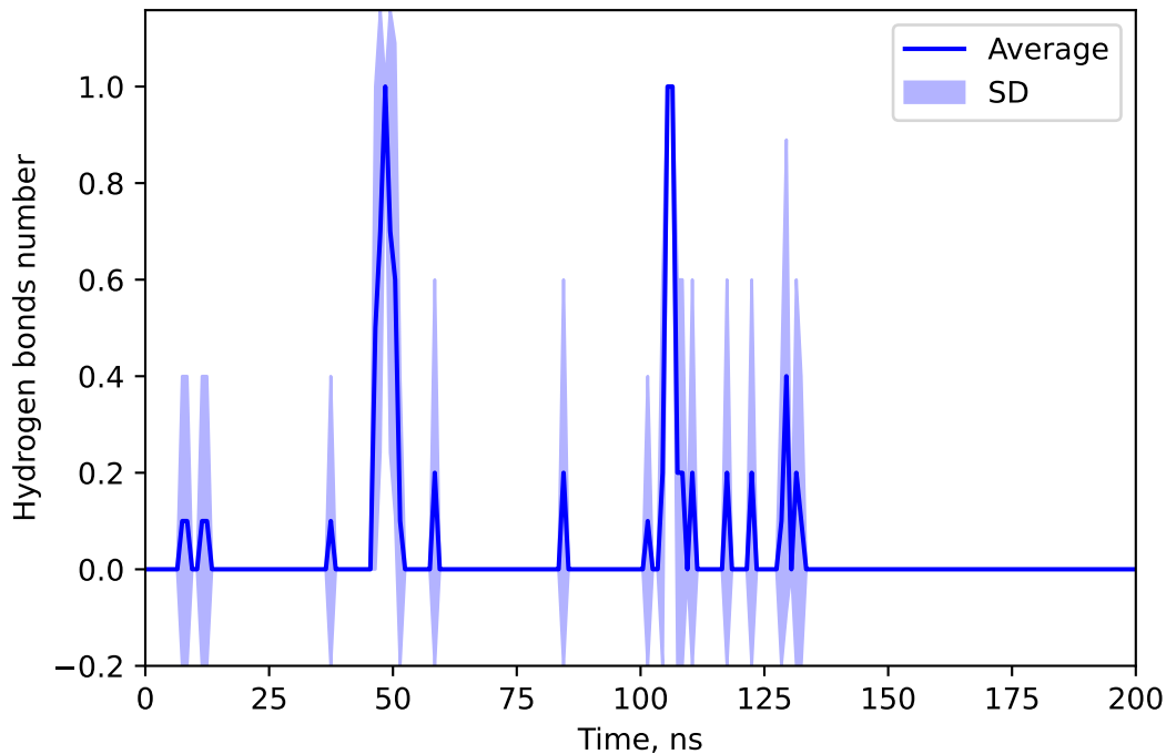
Hydrogen bonds number between 127034107 and TIAM
