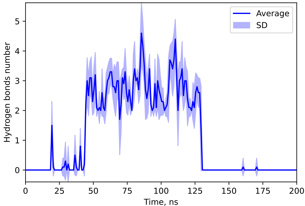
Hydrogen bonds number between 155521967 and STRE
