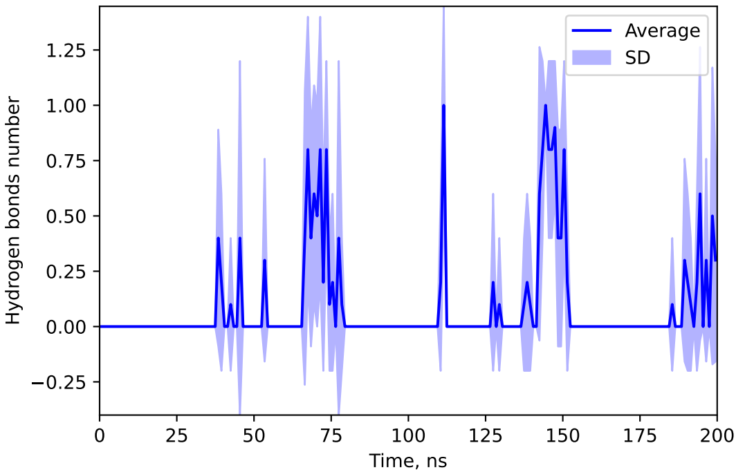
Hydrogen bonds number between 73293549 and DANO
