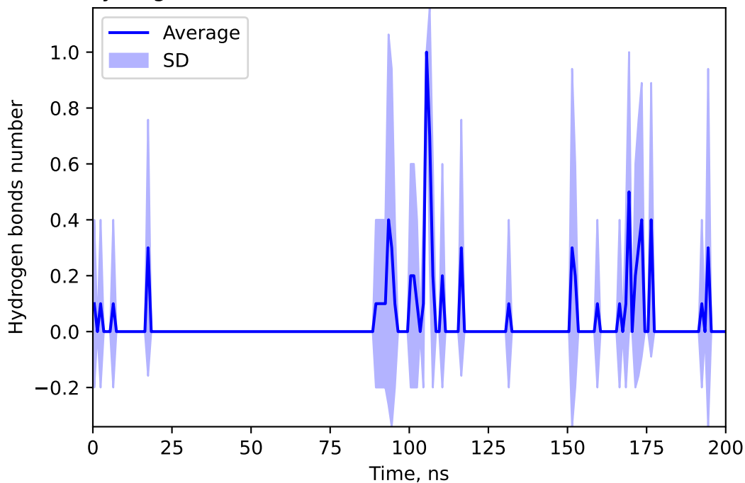
Hydrogen bonds number between 127034107 and DANO
