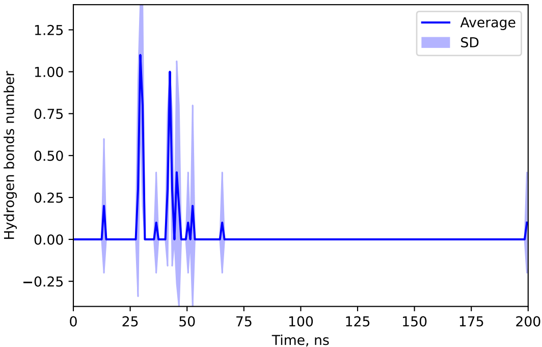
Hydrogen bonds number between 44575206 and TILM
