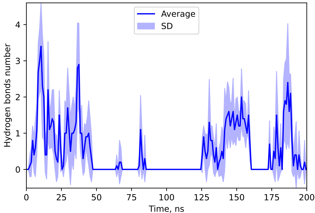
Hydrogen bonds number between 73293549 and CEFA
