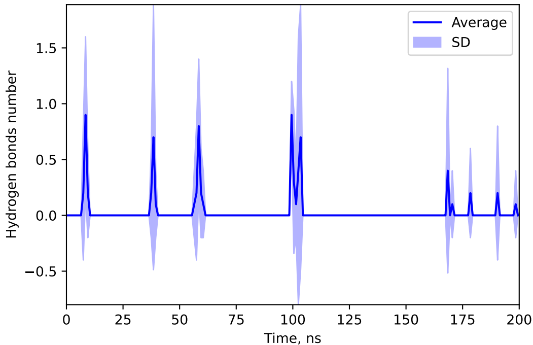
Hydrogen bonds number between 155514020 and CEFA
