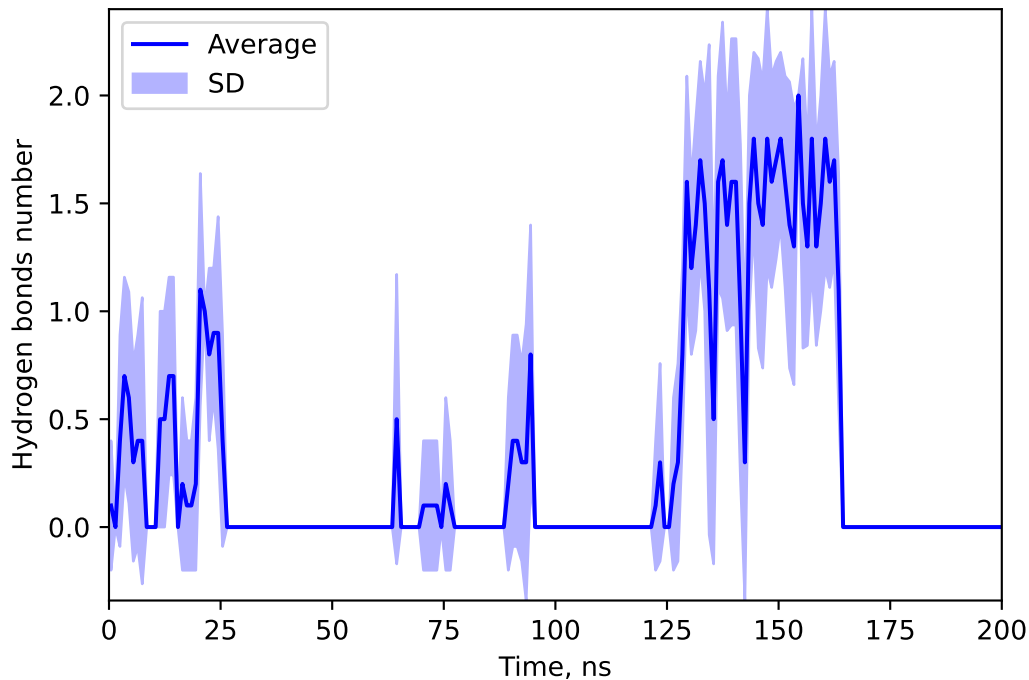
Hydrogen bonds number between 155557444 and SULF
