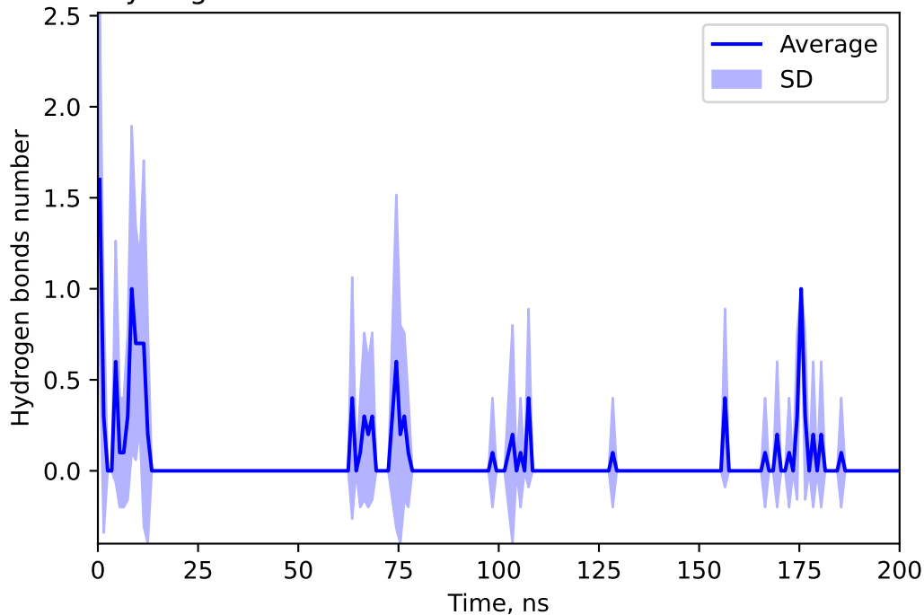
Hydrogen bonds number between 44575206 and LYNC
