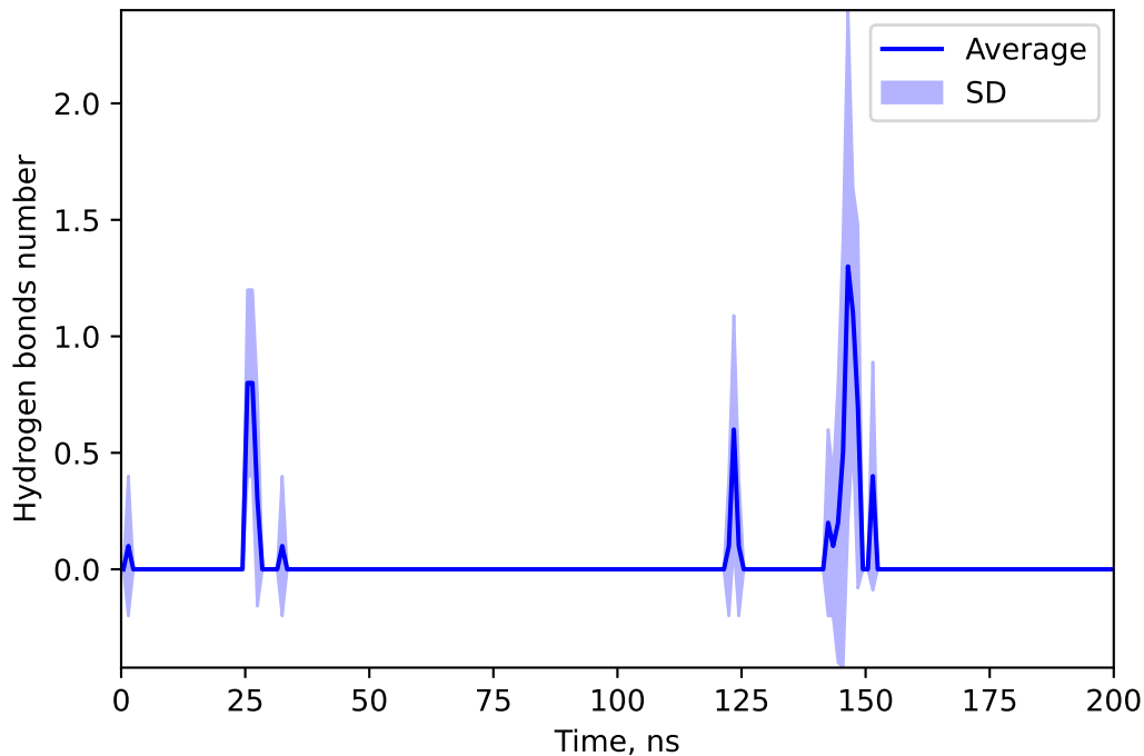
Hydrogen bonds number between 155514020 and SPIR
