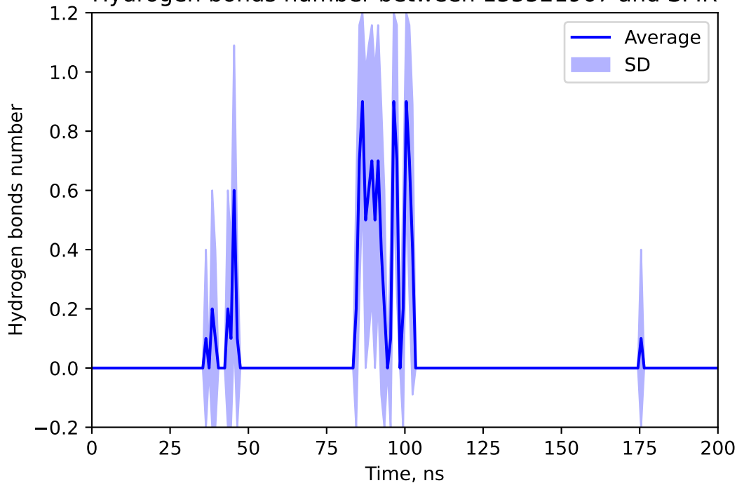
Hydrogen bonds number between 155521967 and SPIR
