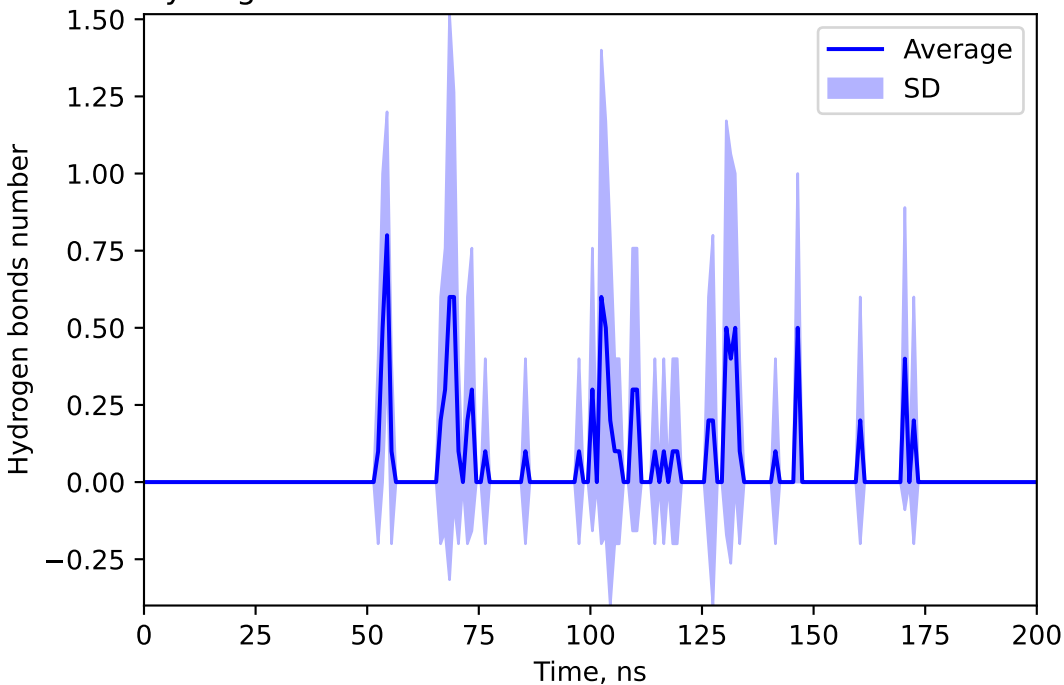
Hydrogen bonds number between 155518747 and TIAM
