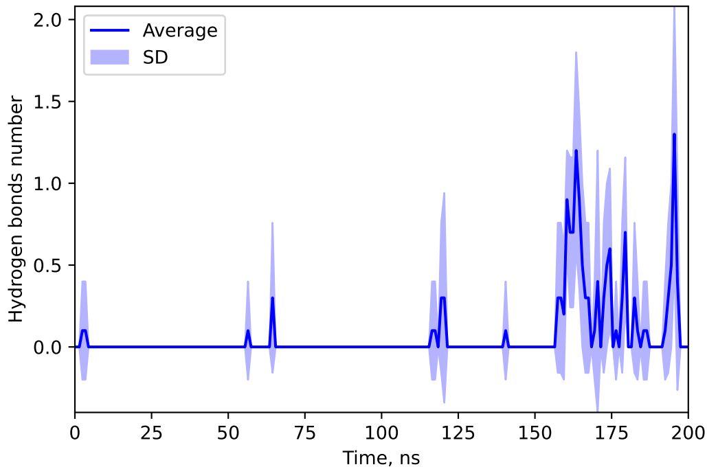
Hydrogen bonds number between 44569229 and TILM
