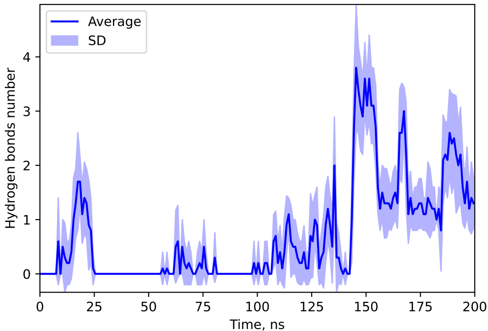
Hydrogen bonds number between 155514020 and DEME
