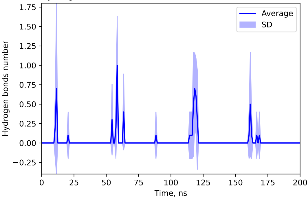
Hydrogen bonds number between 137646969 and RONI
