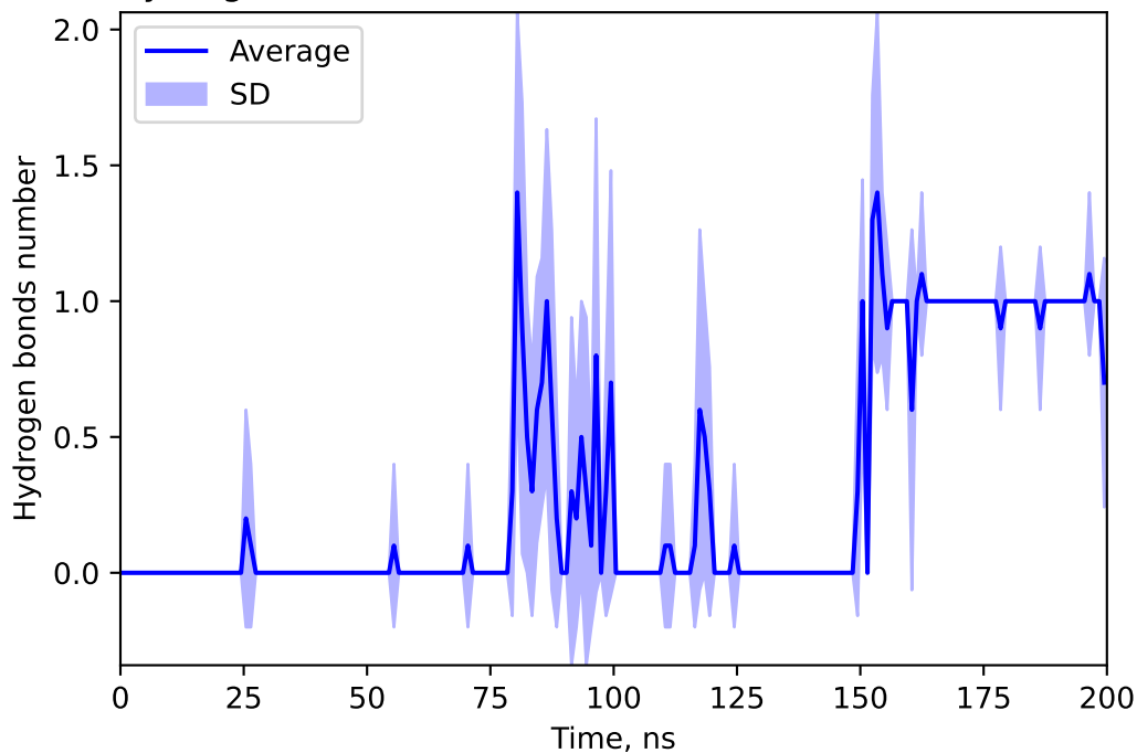
Hydrogen bonds number between 166625339 and LYNC
