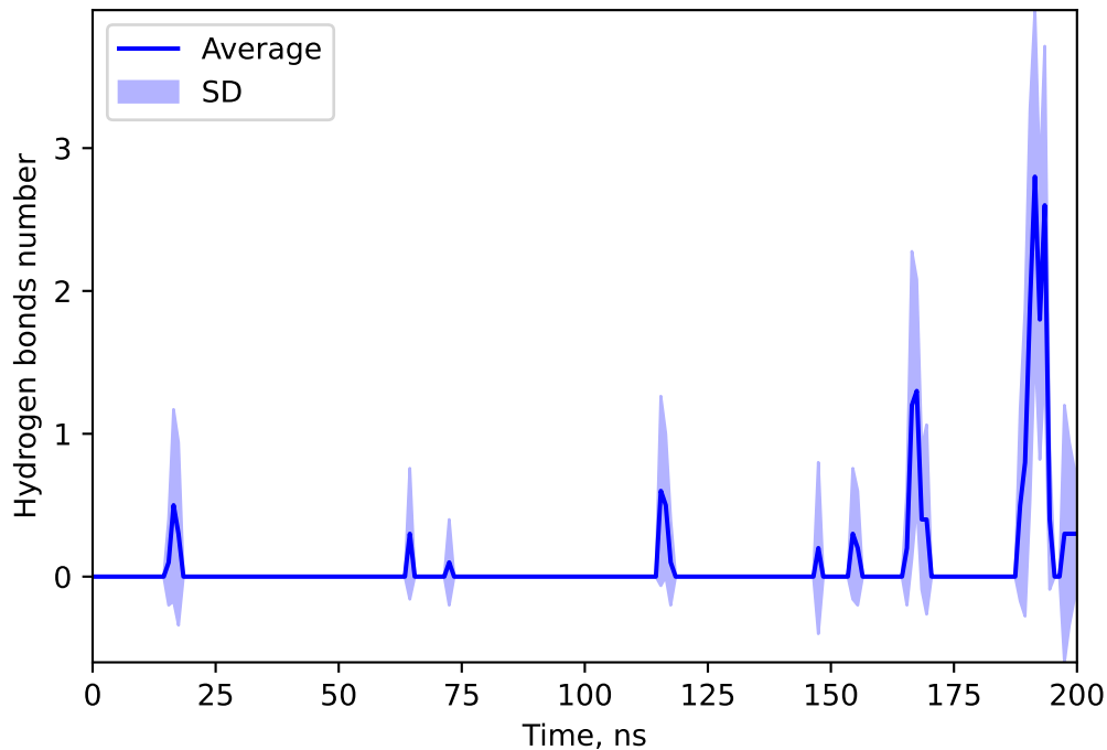
Hydrogen bonds number between 155518747 and RONI
