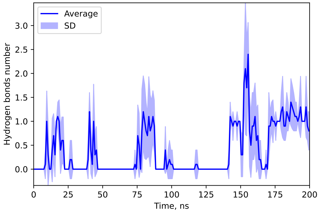
Hydrogen bonds number between 137644274 and SULF
