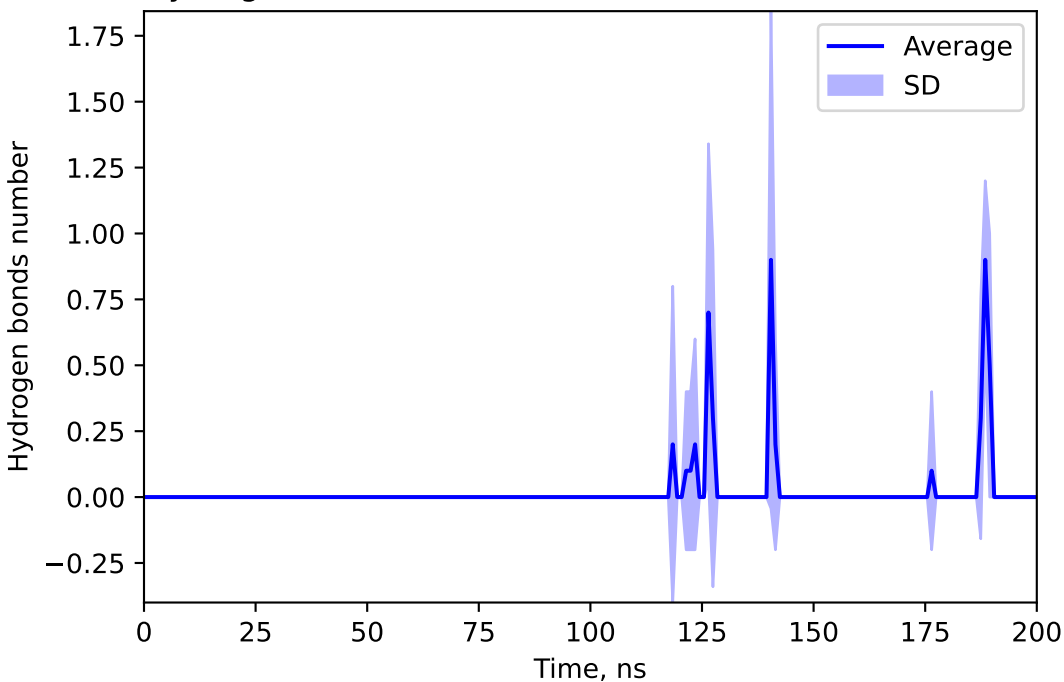
Hydrogen bonds number between 137644274 and SPIR
