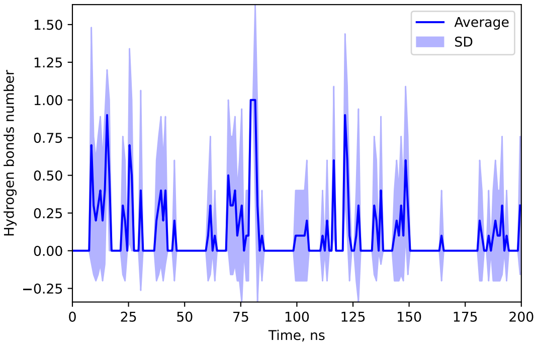
Hydrogen bonds number between 195797 and TILM
