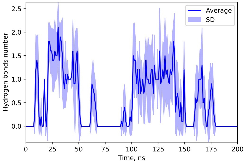
Hydrogen bonds number between 73293549 and SULF
