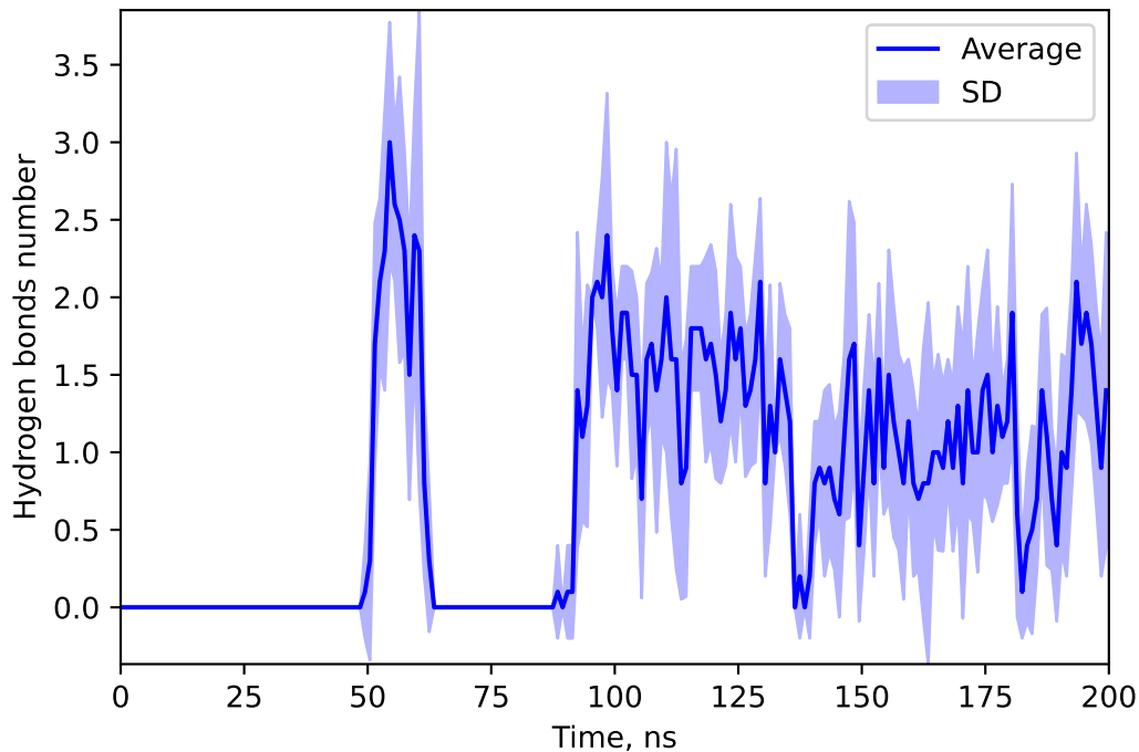
Hydrogen bonds number between 155518747 and DEME
