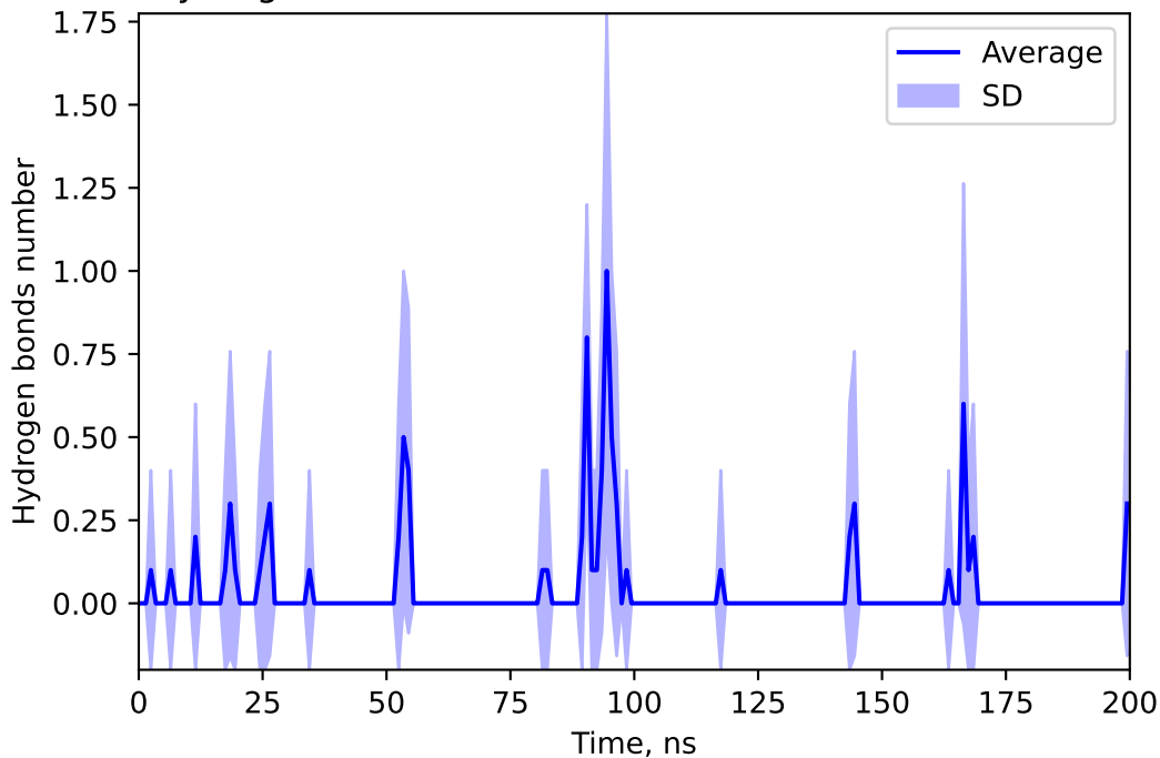
Hydrogen bonds number between 44569229 and SPIR
