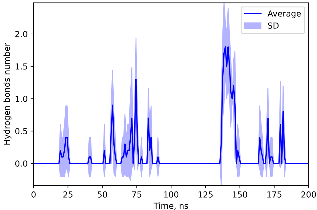
Hydrogen bonds number between 127034107 and SULF
