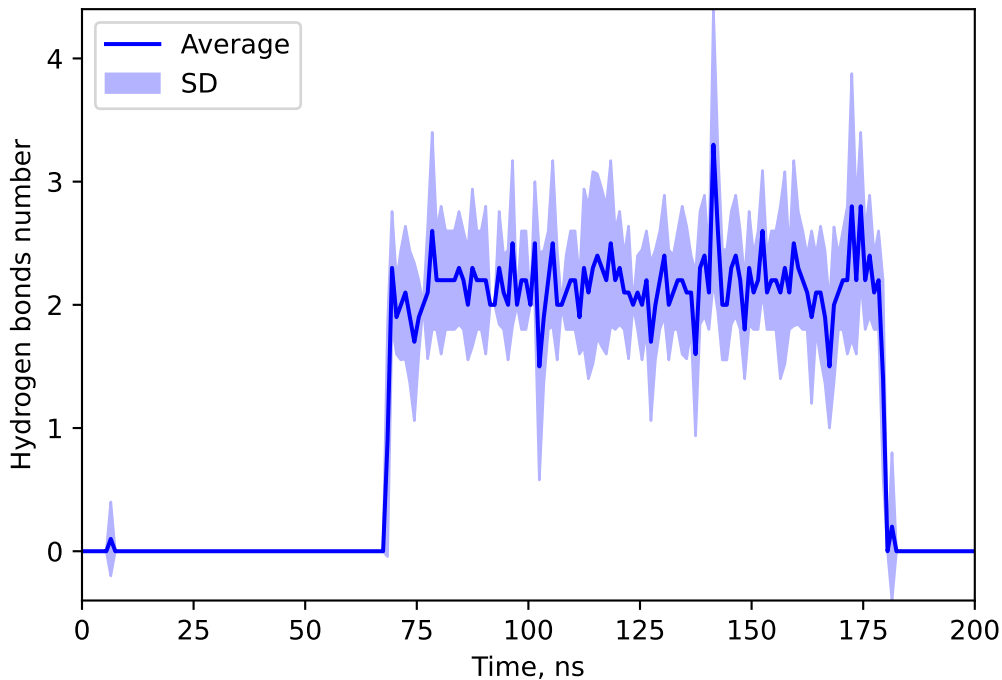
Hydrogen bonds number between 15559627 and STRE
