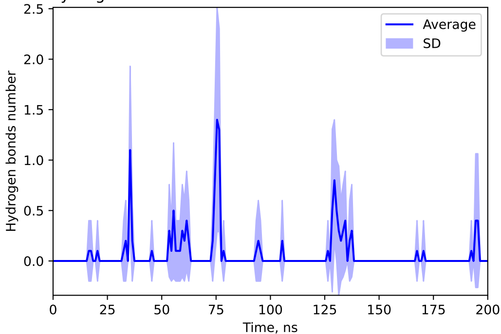
Hydrogen bonds number between 155514020 and DOXY
