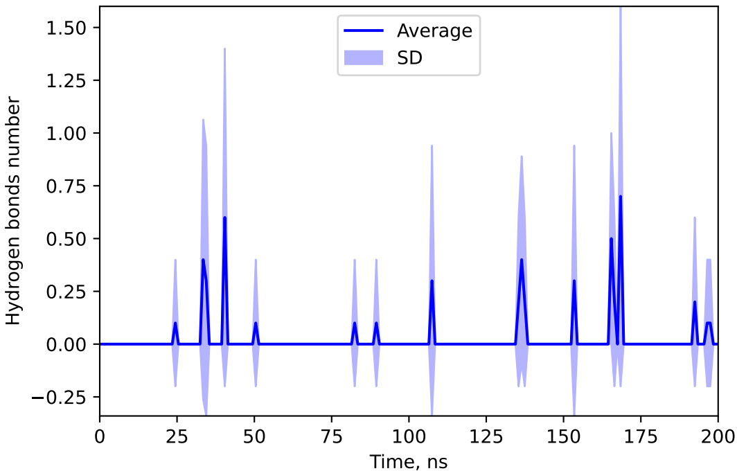
Hydrogen bonds number between 155514020 and RONI
