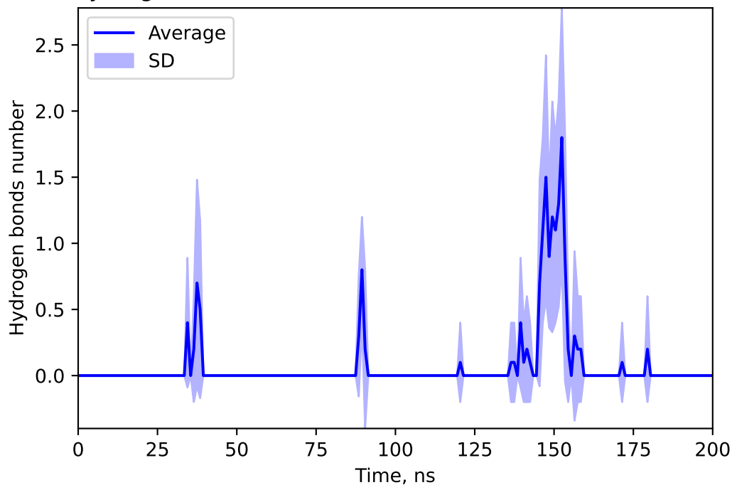
Hydrogen bonds number between 155559627 and DOXY
