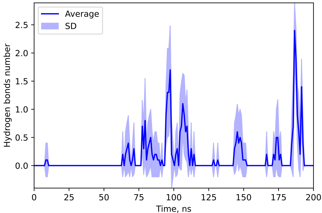
Hydrogen bonds number between 155559627 and SULF
