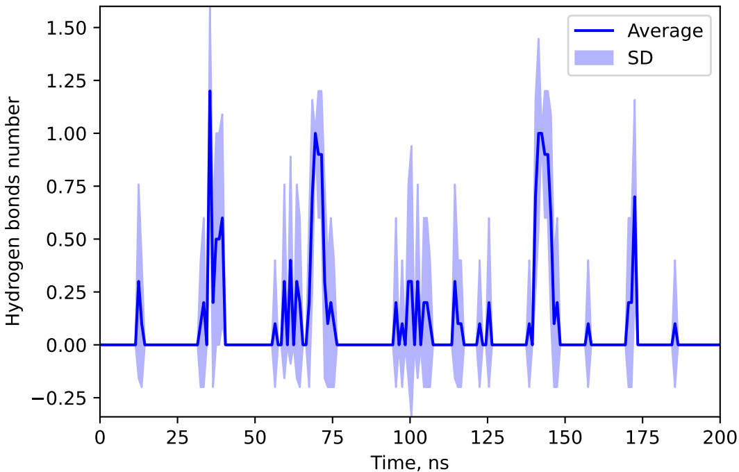
Hydrogen bonds number between 155521967 and DEME
