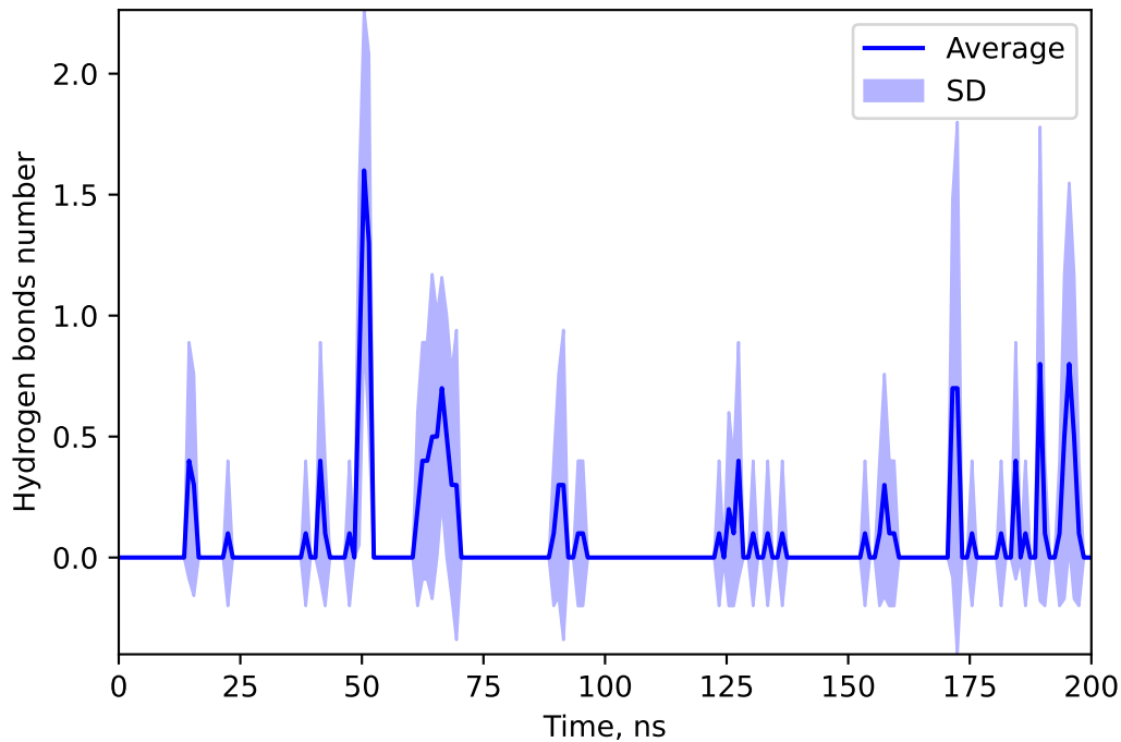
Hydrogen bonds number between 195797 and DANO
