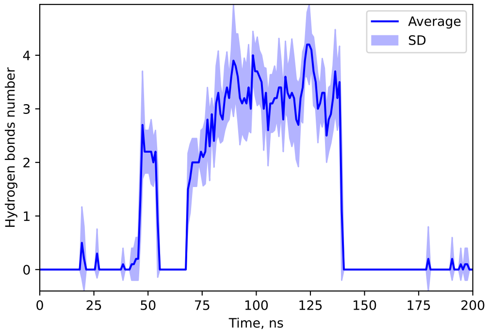
Hydrogen bonds number between 44569229 and STRE
