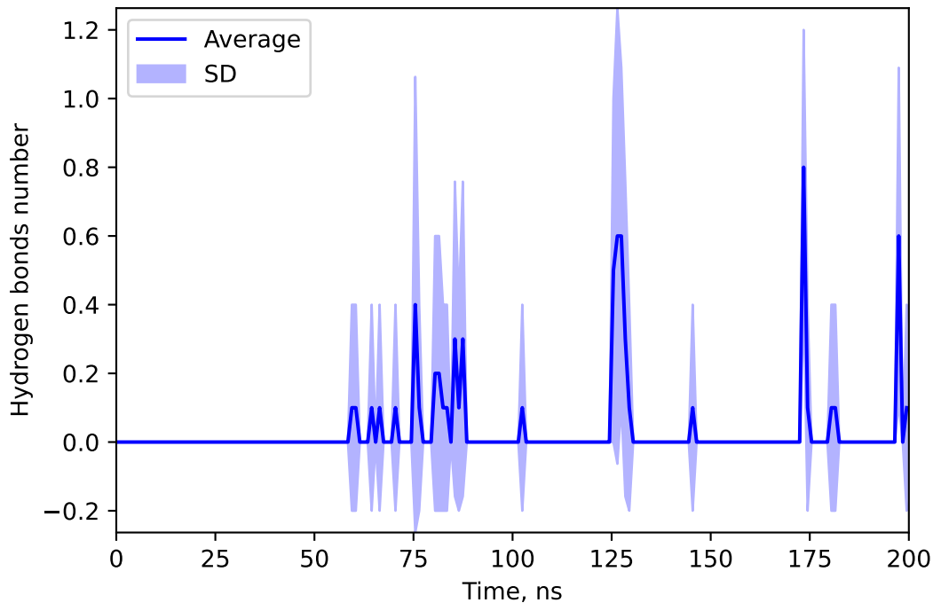
Hydrogen bonds number between 155514020 and DANO
