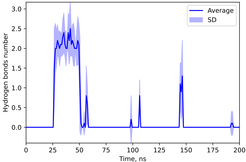
Hydrogen bonds number between 145975502 and STRE
