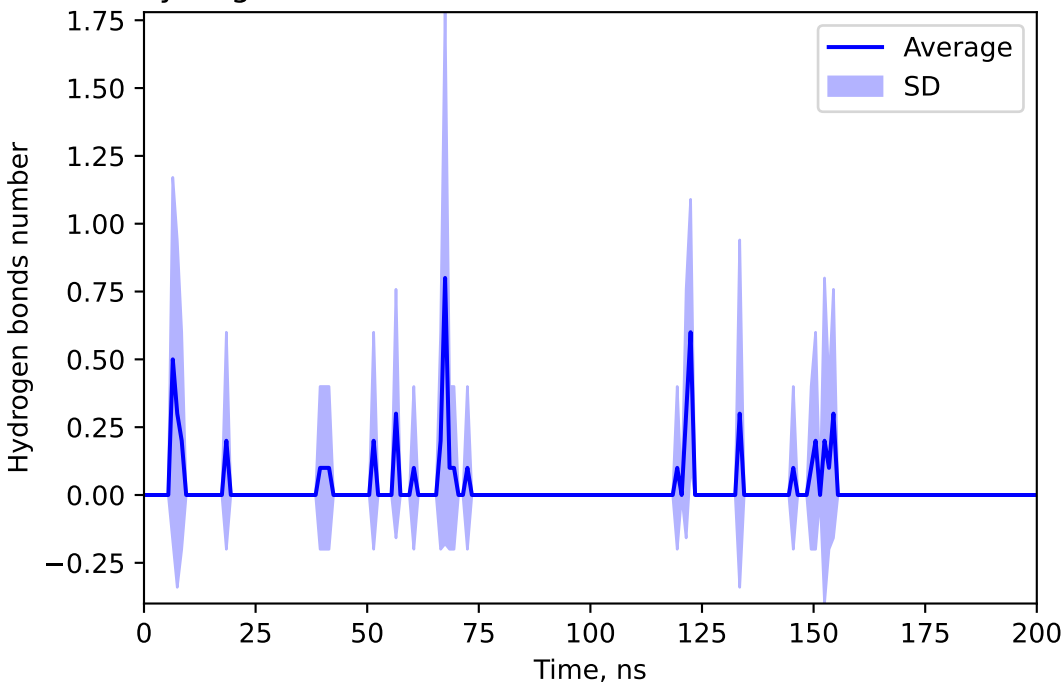
Hydrogen bonds number between 166625339 and METR
