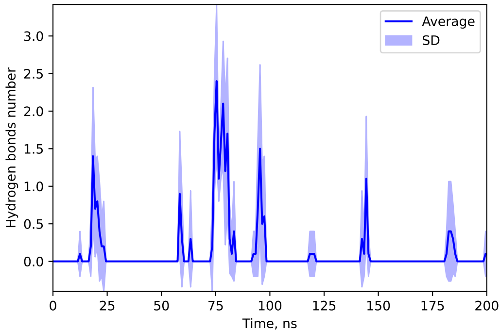
Hydrogen bonds number between 155559627 and CEFA
