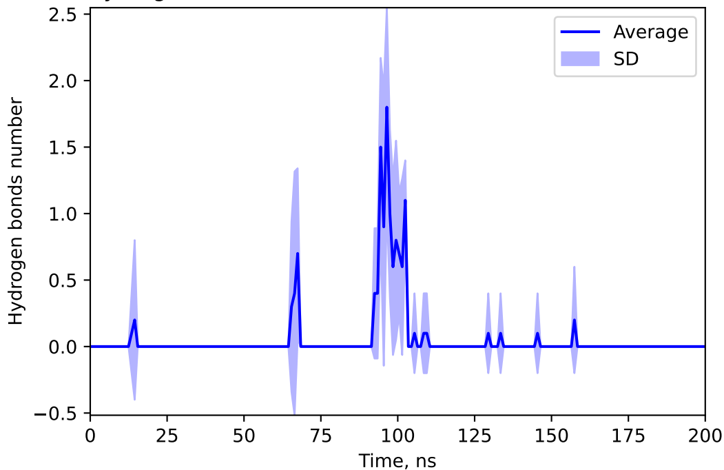
Hydrogen bonds number between 145975502 and RONI
