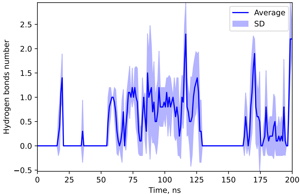
Hydrogen bonds number between 73293549 and DEME
