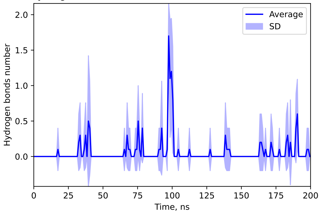
Hydrogen bonds number between 145975502 and DANO
