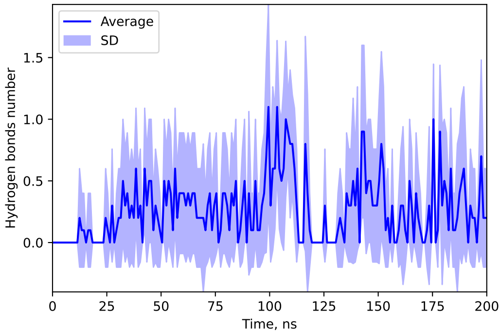
Hydrogen bonds number between 44569229 and DEME
