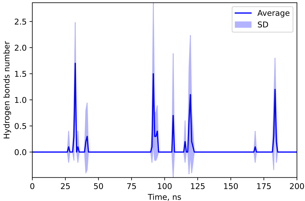
Hydrogen bonds number between 44569229 and RONI
