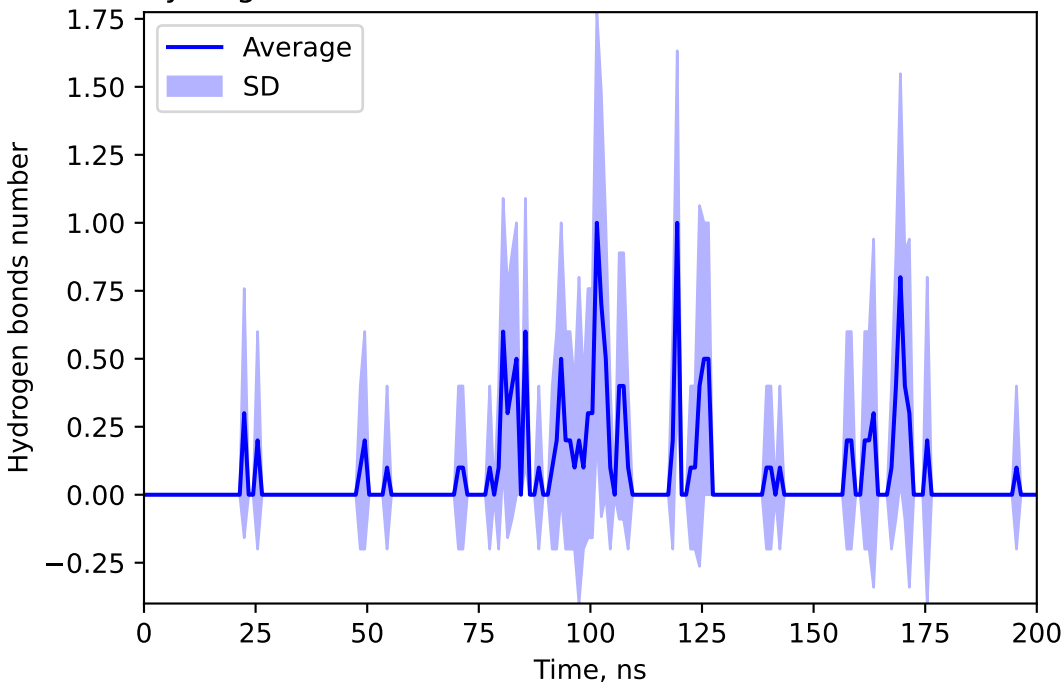
Hydrogen bonds number between 137644274 and TIAM
