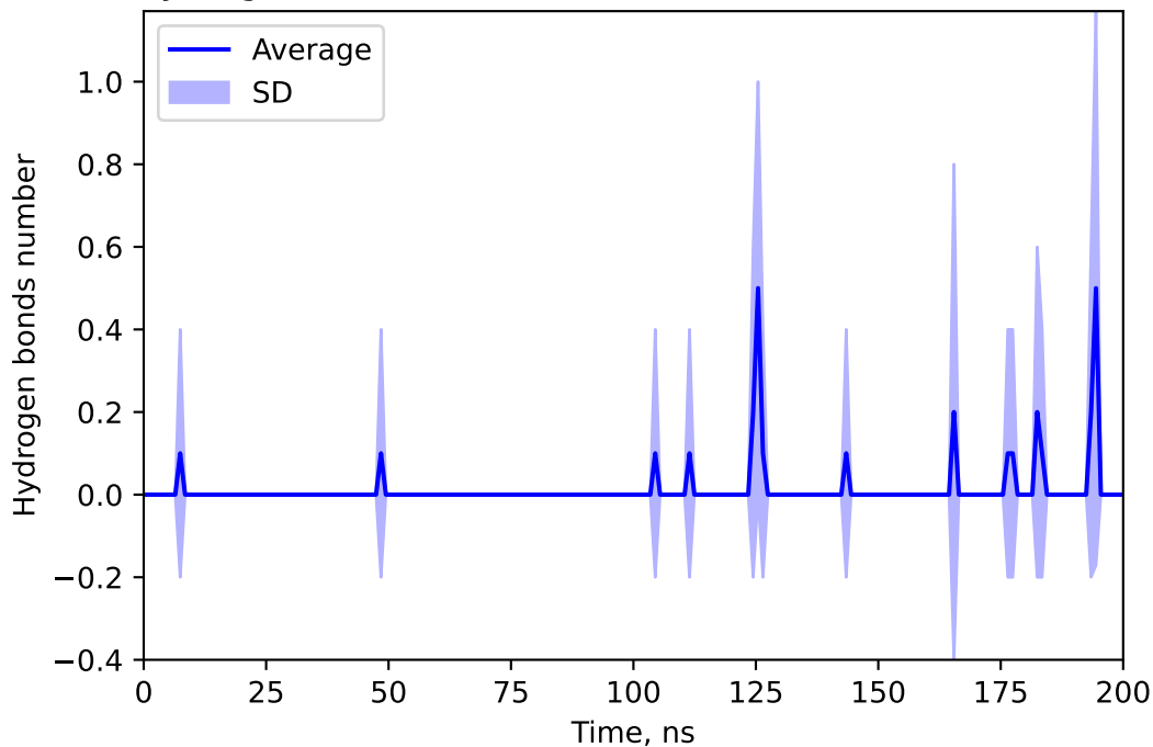
Hydrogen bonds number between 166625339 and DOXY
