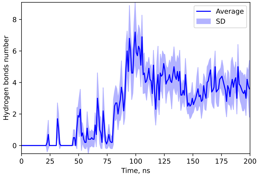
Hydrogen bonds number between 145975502 and CEFA
