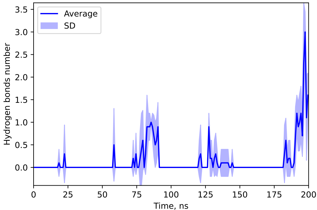
Hydrogen bonds number between 137646969 and DEME
