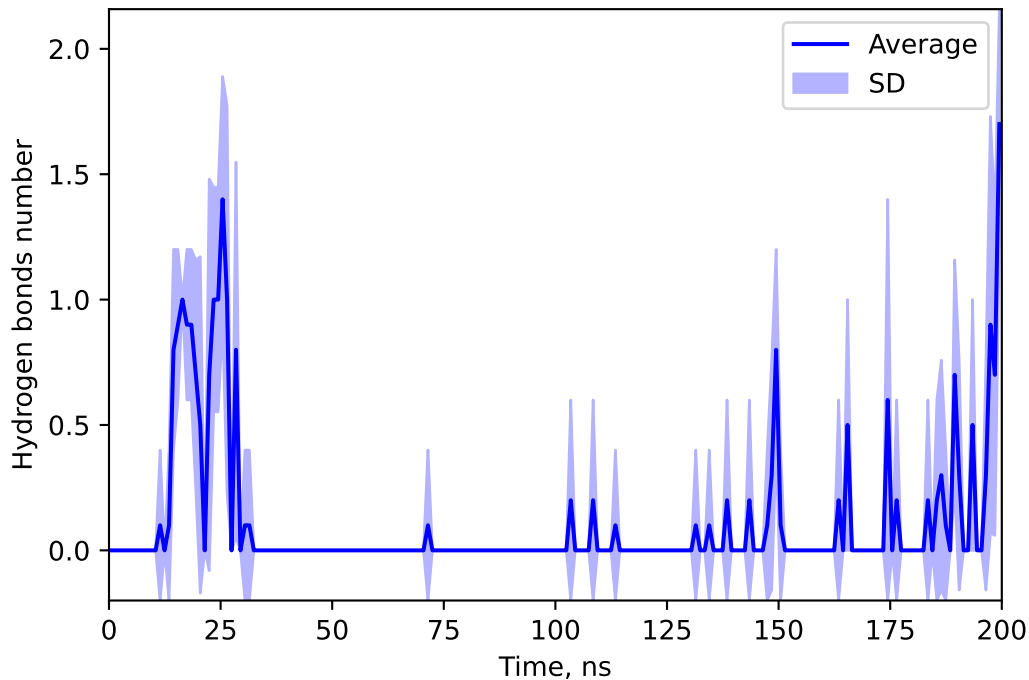
Hydrogen bonds number between 166625339 and TIAM
