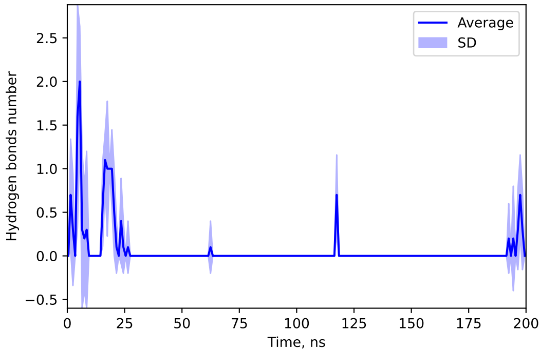
Hydrogen bonds number between 155521967 and CEFA
