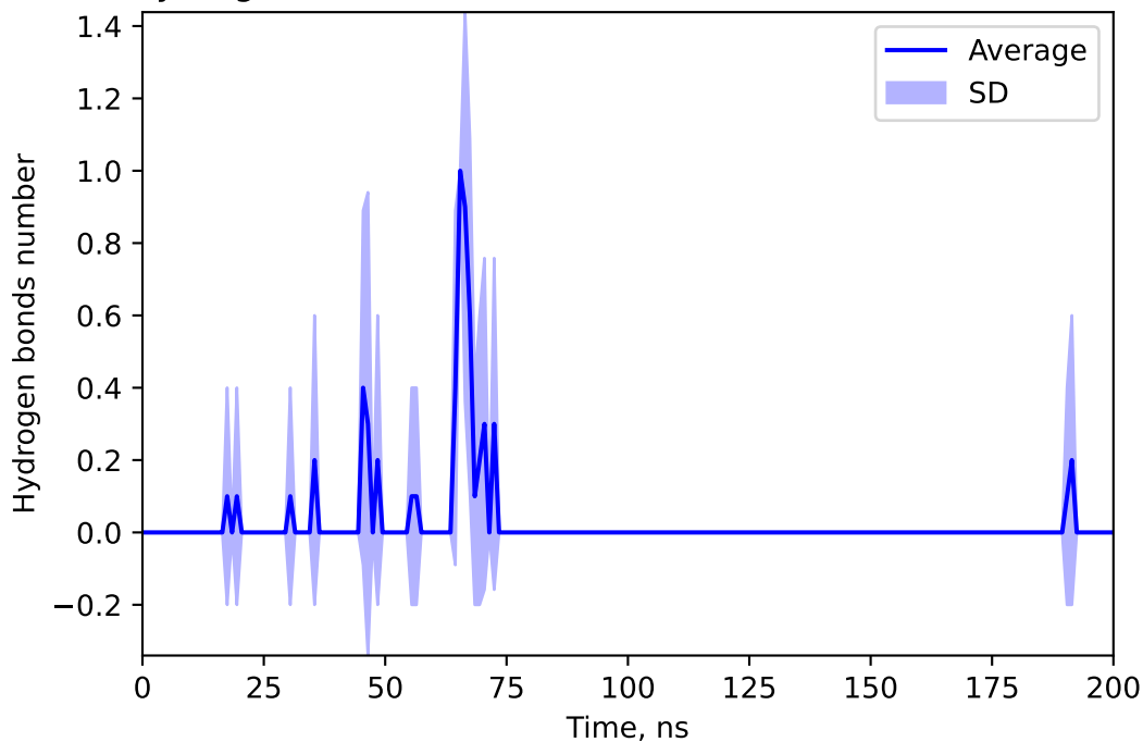
Hydrogen bonds number between 155557444 and DANO
