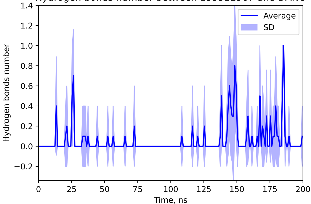
Hydrogen bonds number between 155521967 and DANO
