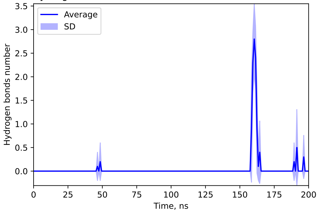
Hydrogen bonds number between 137646969 and LYNC
