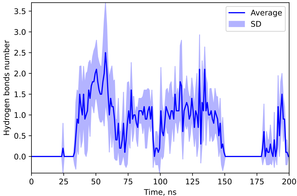
Hydrogen bonds number between 155518747 and SULF
