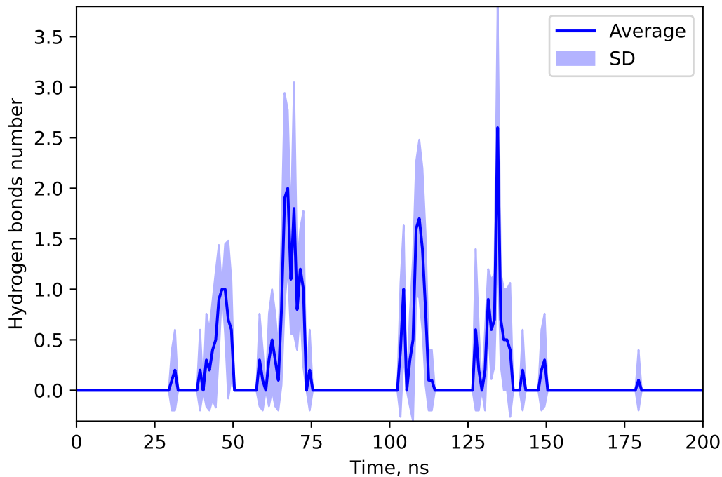
Hydrogen bonds number between 127034107 and DEME
