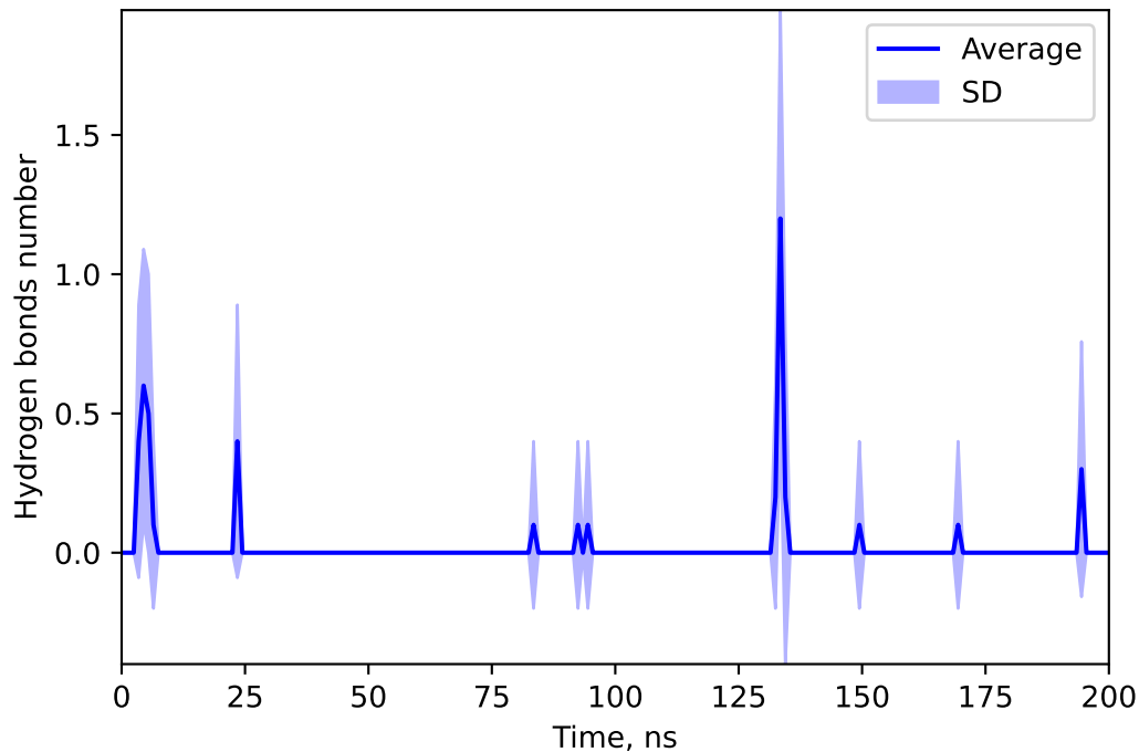
Hydrogen bonds number between 155514020 and METR
