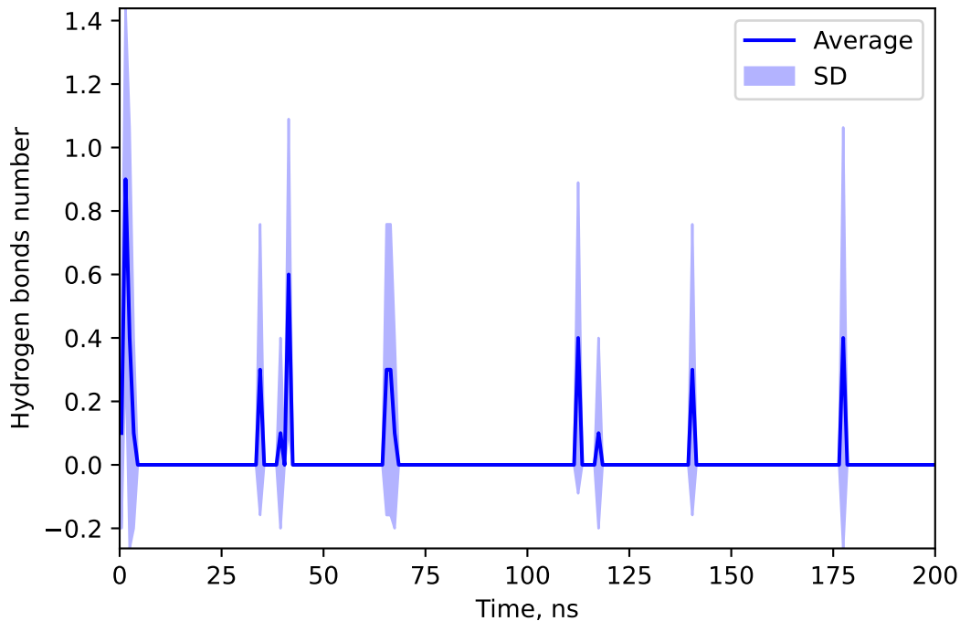
Hydrogen bonds number between 137646969 and TILM
