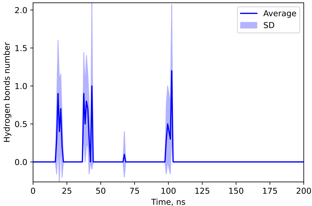
Hydrogen bonds number between 73293549 and DOXY
