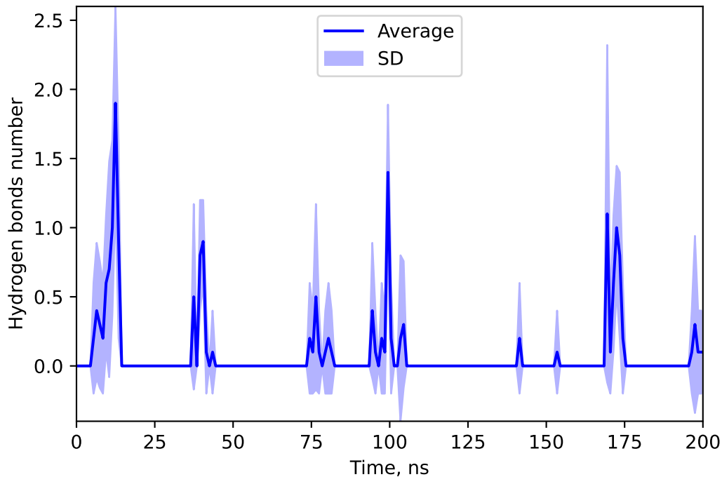
Hydrogen bonds number between 137644274 and LYNC
