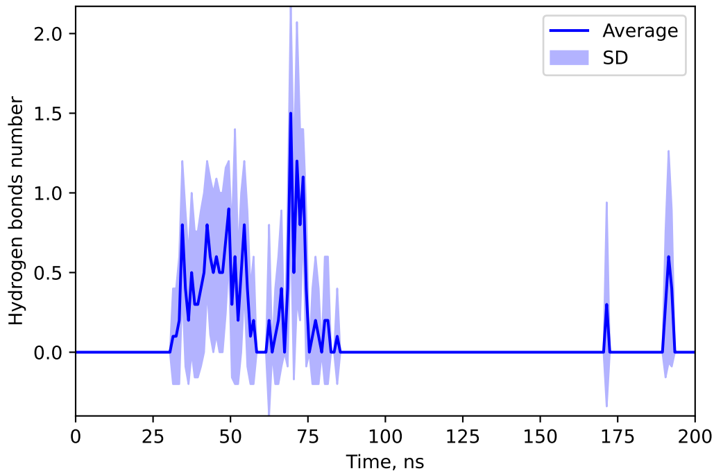
Hydrogen bonds number between 73293549 and TIAM
