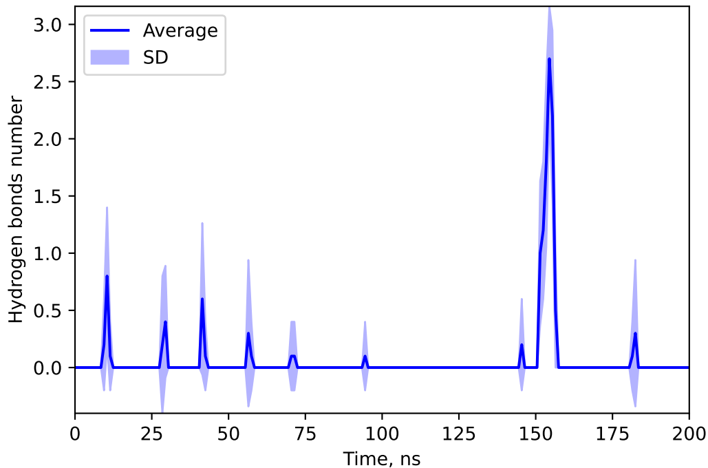
Hydrogen bonds number between 166625339 and RONI
