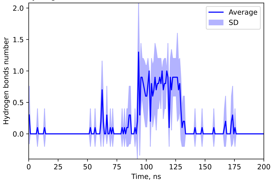
Hydrogen bonds number between 166625339 and DANO
