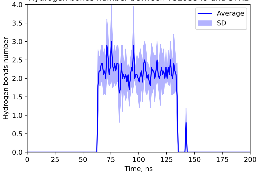
Hydrogen bonds number between 73293549 and STRE
