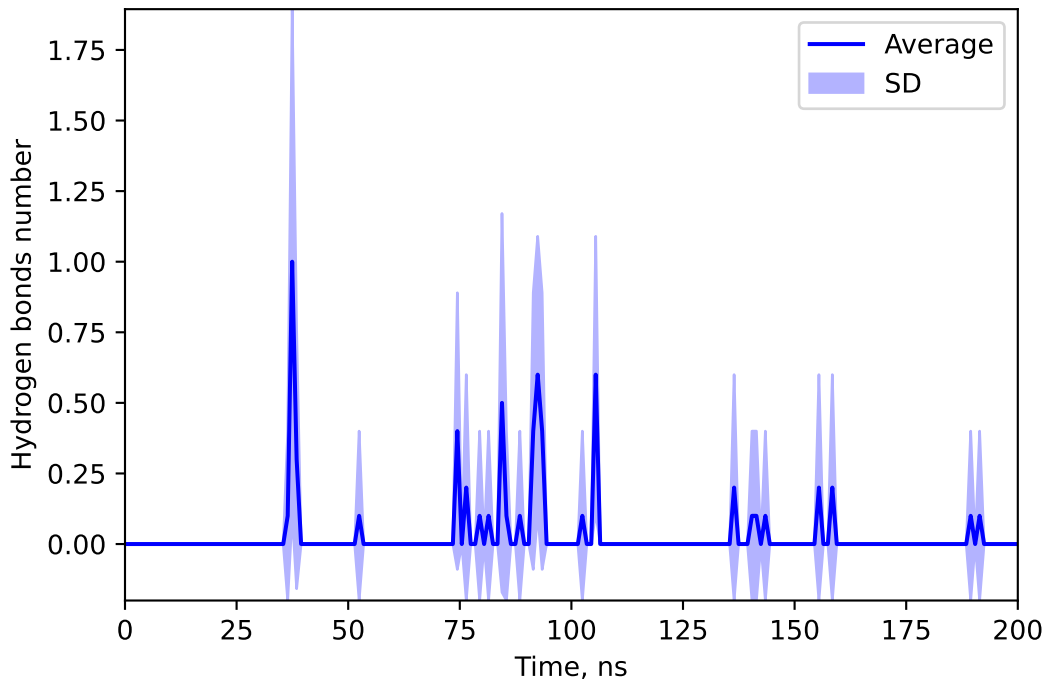
Hydrogen bonds number between 137646969 and TIAM
