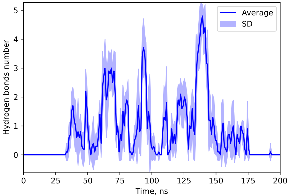
Hydrogen bonds number between 145975502 and DEME
