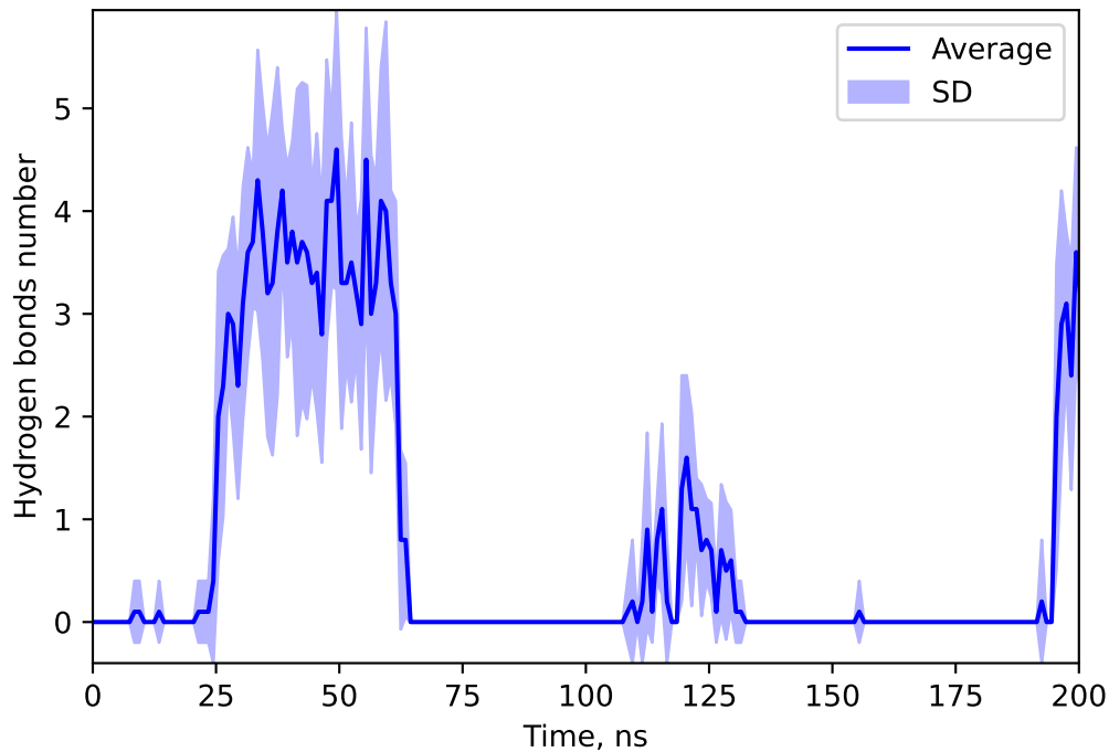
Hydrogen bonds number between 127034107 and CEFA
