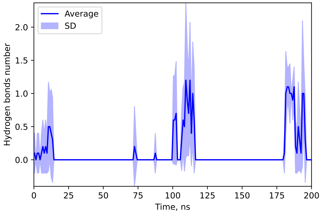
Hydrogen bonds number between 44575206 and DOXY
