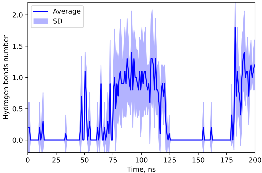
Hydrogen bonds number between 44575206 and SPIR
