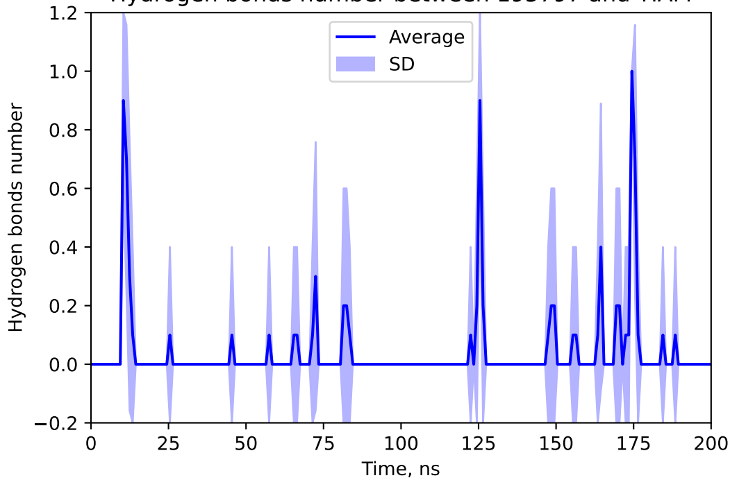
Hydrogen bonds number between 195797 and TIAM
