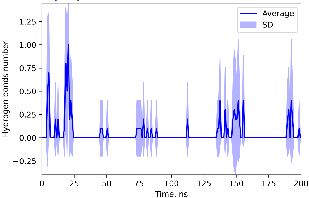
Hydrogen bonds number between 195797 and DEME
