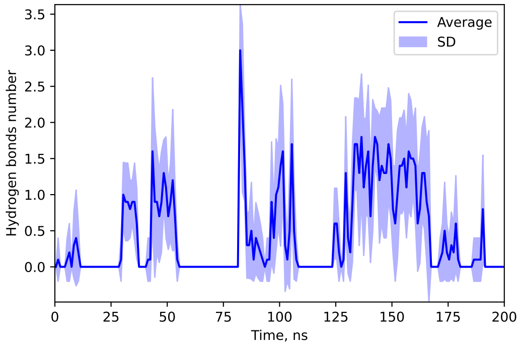
Hydrogen bonds number between 155559627 and DEME
