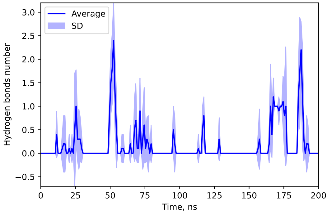
Hydrogen bonds number between 195797 and CEFA
