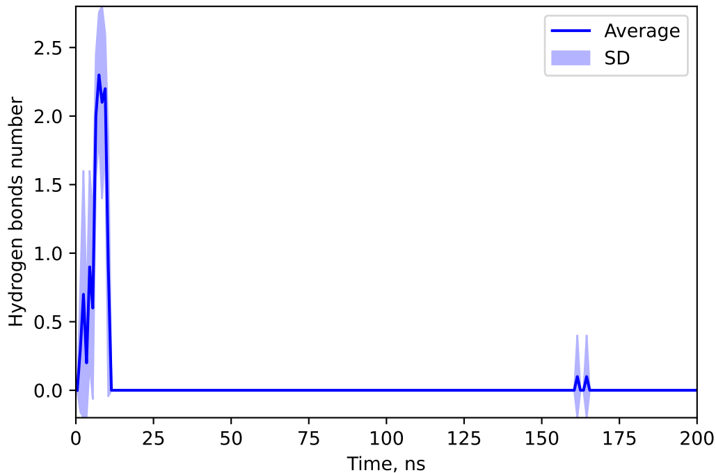
Hydrogen bonds number between 155518747 and STRE
