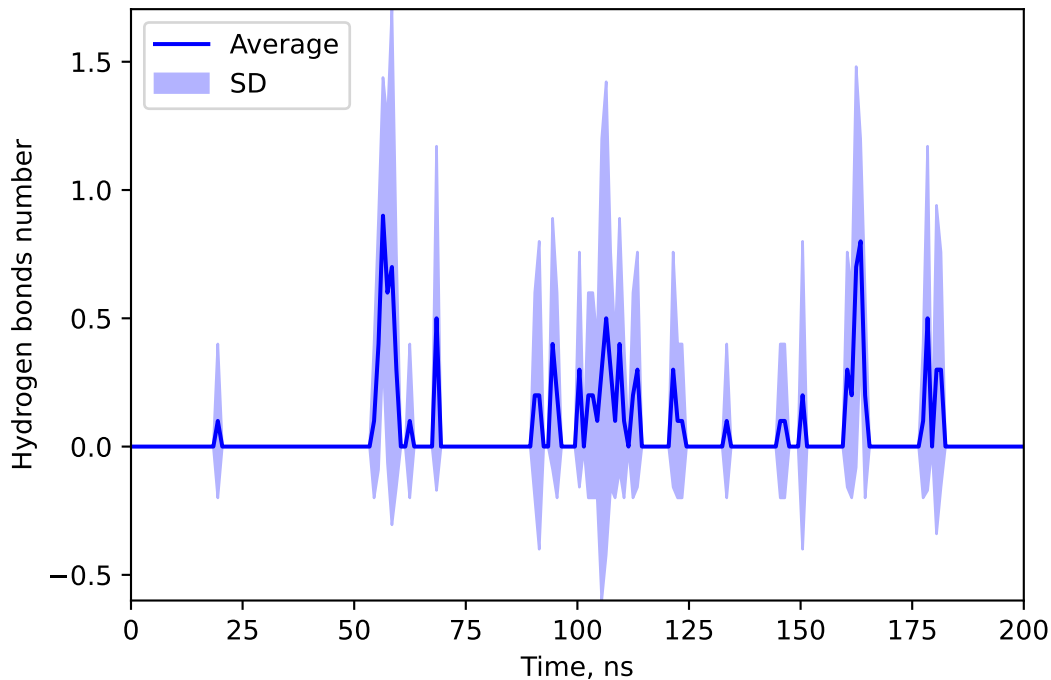
Hydrogen bonds number between 195797 and STRE
