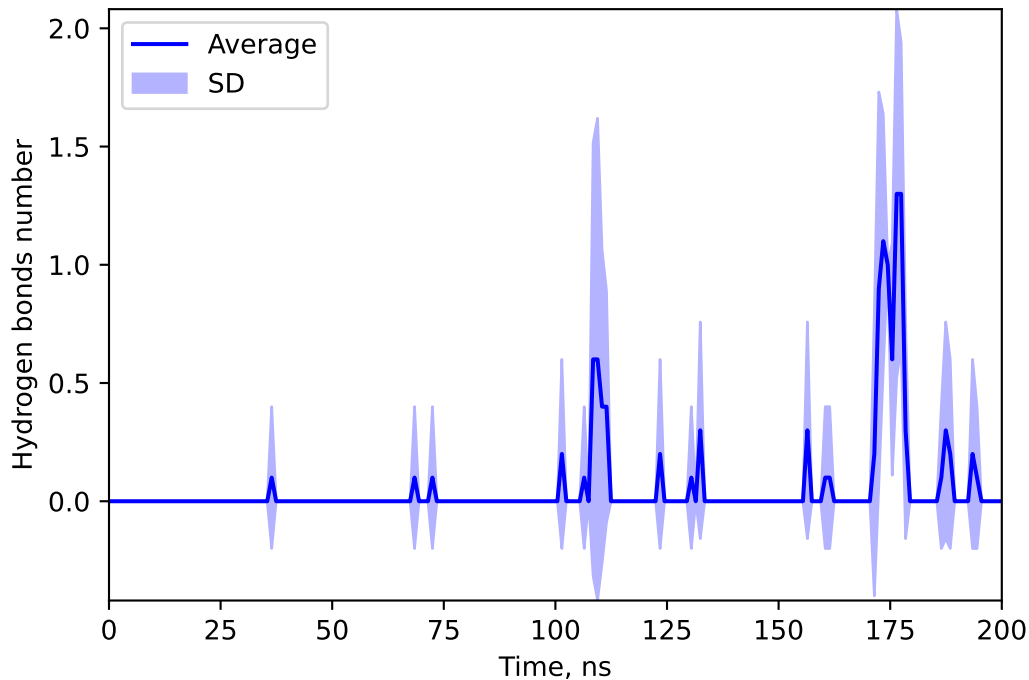
Hydrogen bonds number between 195797 and SPIR
