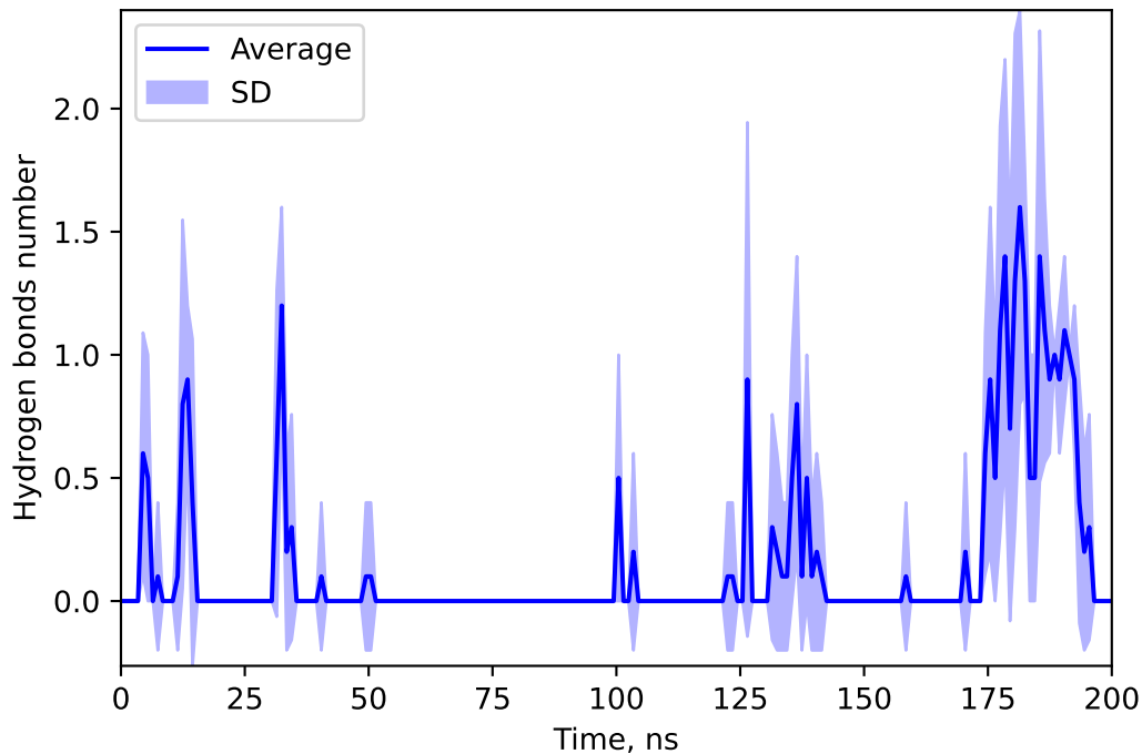
Hydrogen bonds number between 166625339 and SPIR
