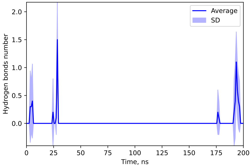
Hydrogen bonds number between 166625339 and STRE
