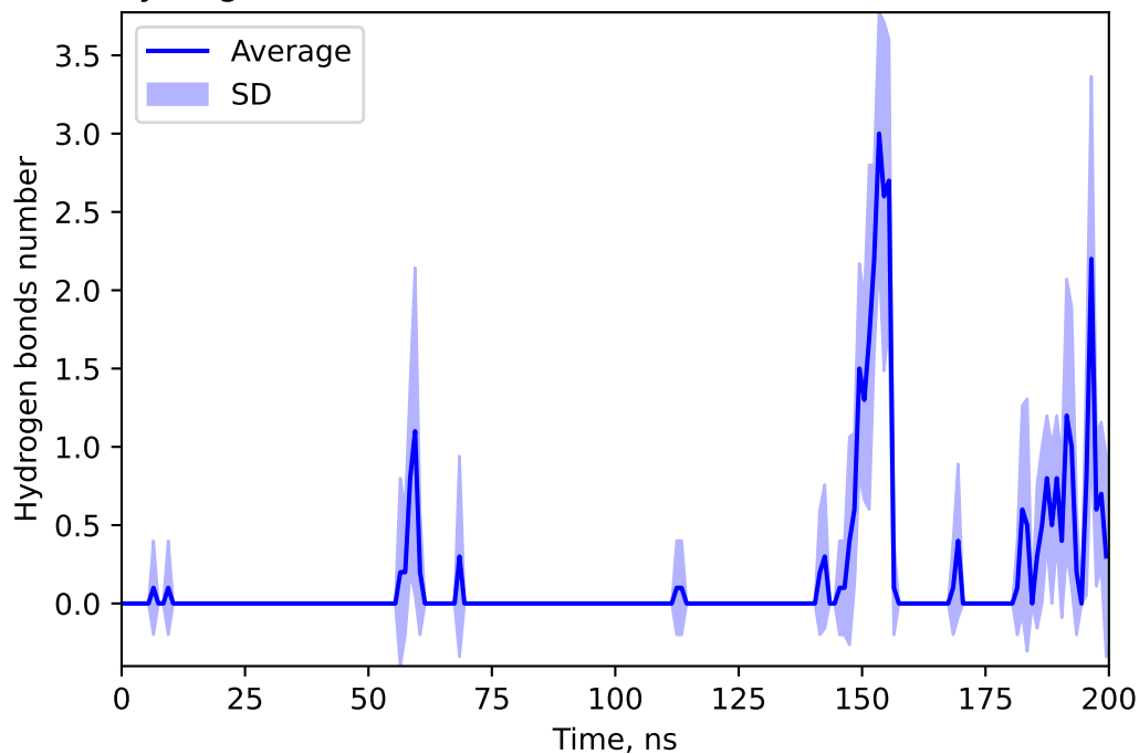
Hydrogen bonds number between 137646969 and DOXY
