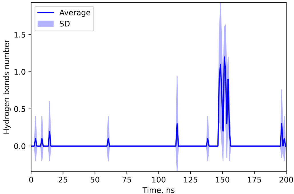
Hydrogen bonds number between 155559627 and METR
