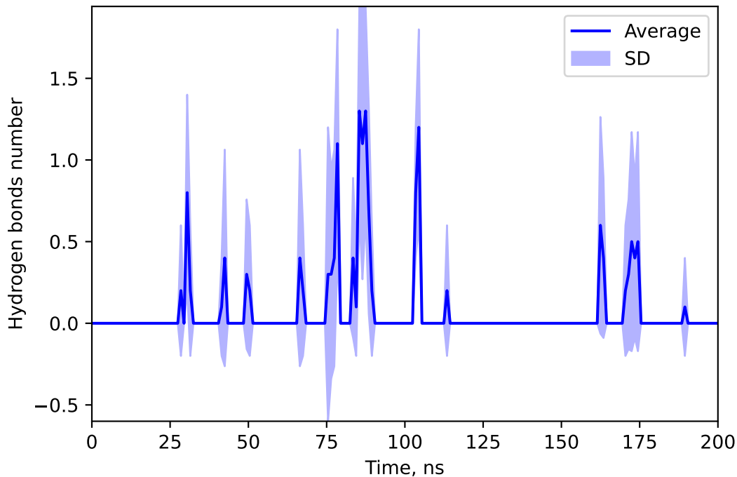
Hydrogen bonds number between 137644274 and METR
