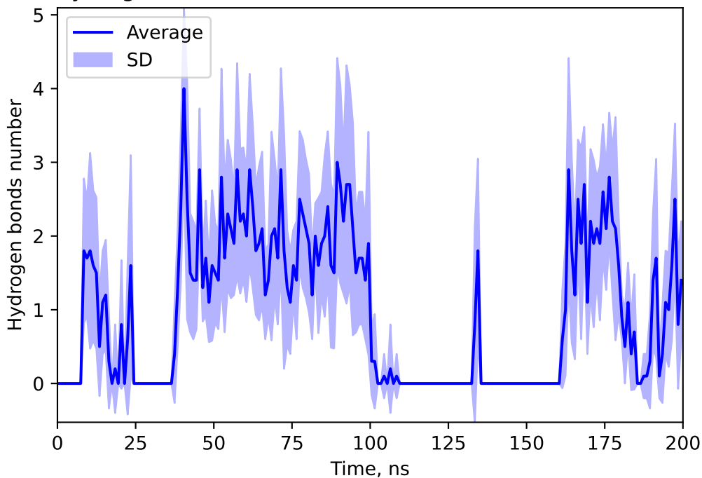
Hydrogen bonds number between 166625339 and CEFA
