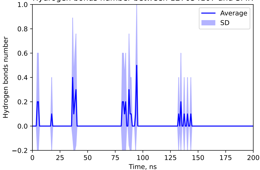
Hydrogen bonds number between 127034107 and SPIR
