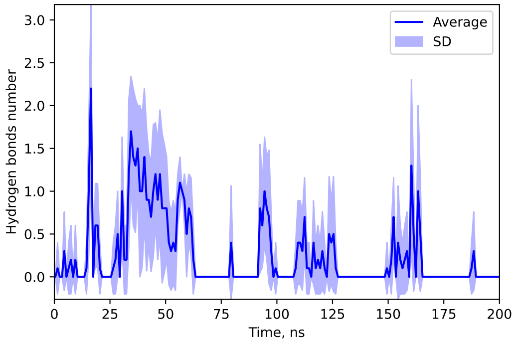
Hydrogen bonds number between 195797 and SULF
