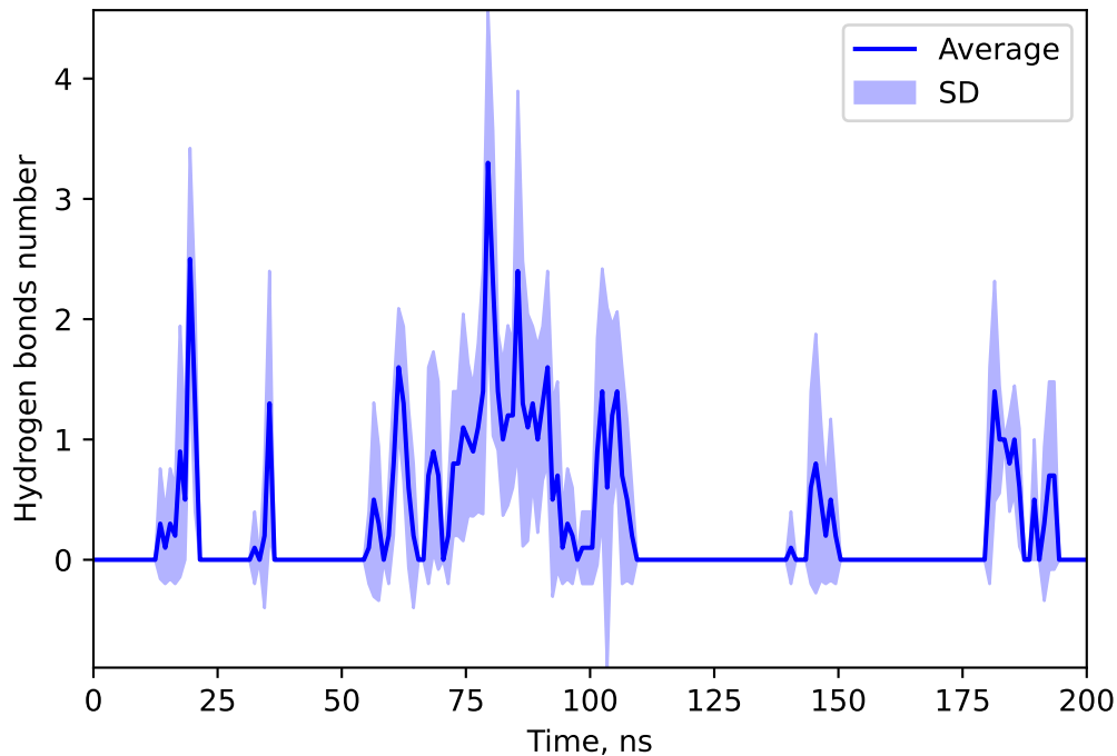
Hydrogen bonds number between 137646969 and CEFA
