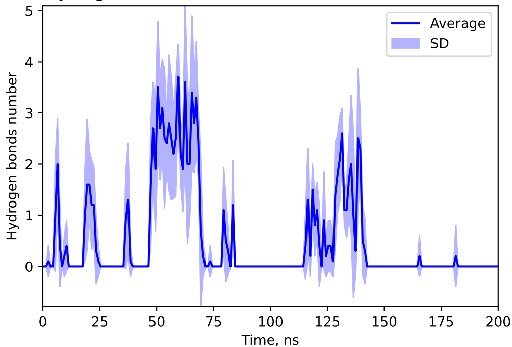
Hydrogen bonds number between 44575206 and CEFA
