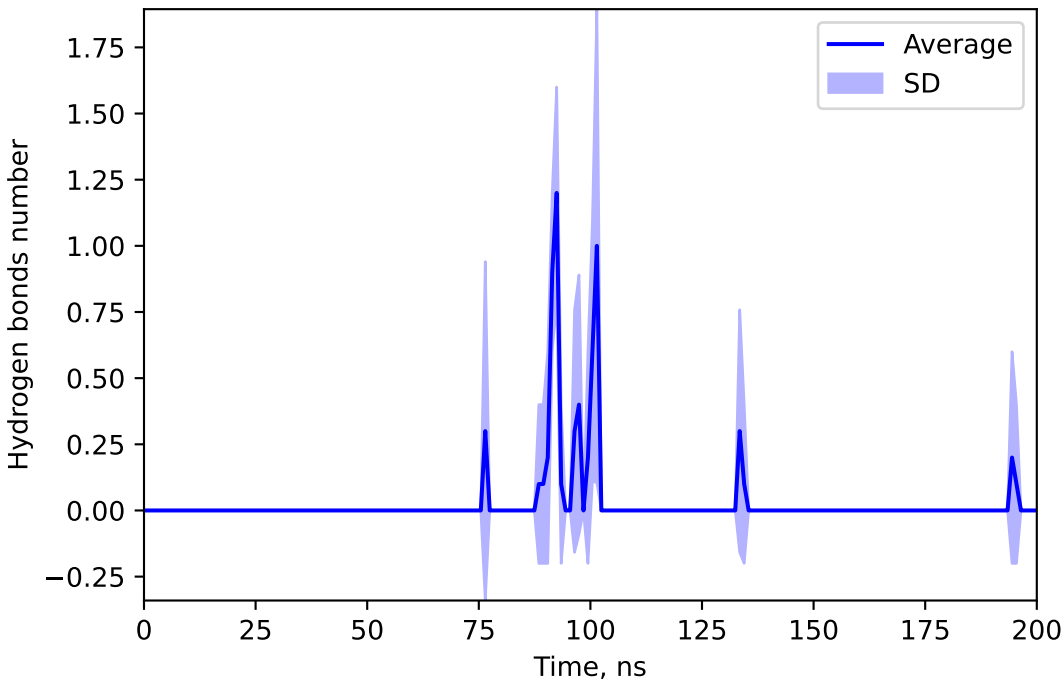
Hydrogen bonds number between 155557444 and LYNC
