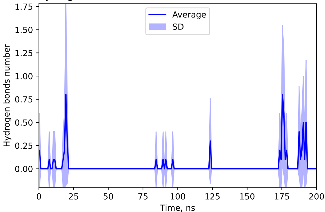
Hydrogen bonds number between 155514020 and SULF
