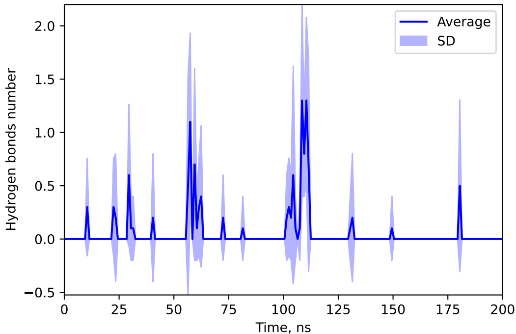
Hydrogen bonds number between 145975502 and METR
