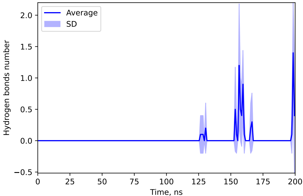
Hydrogen bonds number between 137644274 and DOXY
