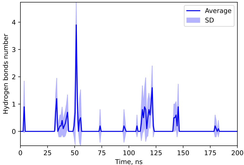
Hydrogen bonds number between 145975502 and LYNC
