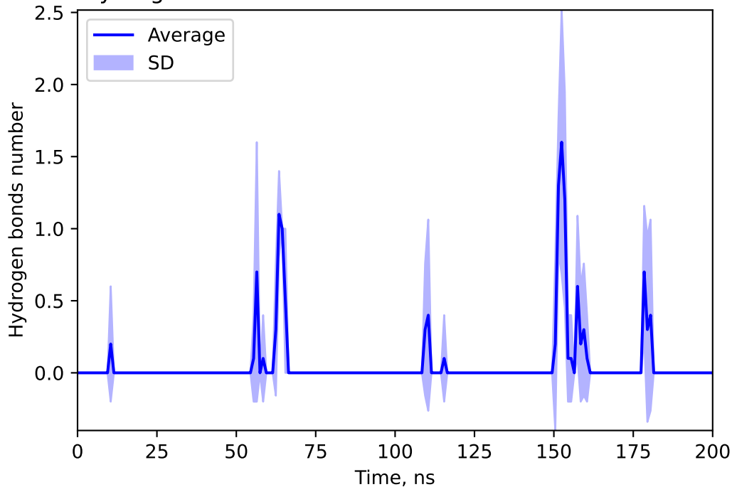
Hydrogen bonds number between 44569229 and LYNC
