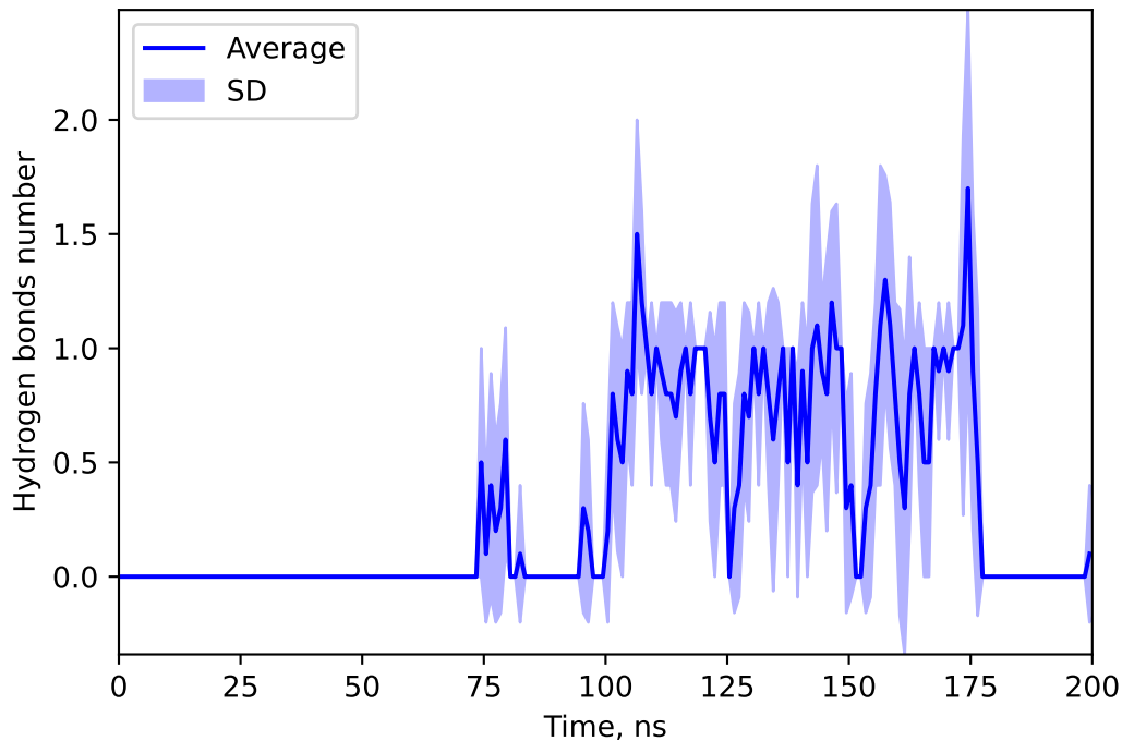
Hydrogen bonds number between 73293549 and TILM
