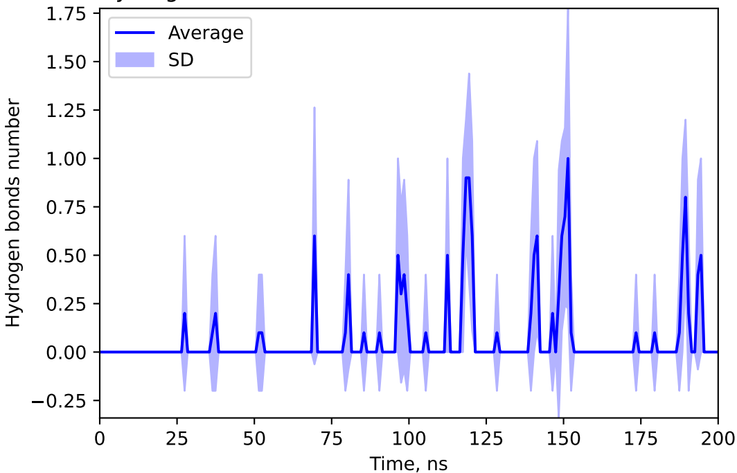
Hydrogen bonds number between 44575206 and DANO
