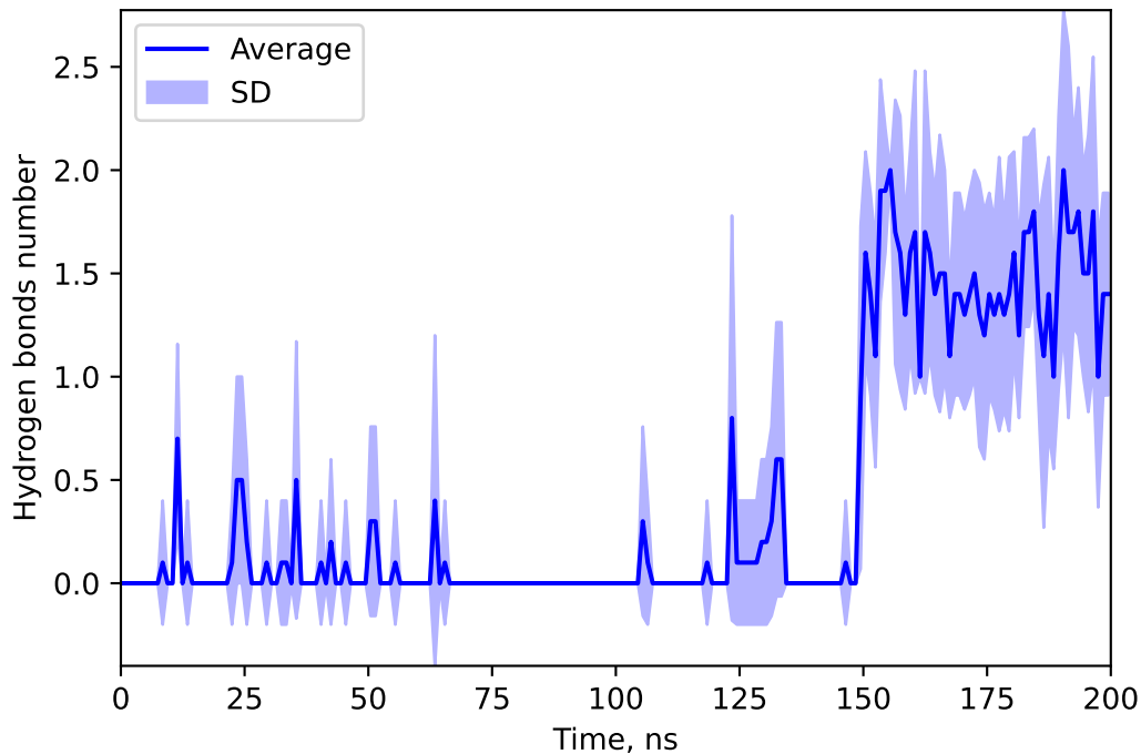
Hydrogen bonds number between 155518747 and DANO
