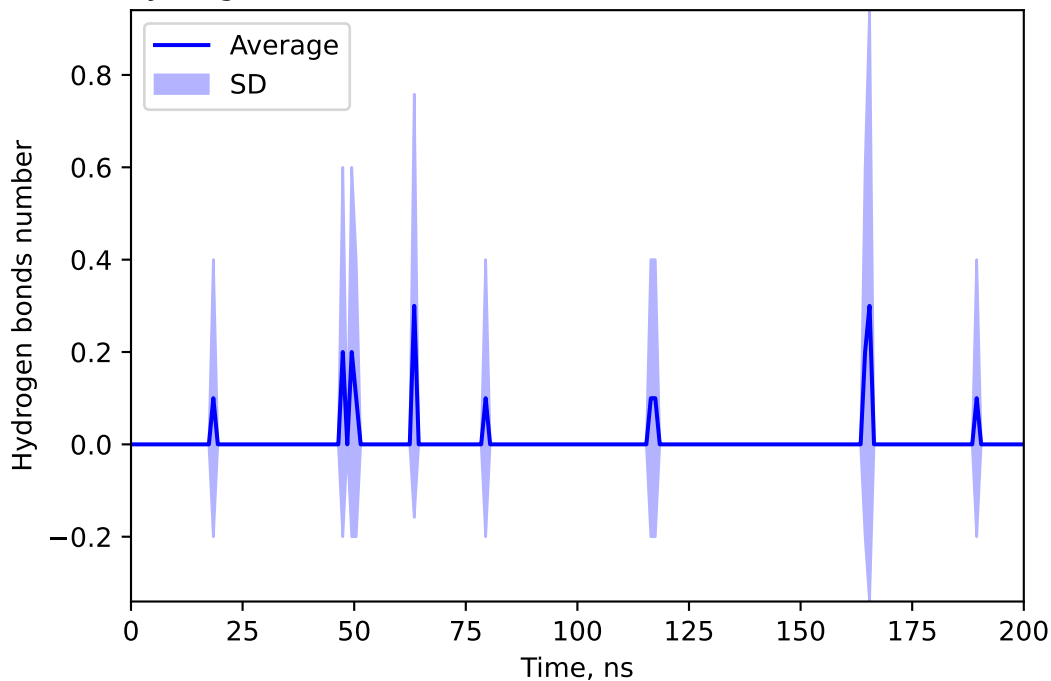
Hydrogen bonds number between 137646969 and METR
