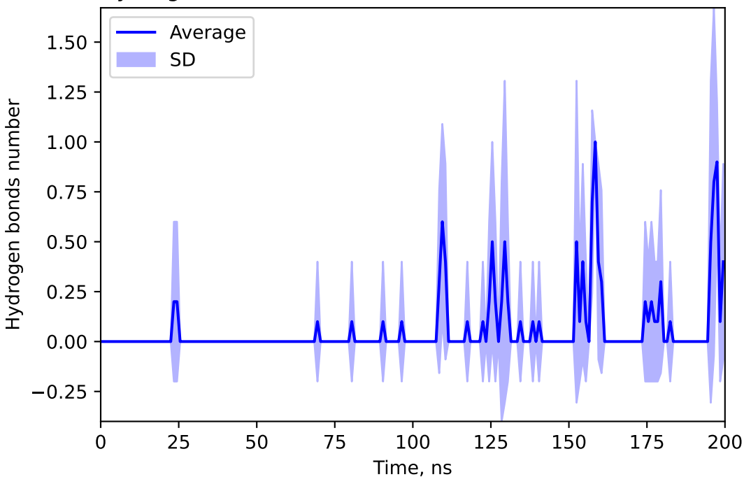
Hydrogen bonds number between 166625339 and TILM
