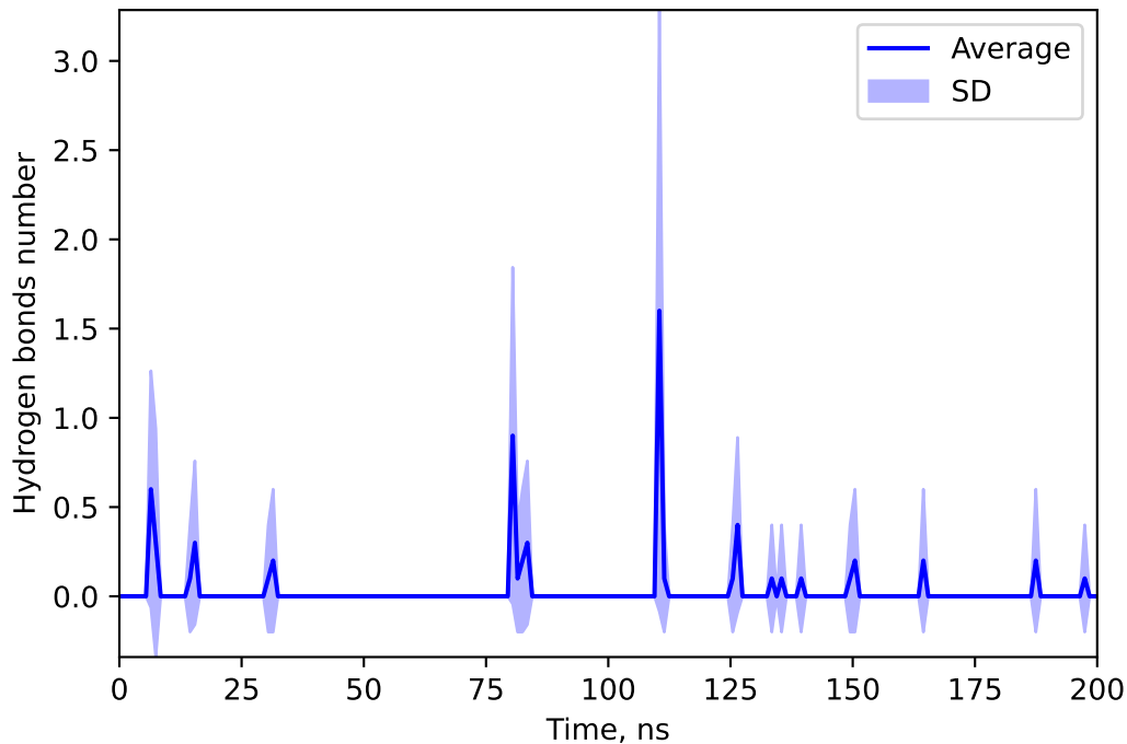
Hydrogen bonds number between 127034107 and METR
