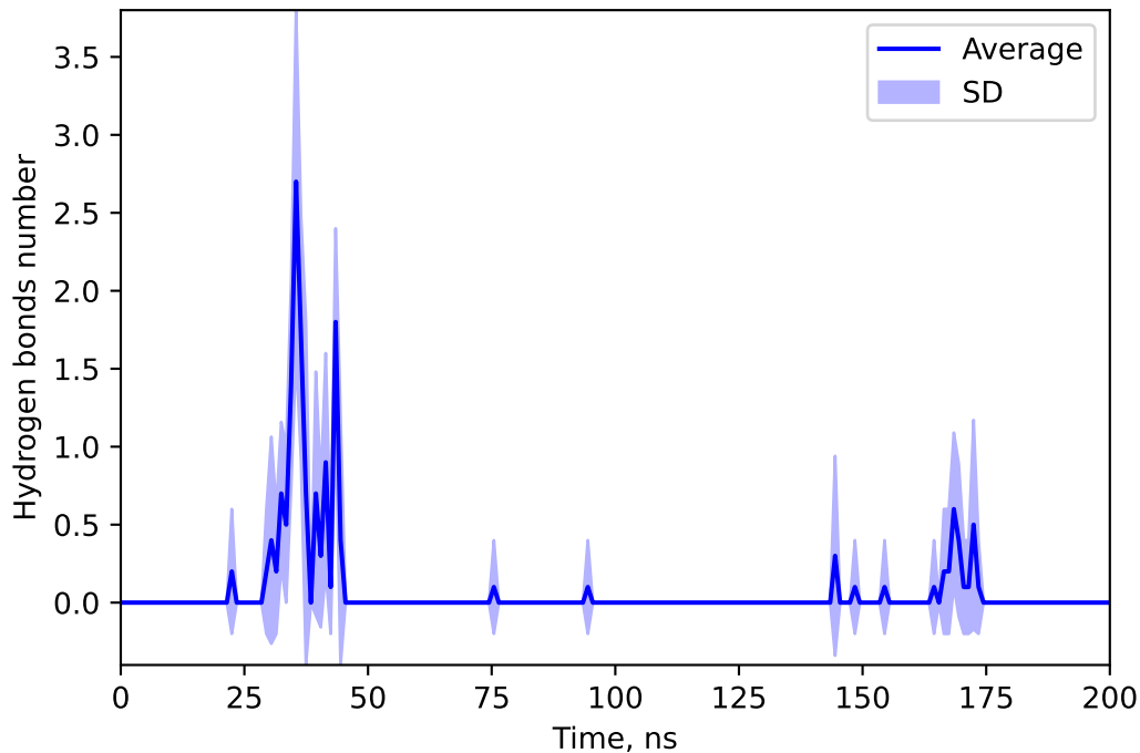
Hydrogen bonds number between 155559627 and TILM
