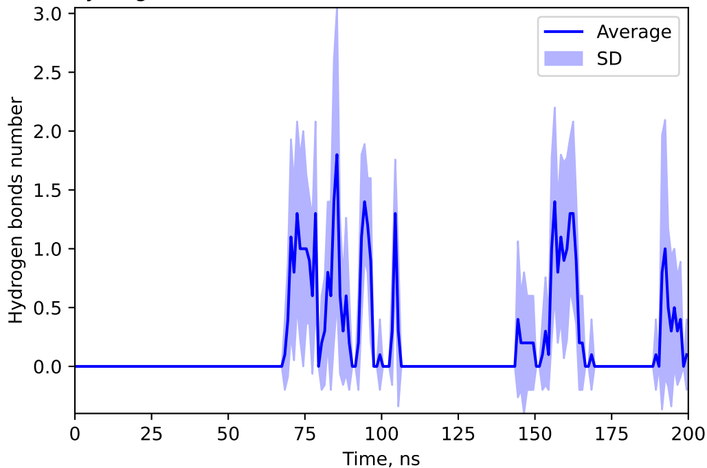
Hydrogen bonds number between 145975502 and DOXY
