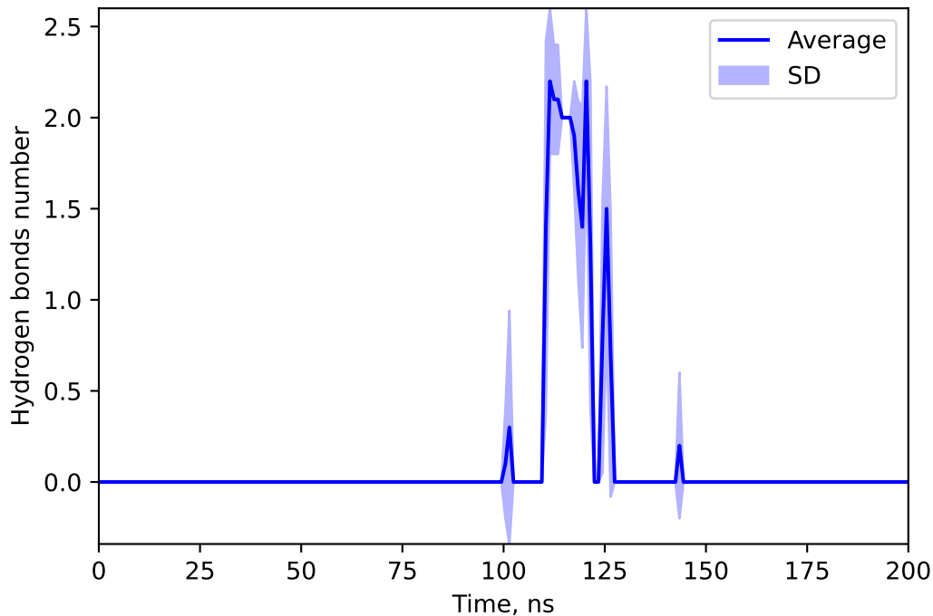
Hydrogen bonds number between 44575206 and STRE
