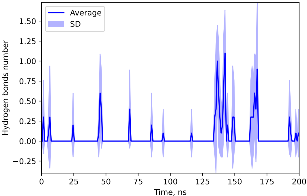
Hydrogen bonds number between 44569229 and DOXY
