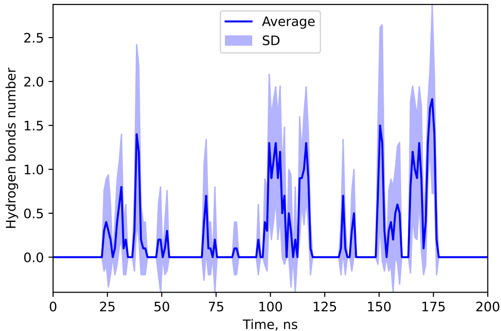
Hydrogen bonds number between 137646969 and SULF
