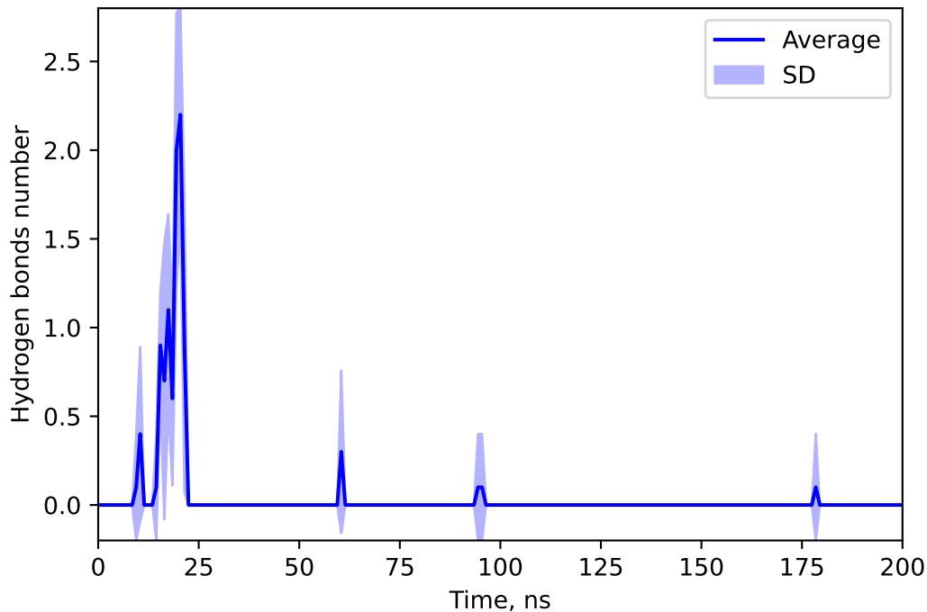
Hydrogen bonds number between 155521967 and TILM
