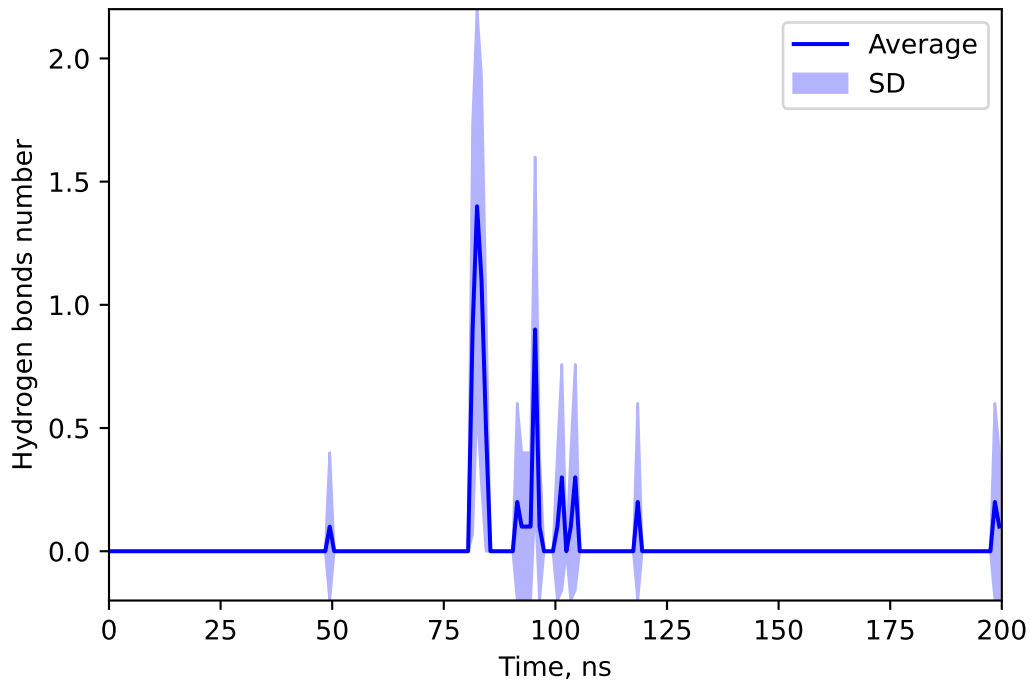
Hydrogen bonds number between 137646969 and SPIR
