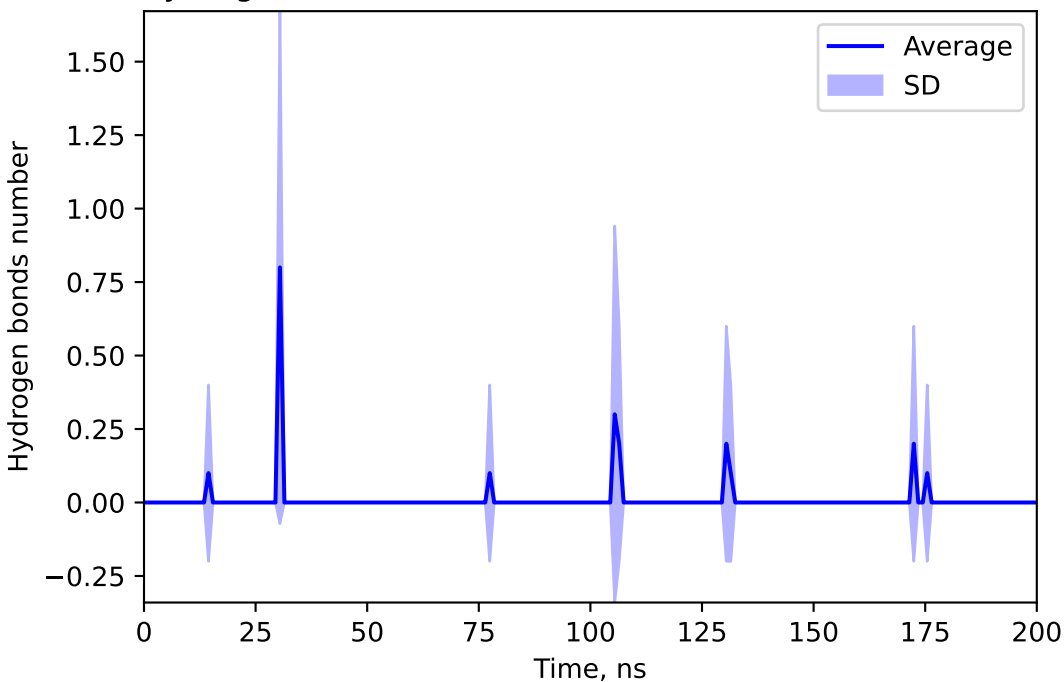
Hydrogen bonds number between 155557444 and RONI
