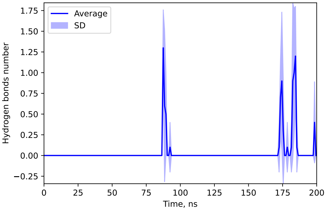
Hydrogen bonds number between 73293549 and SPIR
