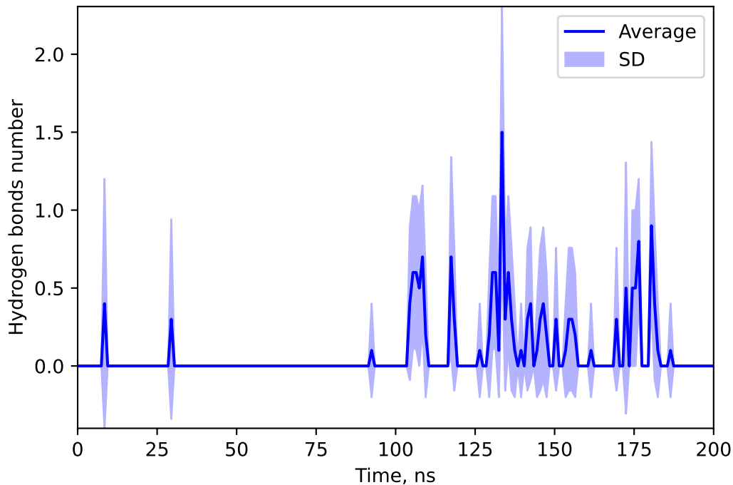
Hydrogen bonds number between 137644274 and TILM
