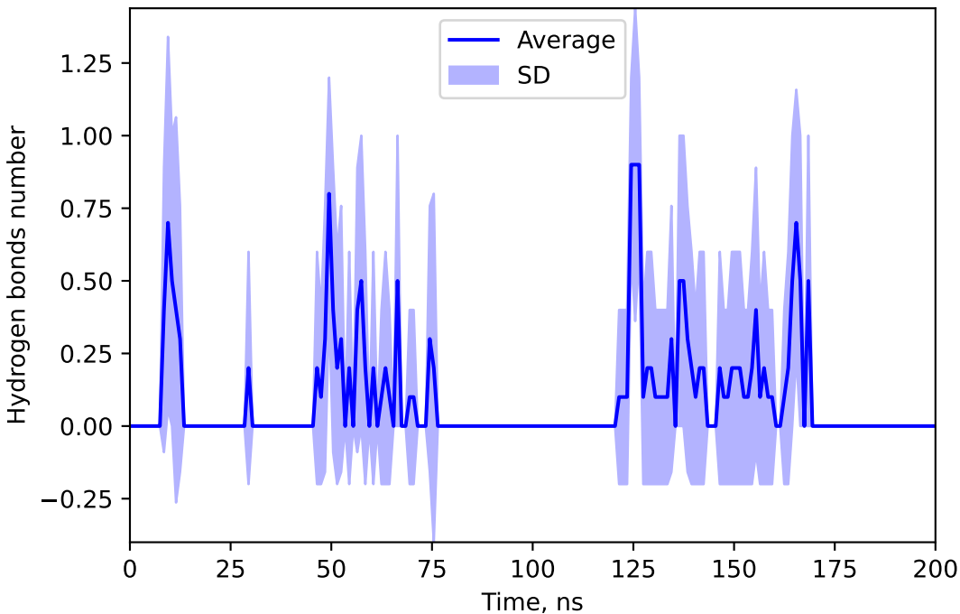
Hydrogen bonds number between 195797 and LYNC
