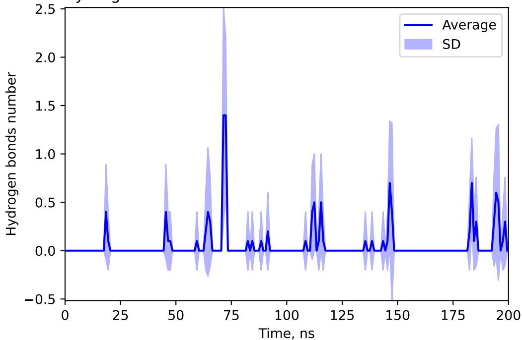
Hydrogen bonds number between 155521967 and LYNC
