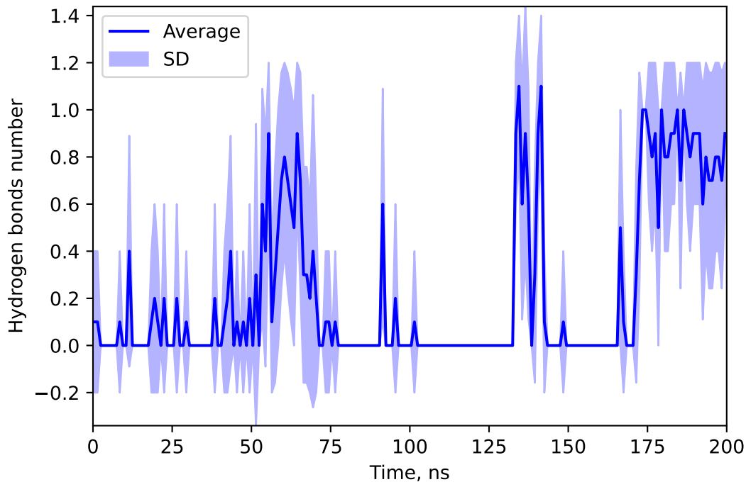
Hydrogen bonds number between 155559627 and DANO
