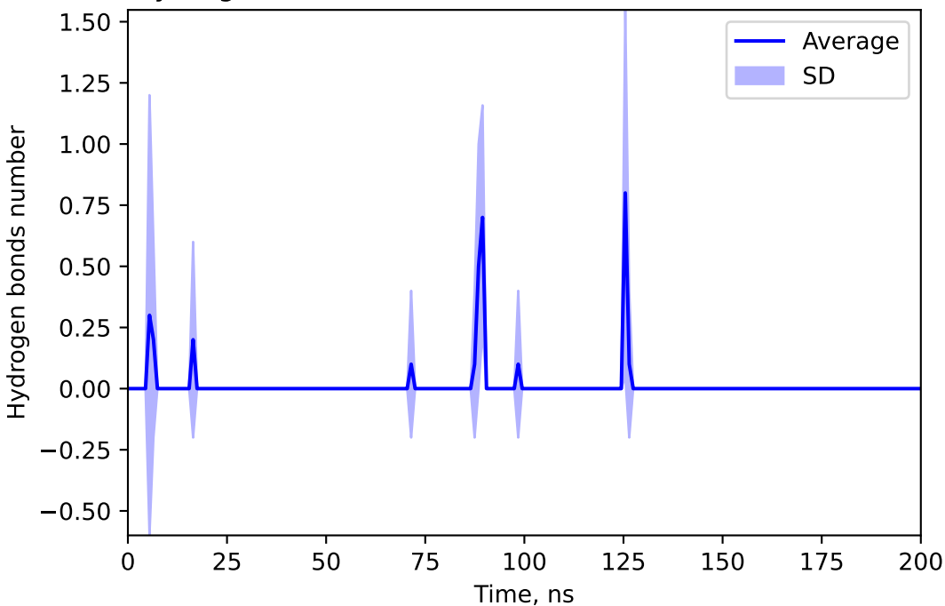
Hydrogen bonds number between 44575206 and RONI
