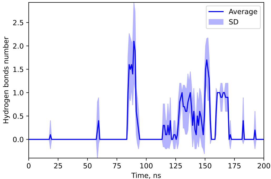
Hydrogen bonds number between 155557444 and SPIR
