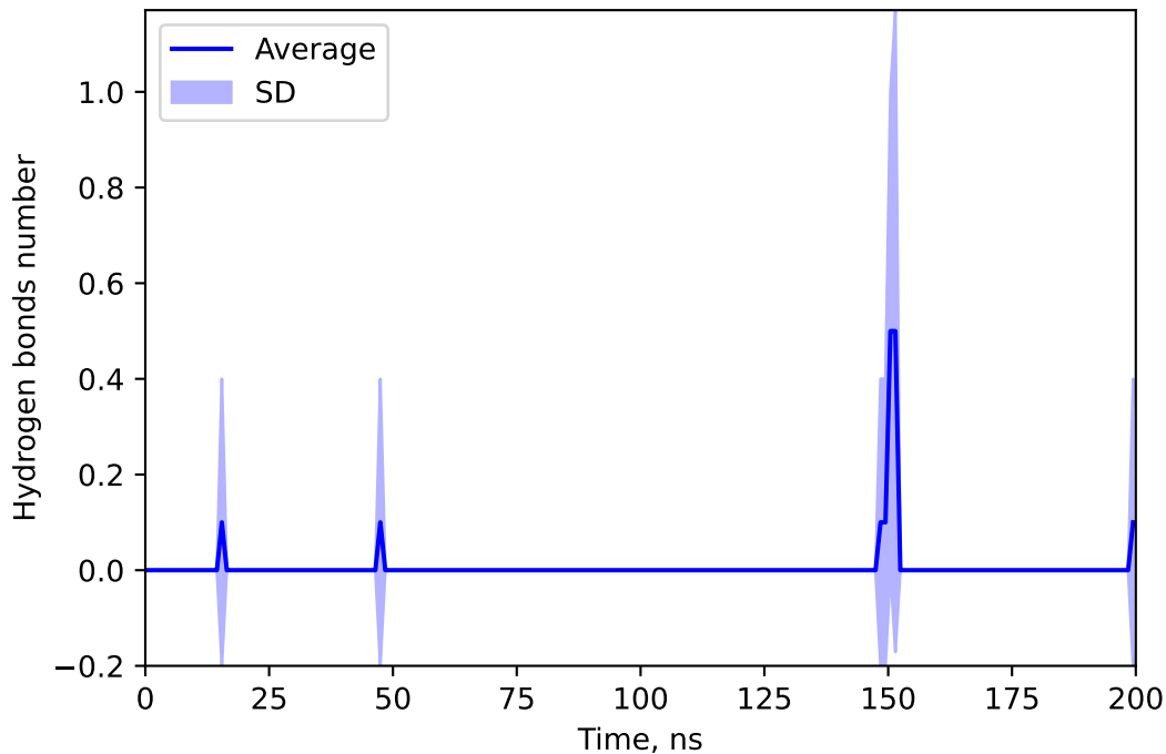
Hydrogen bonds number between 127034107 and LYNC
