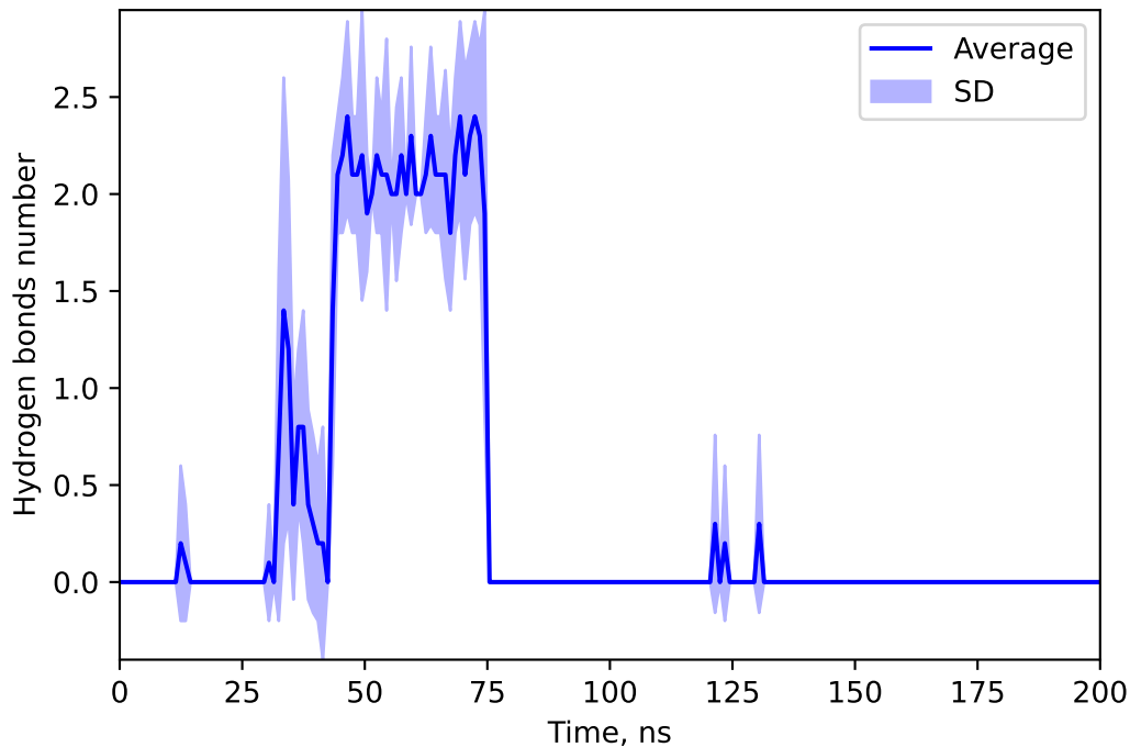
Hydrogen bonds number between 155514020 and STRE
