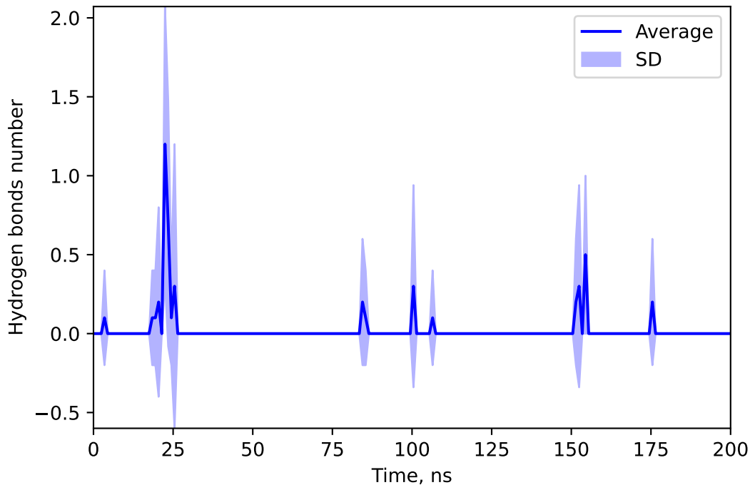
Hydrogen bonds number between 155518747 and METR
