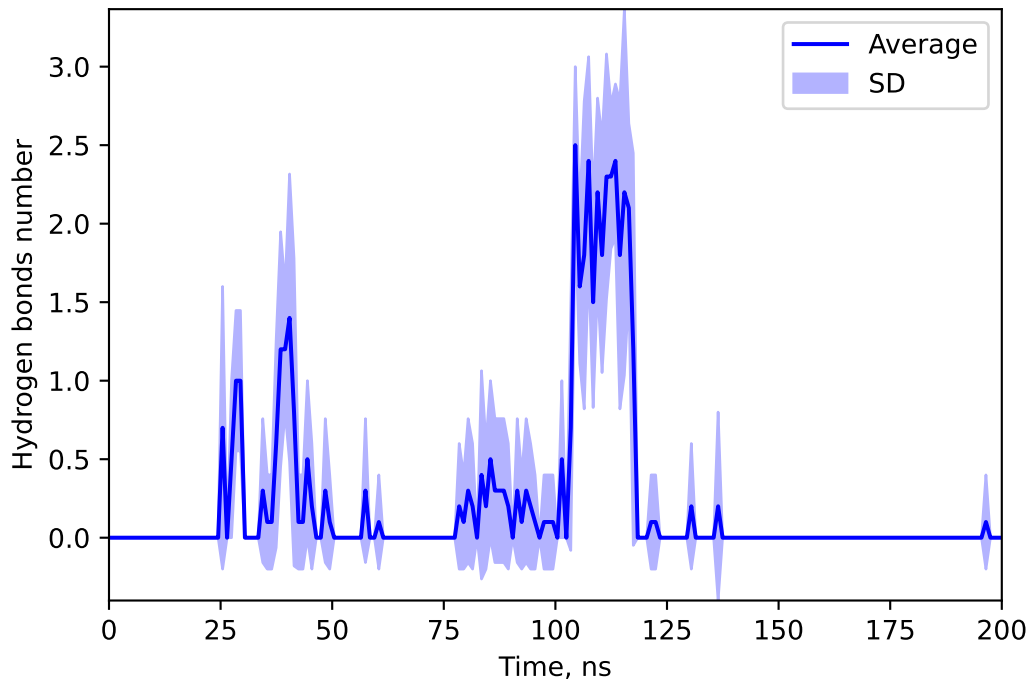
Hydrogen bonds number between 44569229 and DANO
