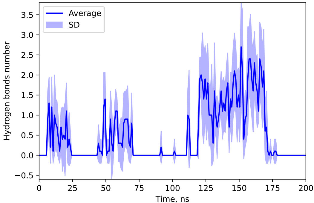
Hydrogen bonds number between 44569229 and CEFA
