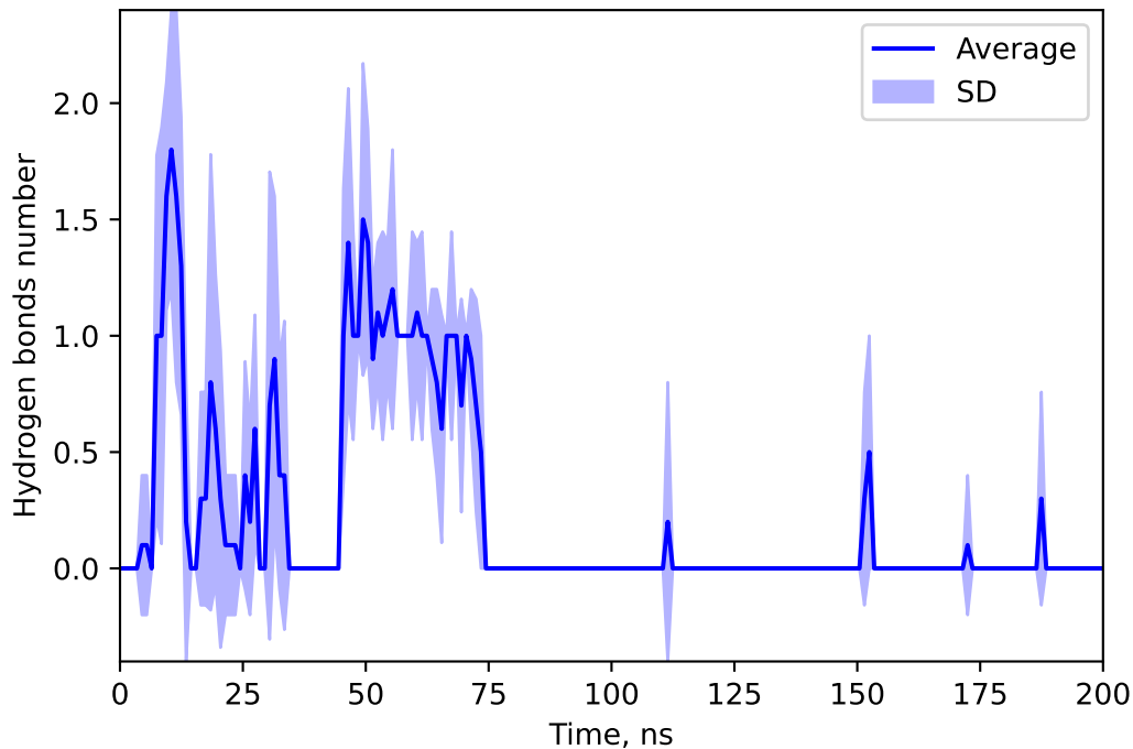
Hydrogen bonds number between 145975502 and SULF
