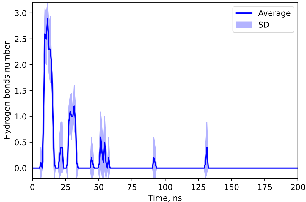
Hydrogen bonds number between 127034107 and TILM
