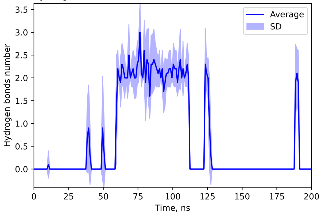
Hydrogen bonds number between 155557444 and STRE
