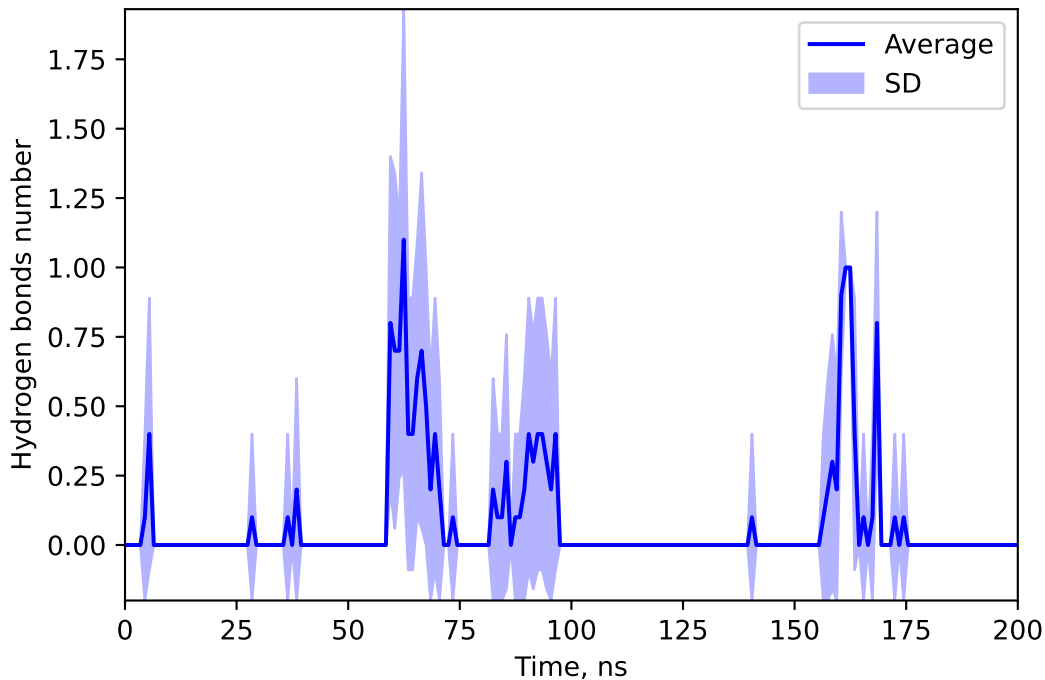
Hydrogen bonds number between 155514020 and TILM
