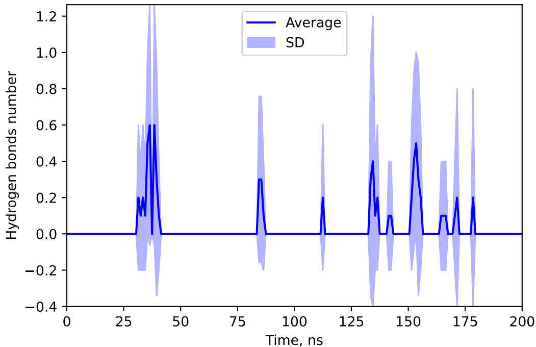
Hydrogen bonds number between 155557444 and METR
