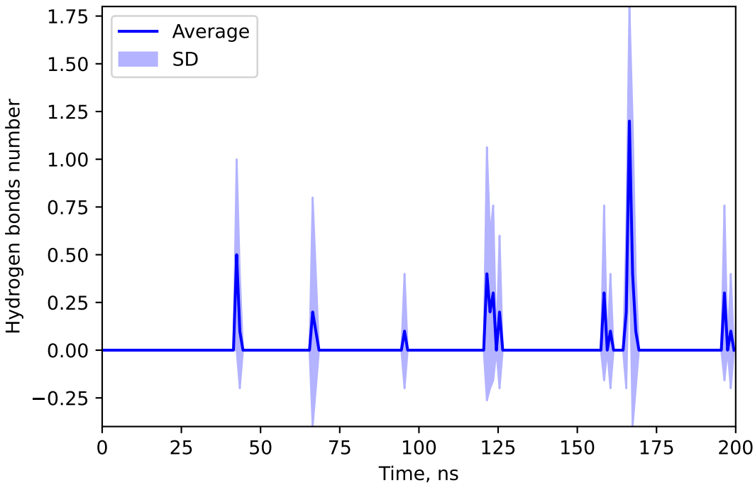
Hydrogen bonds number between 127034107 and RONI
