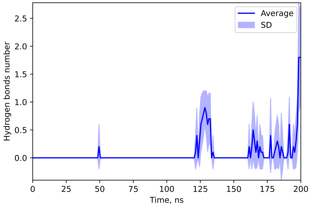
Hydrogen bonds number between 137646969 and DANO
