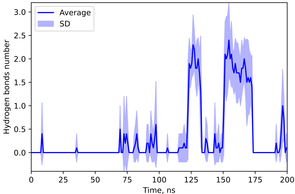
Hydrogen bonds number between 166625339 and SULF
