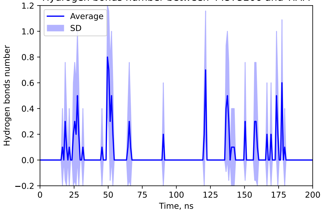
Hydrogen bonds number between 44575206 and TIAM
