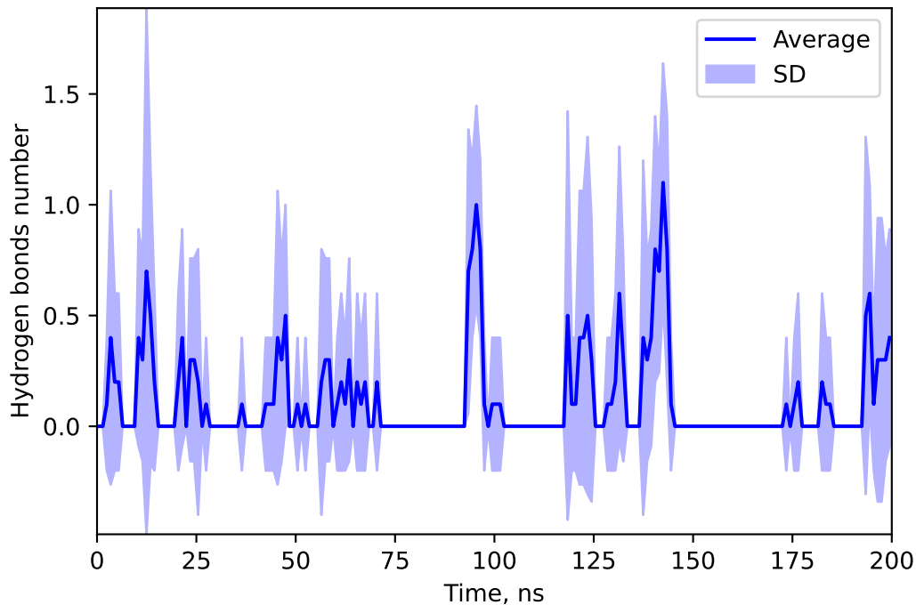
Hydrogen bonds number between 155557444 and DEME
