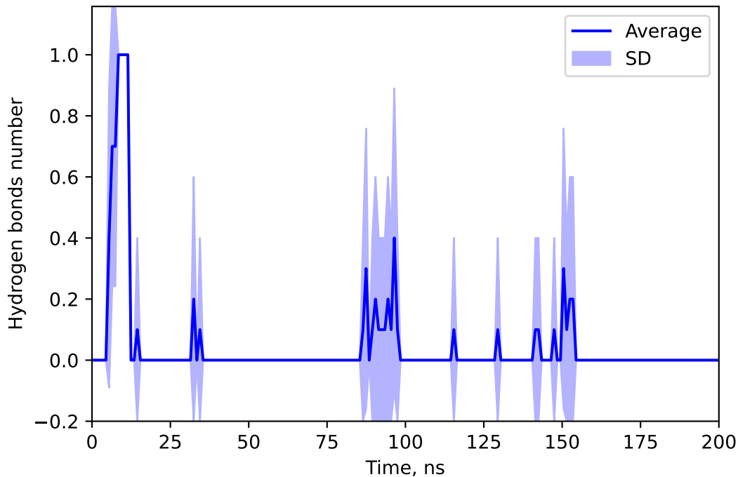
Hydrogen bonds number between 155514020 and TIAM
