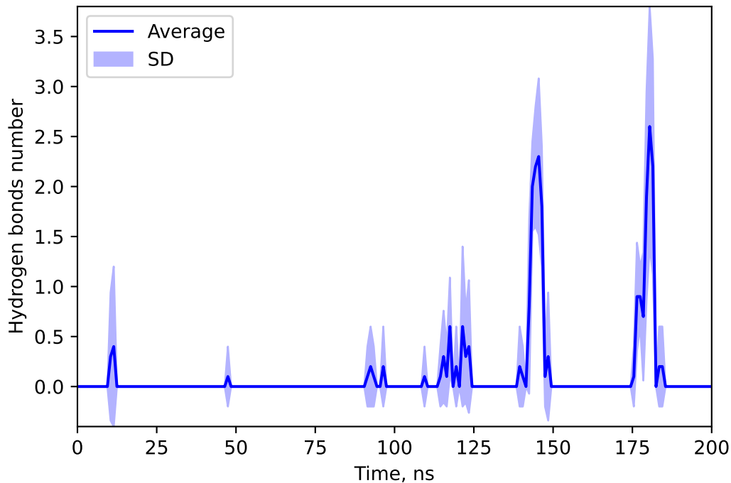
Hydrogen bonds number between 73293549 and LYNC
