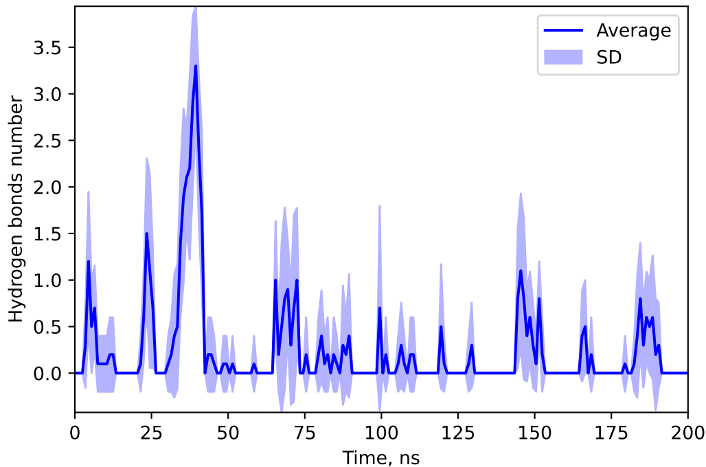
Hydrogen bonds number between 44569229 and SULF
