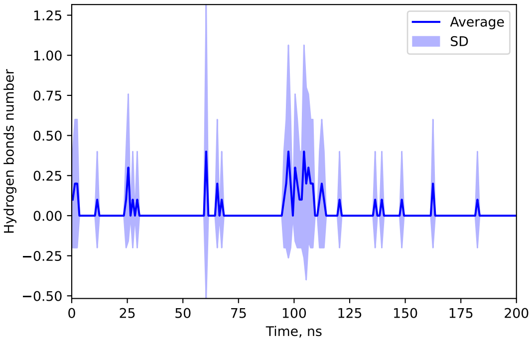
Hydrogen bonds number between 195797 and METR
