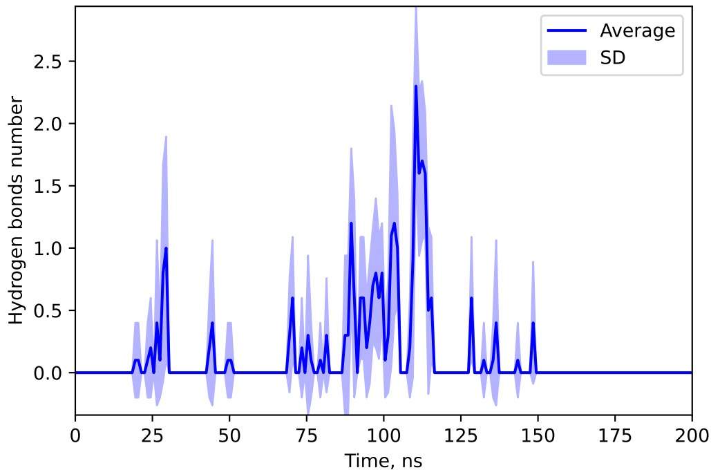
Hydrogen bonds number between 145975502 and TIAM
