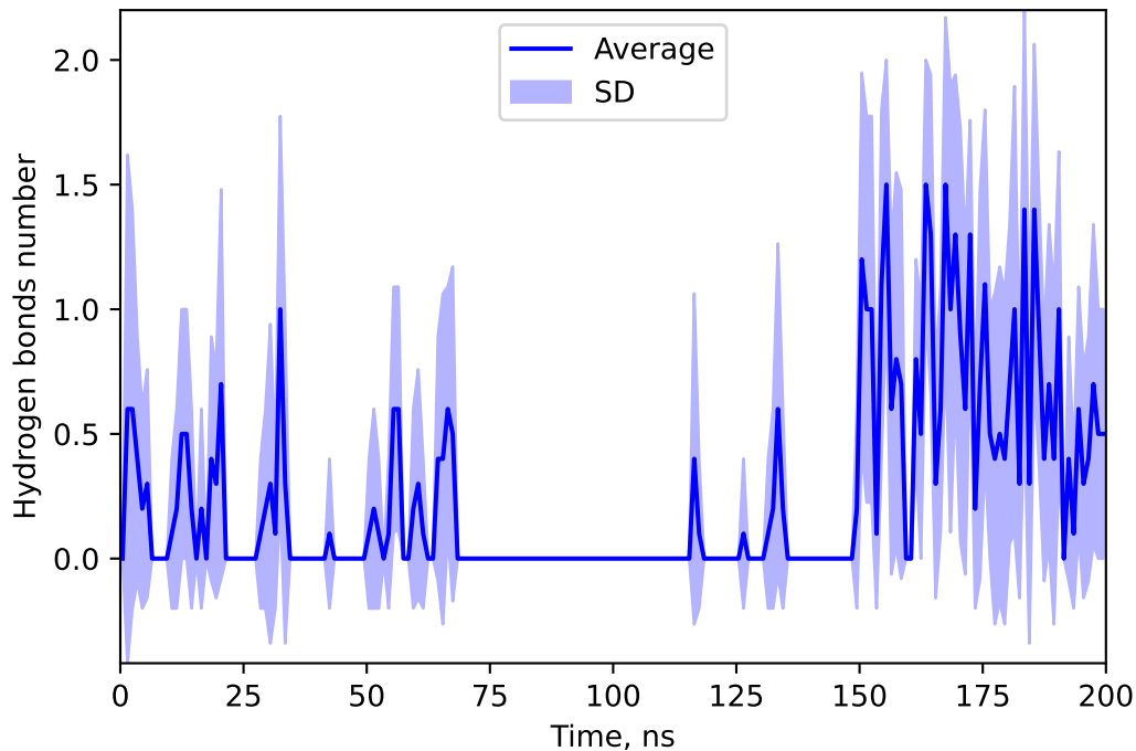
Hydrogen bonds number between 155557444 and DOXY
