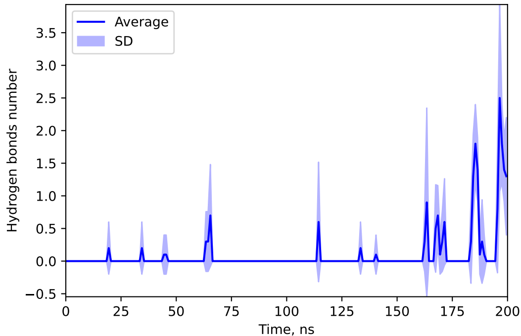
Hydrogen bonds number between 137644274 and RONI
