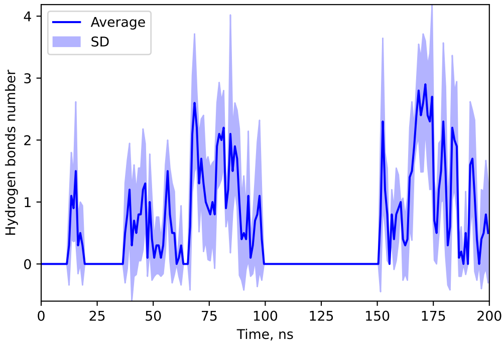
Hydrogen bonds number between 155518747 and CEFA
