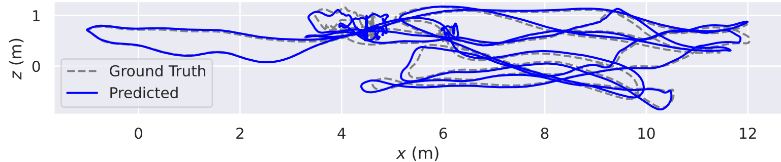
Euroc MH_03_medium Trial #1 (ATE: 11.571)
