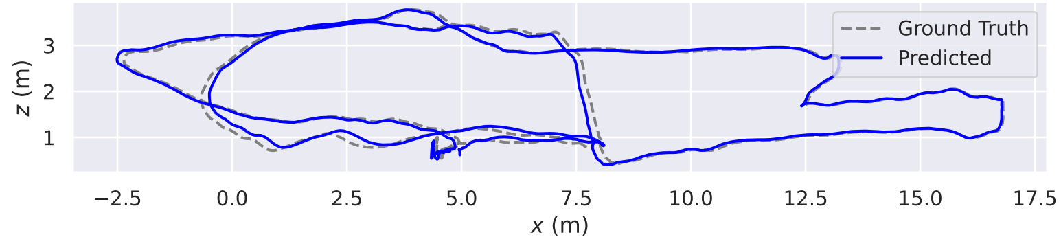
Euroc MH_05_difficult Trial #1 (ATE: 8.024)
